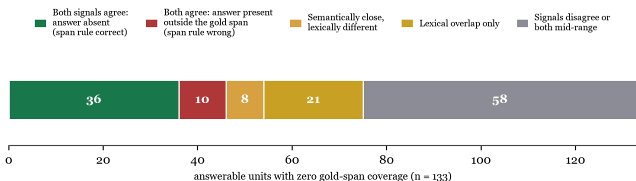
Figure 5. A lexical-only reading suggests 23.3% under-coverage; requiring both proxies to agree gives 7.5%. Neither is the answer — 65.4% is unresolved by any automated signal and needs human entailment judgement that has not been performed.
