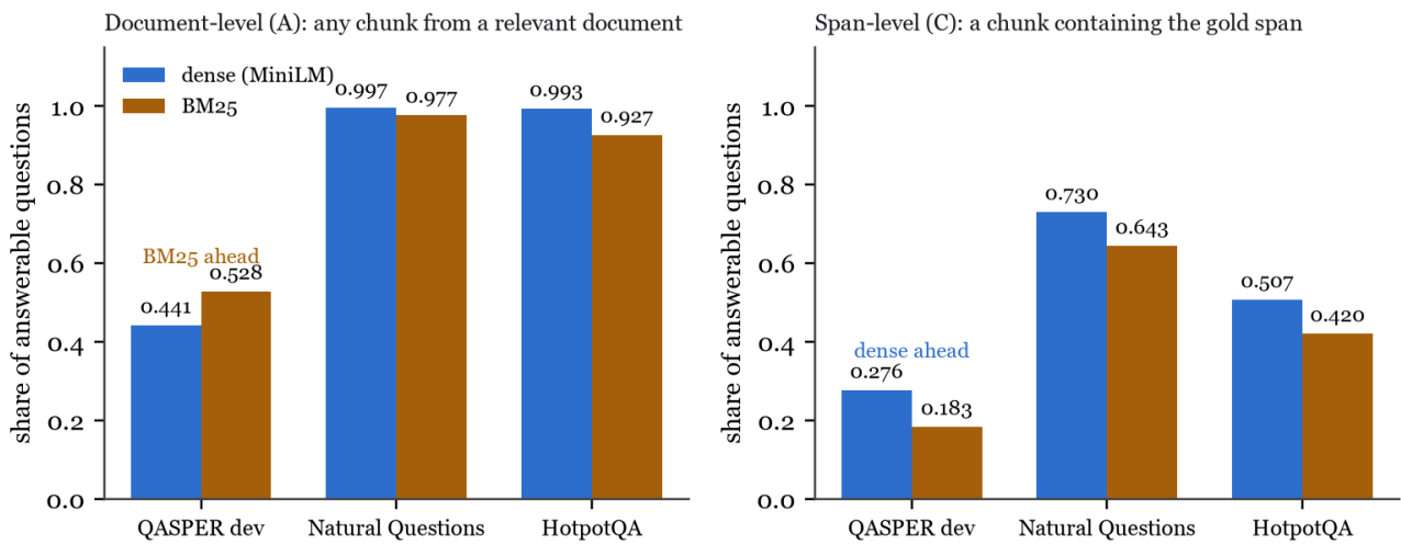
Figure 2. On QASPER the ranking inverts: a document-level evaluation recommends BM25, a span-level evaluation recommends the dense retriever, significantly. The inversion appears on one of three corpora, so the claim is that it is possible and was observed — not that it is general.
