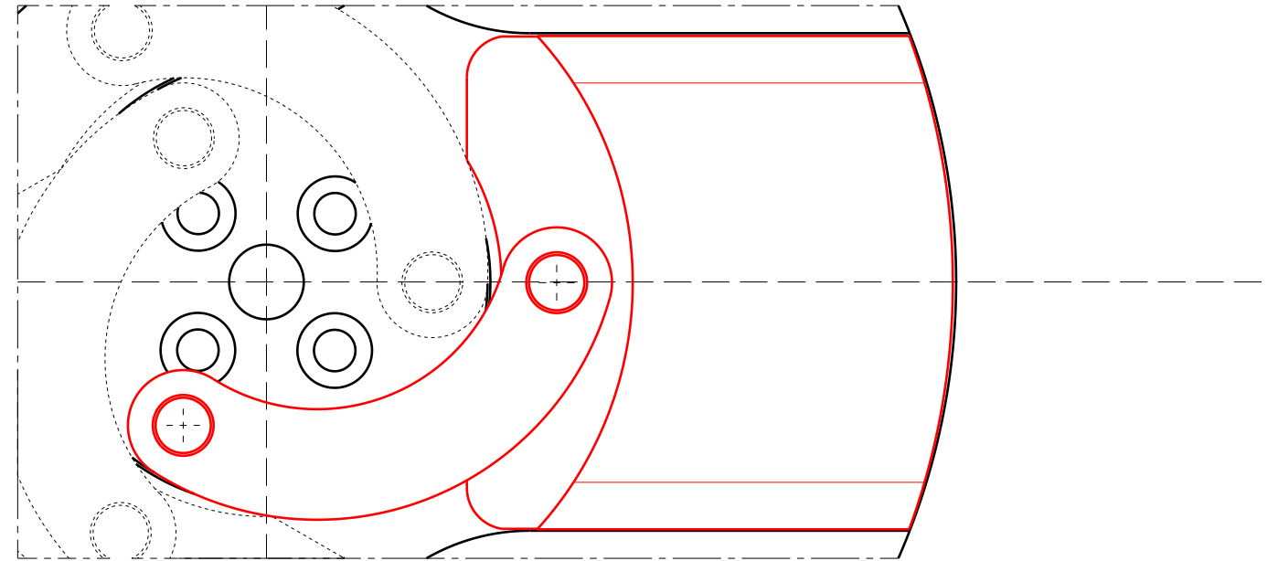
Detail A (closed) Scale: 2:1
