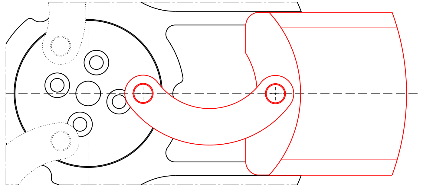
Detail A (opened) Scale: 2:1
