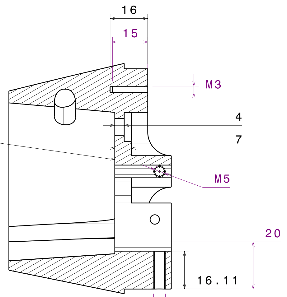
Section view E-E Scale: 1:1
