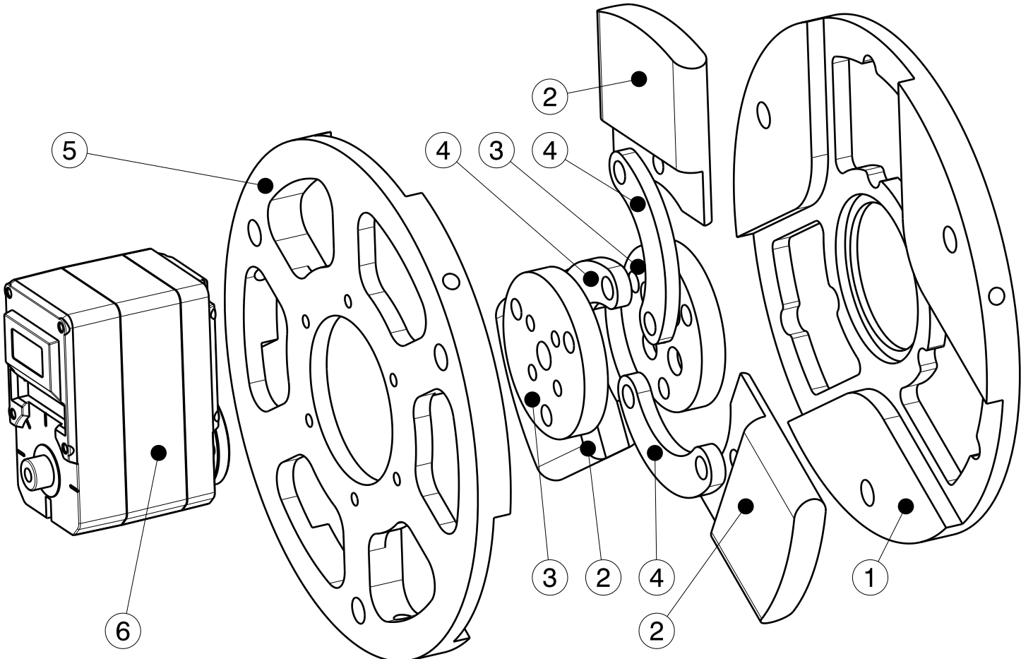
Exploded view Scale: 1:1
