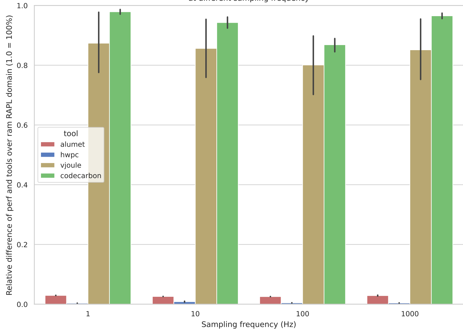
Relative difference of perf and tools over ram RAPL domain at different sampling frequency
