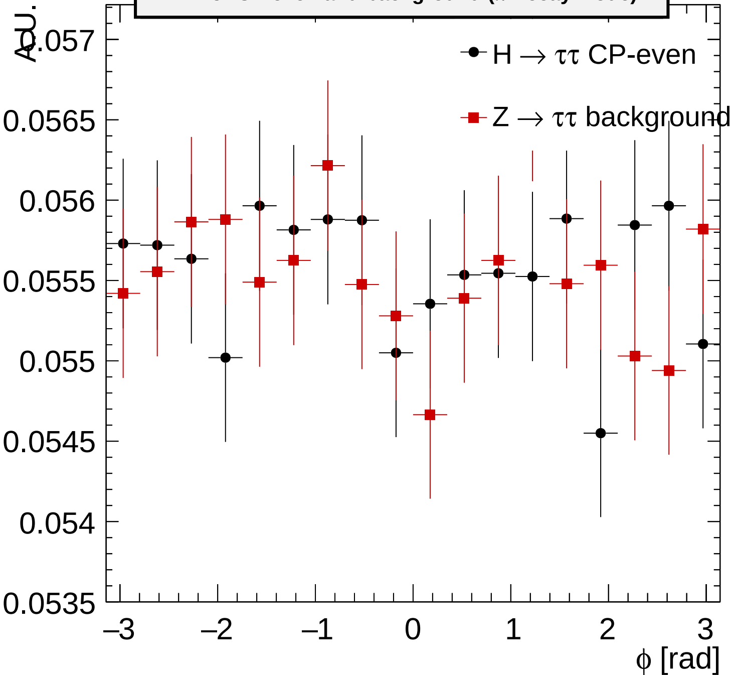
Phi for CP-even and background ( \pi Decay Mode)
