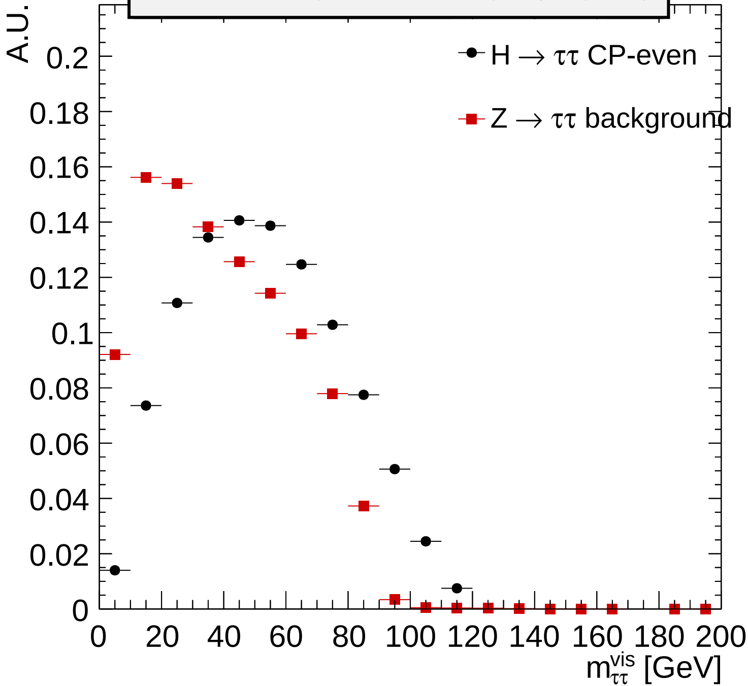
Visible Mass of the Di-tau System for CP-even and background ( \pi Decay Product)
