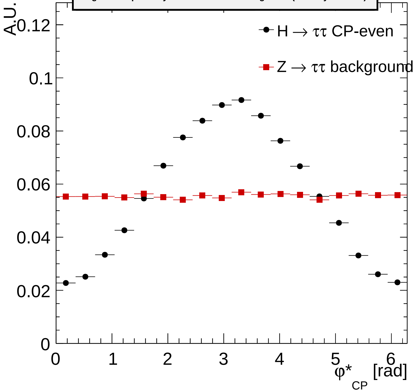
Signed Acoplanarity for CP-even and background ( \pi Decay Product)
