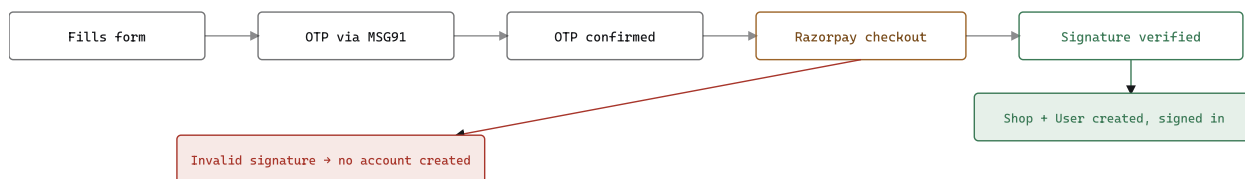
Fig. 2 – End-to-end shop creation, from the registration form to a working login.
