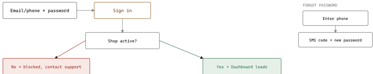
Fig. 1 – The sign-in decision path, including the shop-suspension check and the separate forgot-password recovery path.
