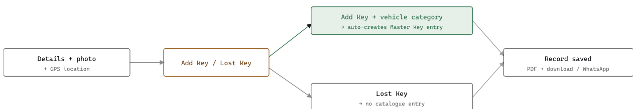
Fig. 3 – The Master Key auto-create is guarded behind both the Add Key flag and a recognised vehicle category.
