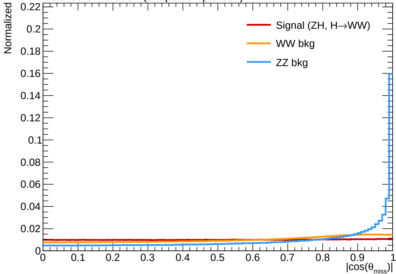
FCC-ee Simulation (shape comparison)
