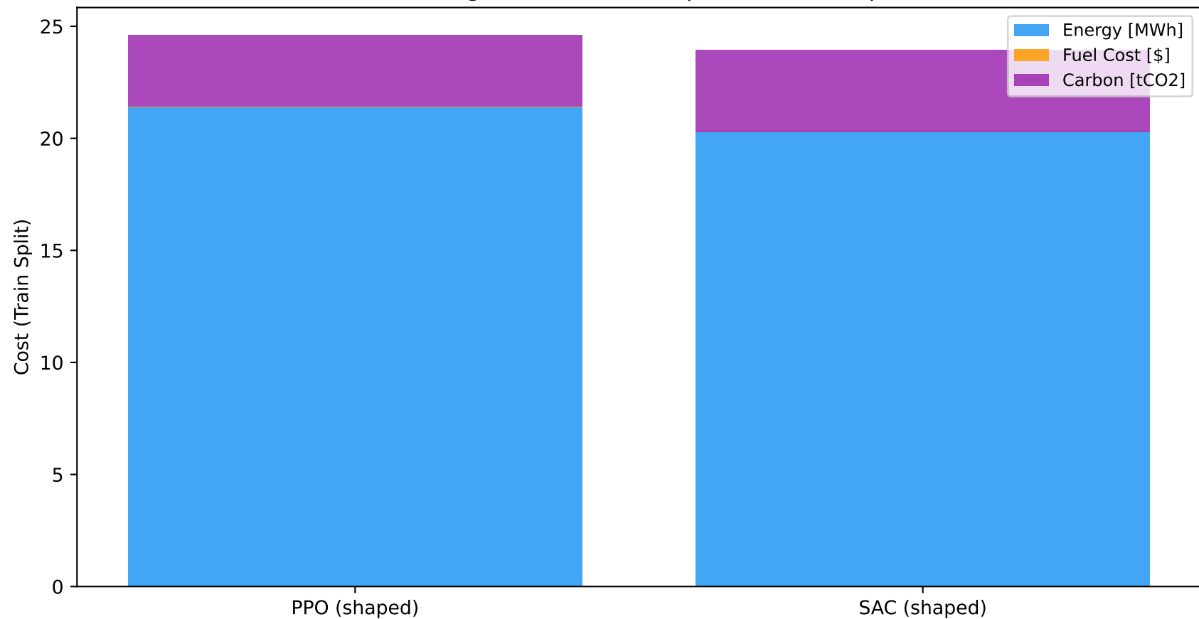
DC Microgrid — Cost Decomposition (Train Split)
