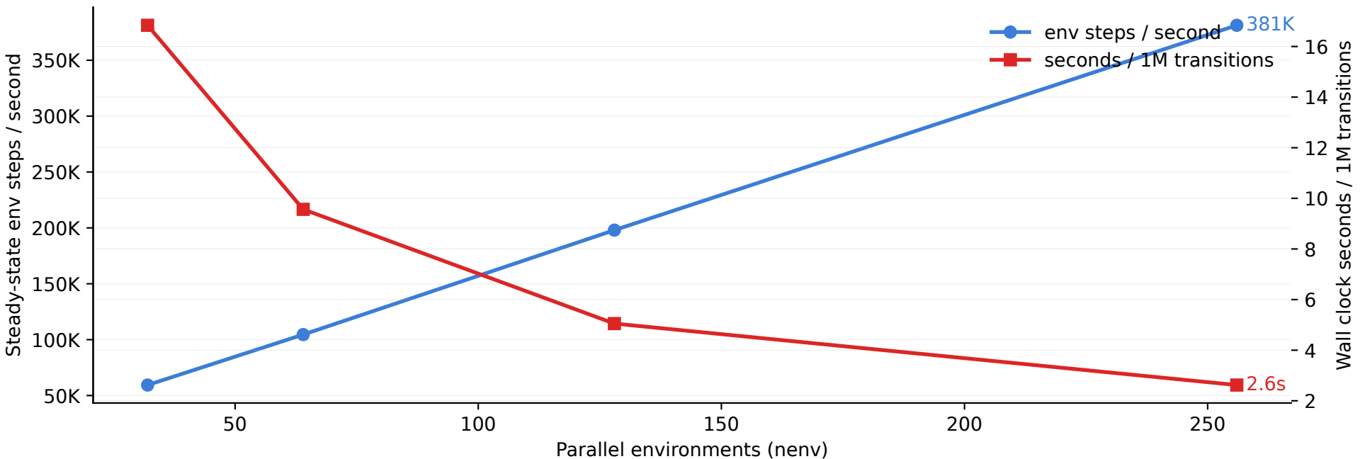
DC Microgrid JAX-only extended scaling
