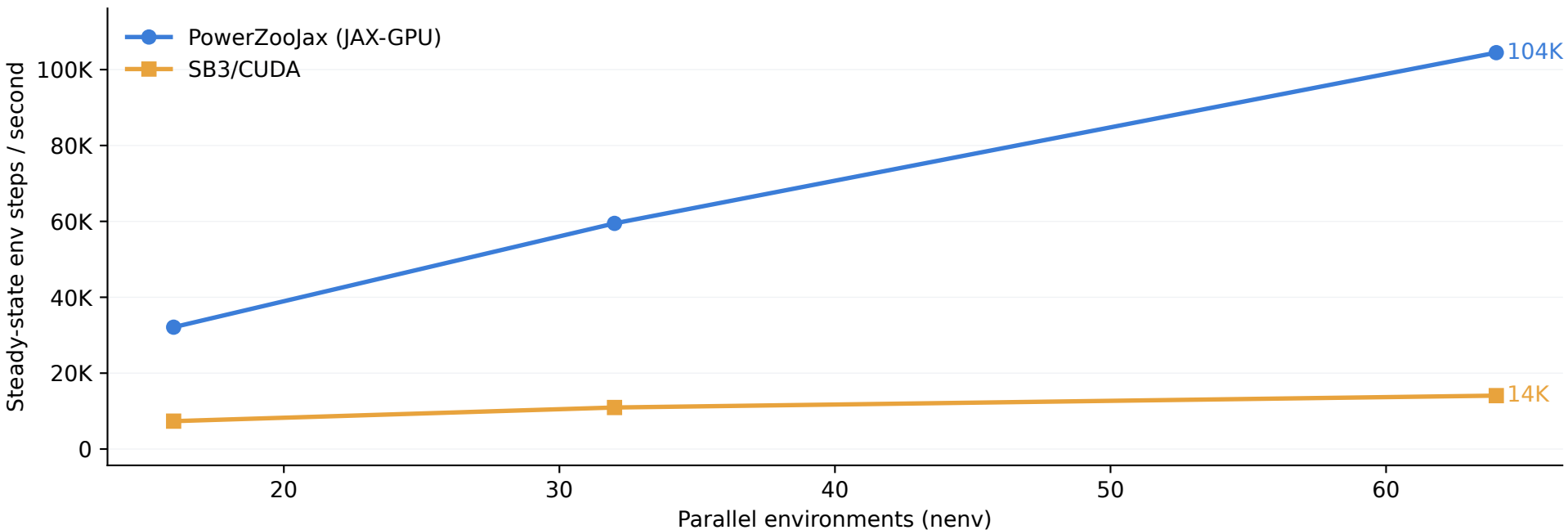
DC Microgrid matched-range execution scaling
