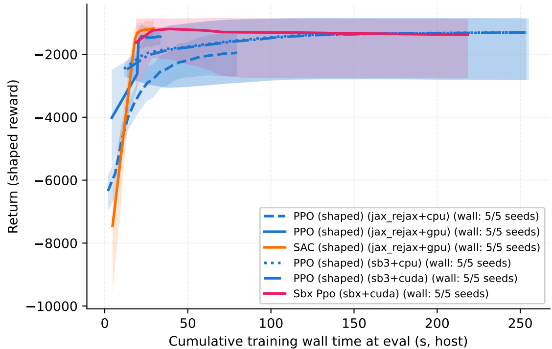
Eval return vs wall time (cross-backend/device comparison)
