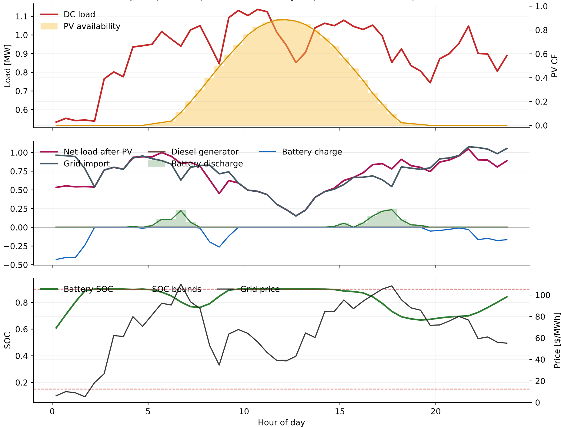
JAX/ReJAX SAC representative DC Microgrid episode (in-distribution, ep=5)
