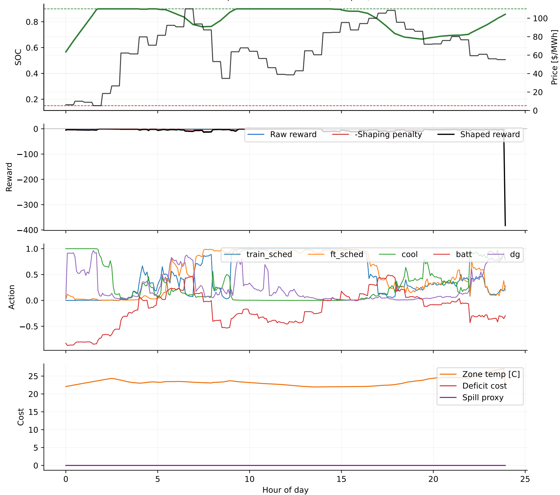
SAC representative mechanism (iid, ep=5)
