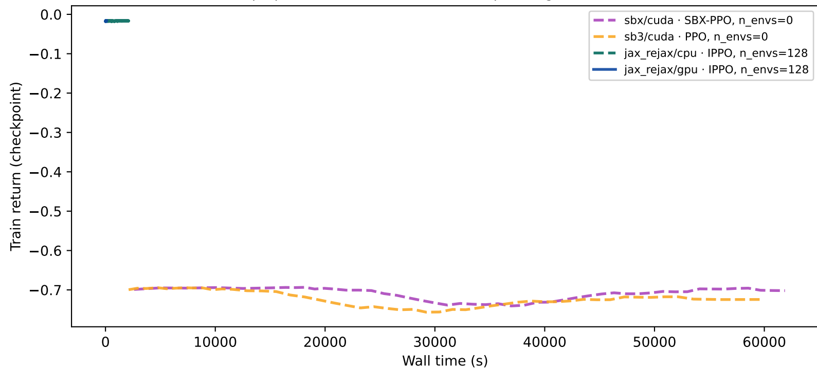
DERs — Cross-backend learning vs wall time (seed=0) All backends trained on the canonical train split (proportional wall time where checkpoint logs are absent)
