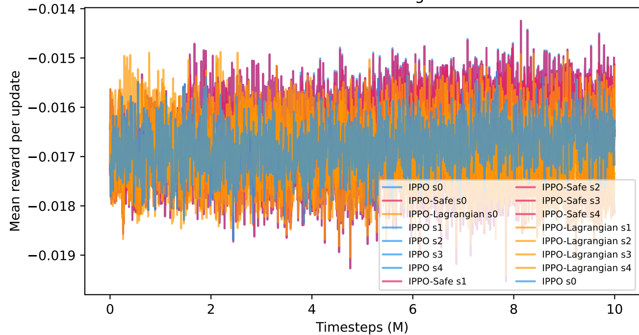
DERs — MARL Learning Curves
