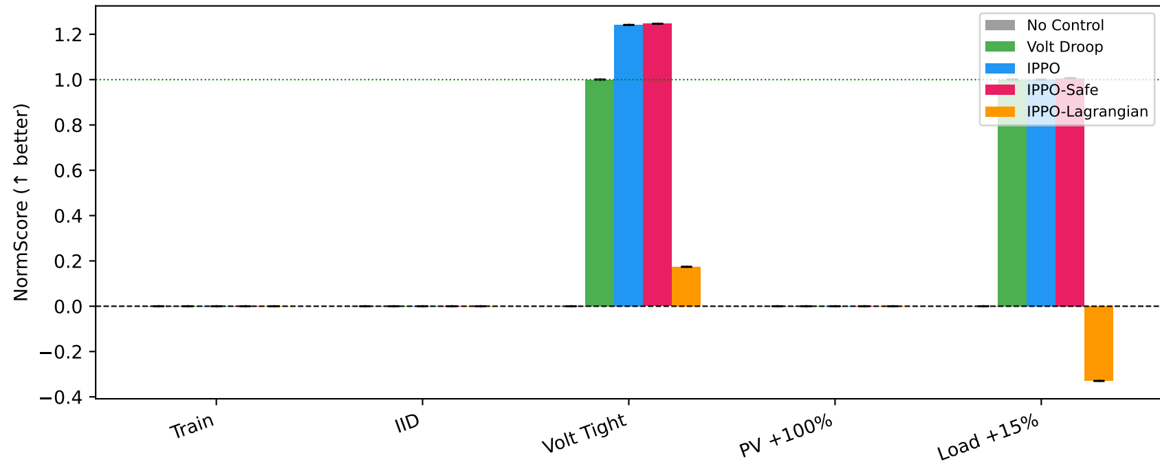
DERs — NormScore by Algorithm and Split
