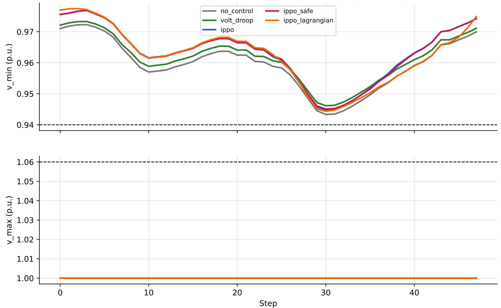
DERs Phase-1 — representative IID episode voltage envelope
