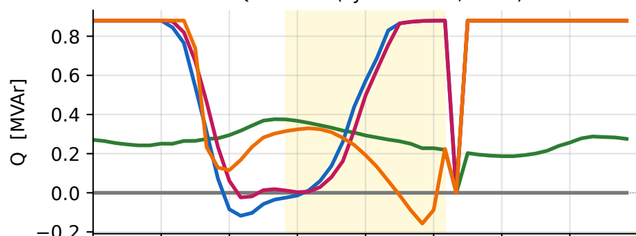
PV Q realized (system total, MVar)
