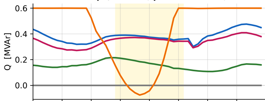
PV Q realized (system total, MVar)
