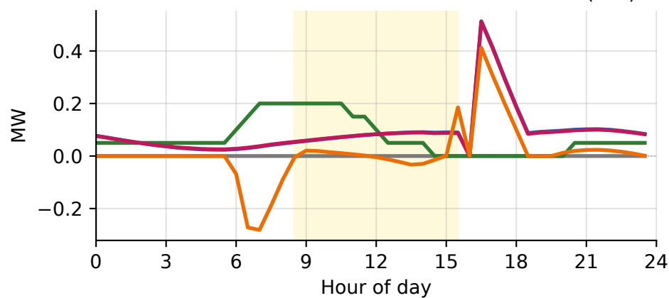
Flex net load relief = curtail + shift-out – shift-in (MW)
