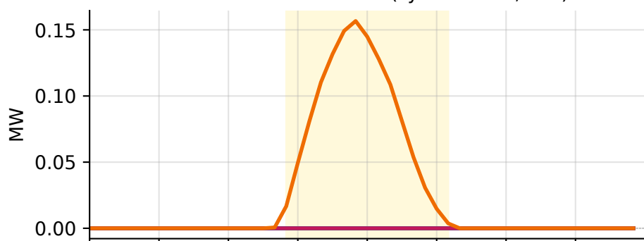
PV curtailment realized (system total, MW)
