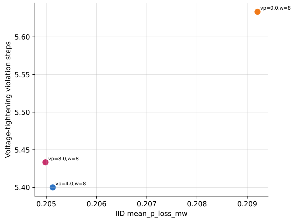
Sweep trade-off
