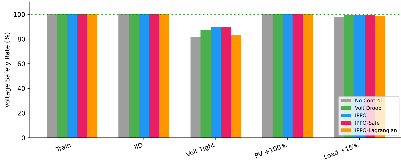
DERs — Fraction of Steps with All Voltages in Bounds
