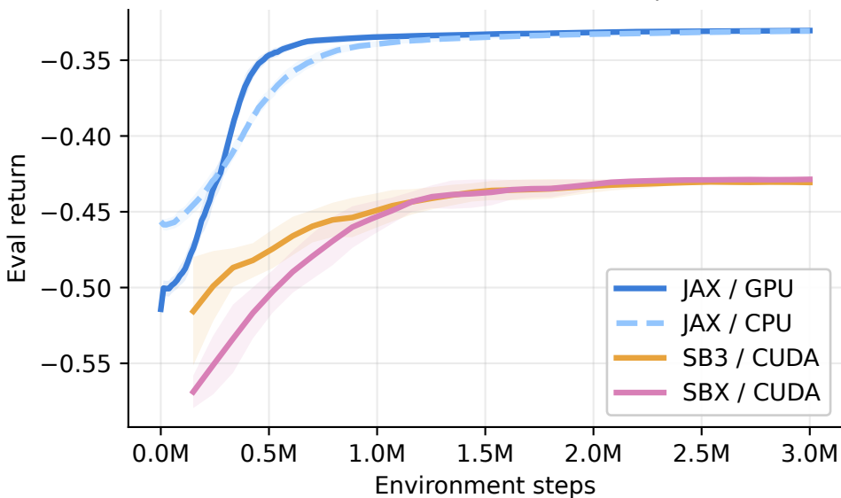
Eval return vs environment steps
