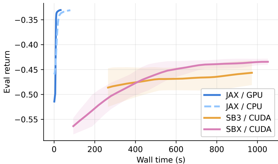
Eval return vs wall time
