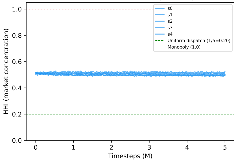
IPPO — Market HHI during Training
