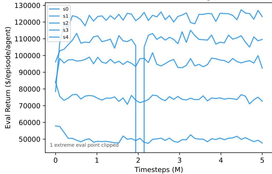
IPPO — Eval Return (mean/agent)
