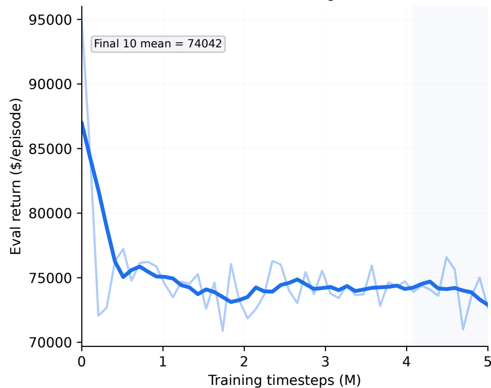
Eval return convergence
