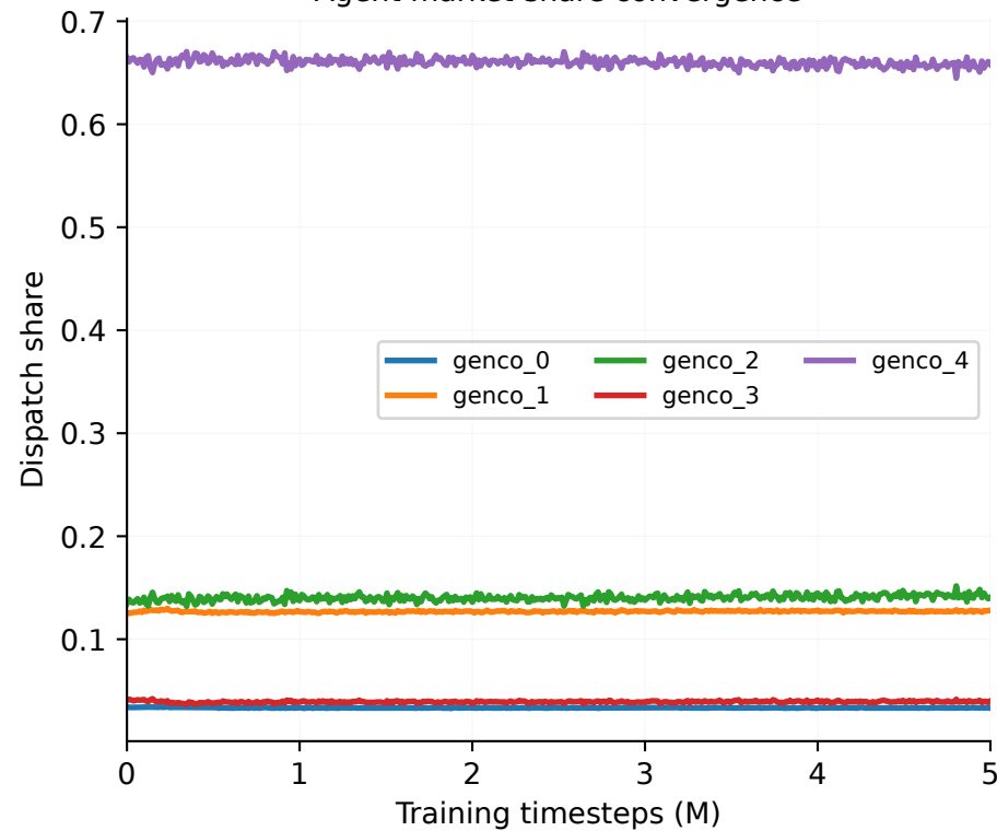
Agent market-share convergence
