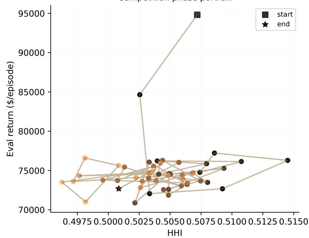
Competition phase portrait
