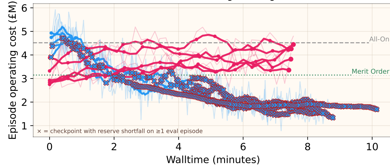
Eval Cost During Training
