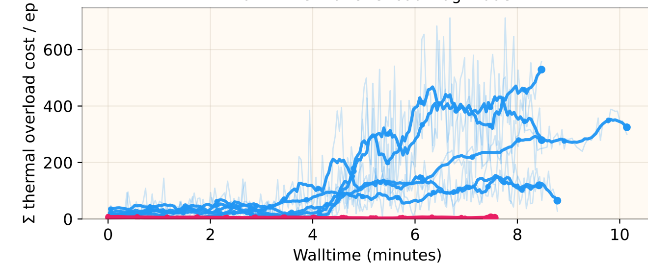
Eval — Thermal Overload Magnitude
