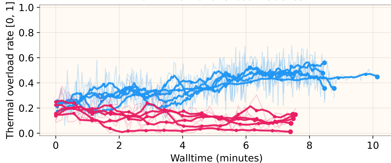
Eval — Thermal Overload Incidence
