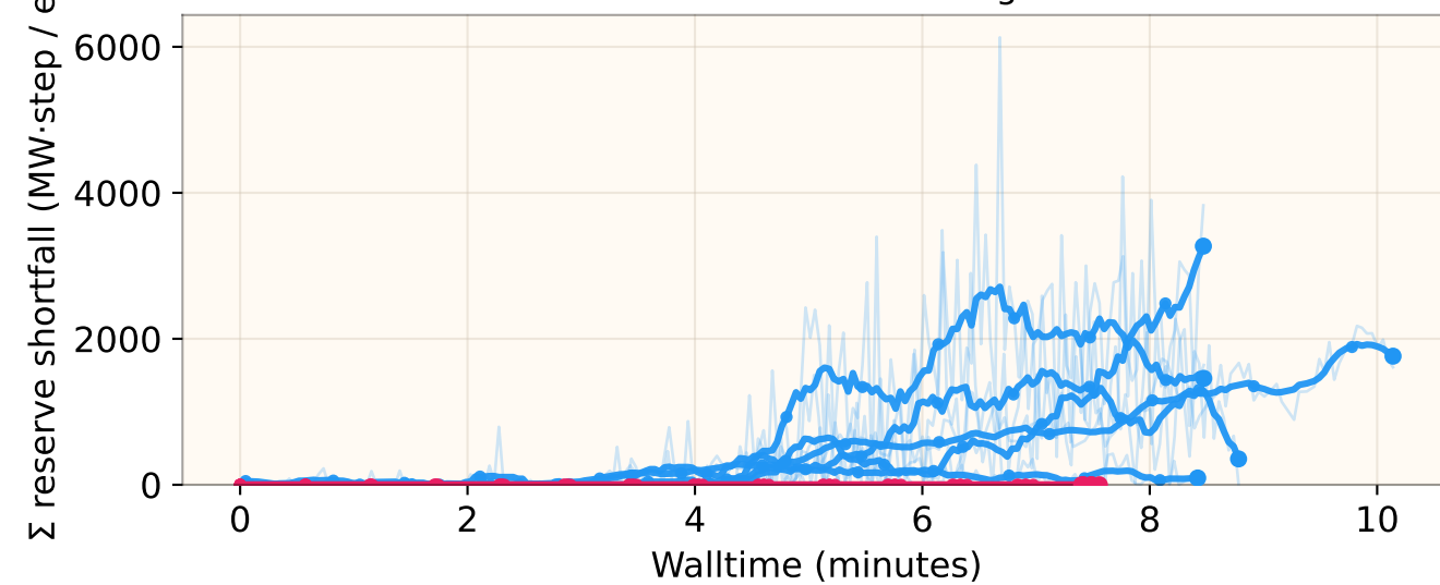
Eval — Reserve Shortfall Magnitude
