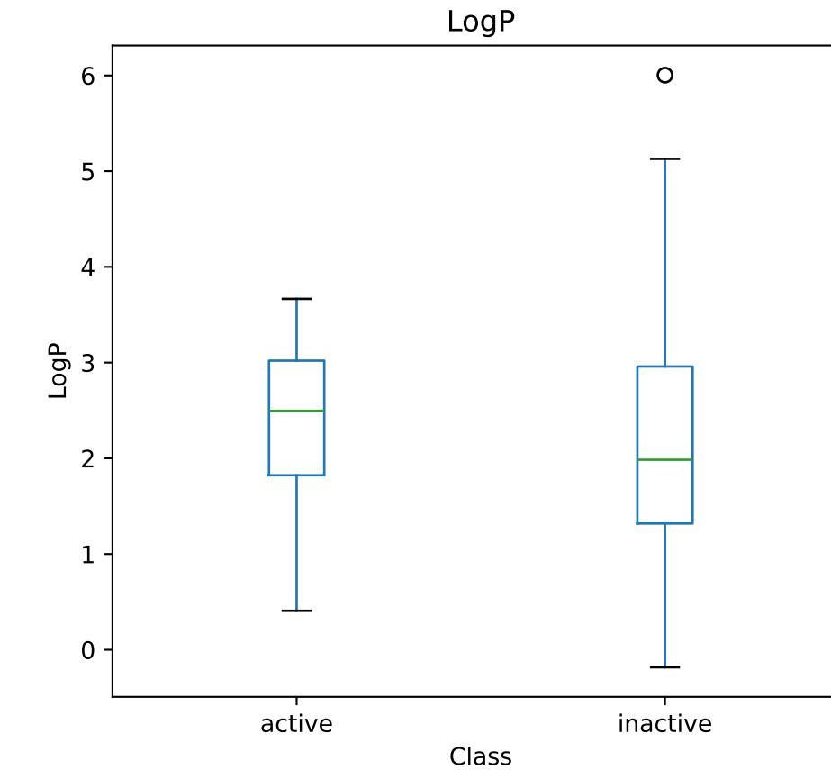
Property distribution by activity class
