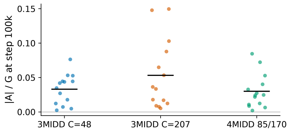
F Common-support normalized endpoints
