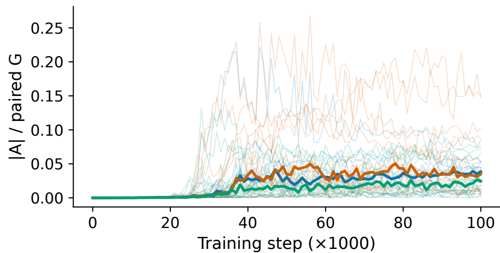
F Common-support normalized endpoints
