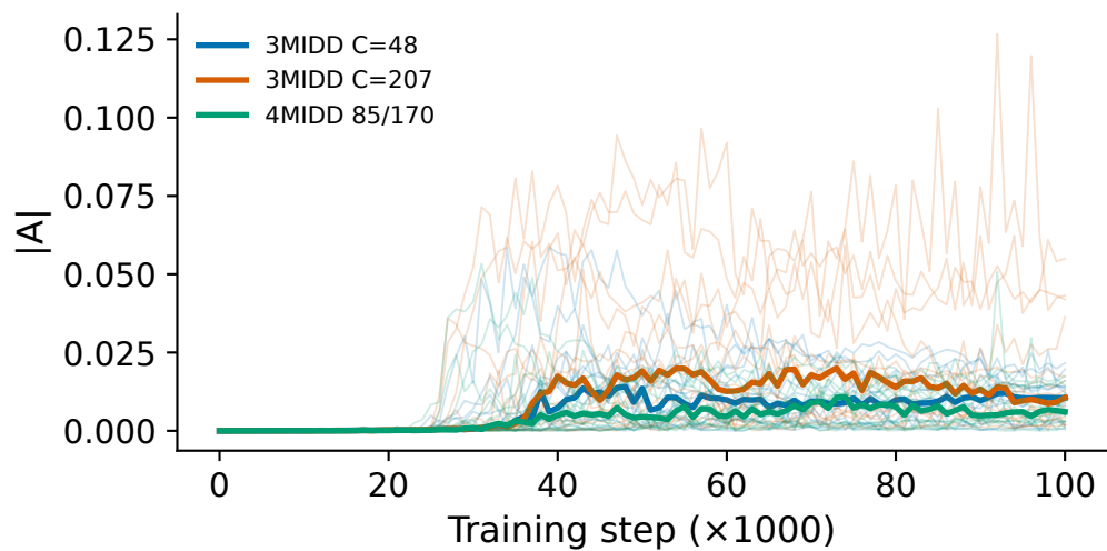
E Fixed-phase sign tendencies, N=14
