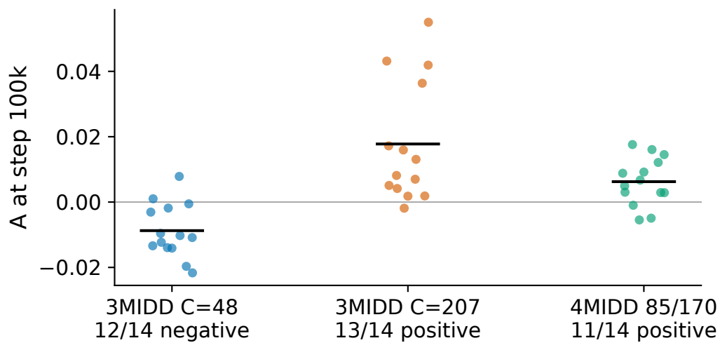
E Fixed-phase sign tendencies, N=14
