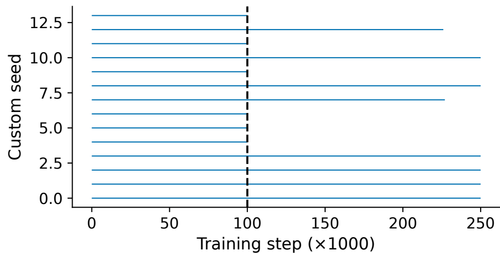
C Raw magnitude, common N=14
