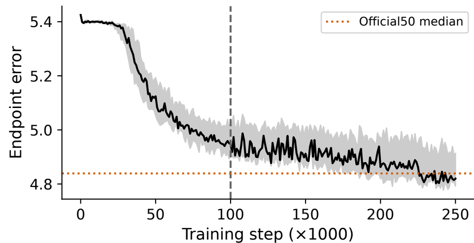
D Magnitude-normalized trajectories
