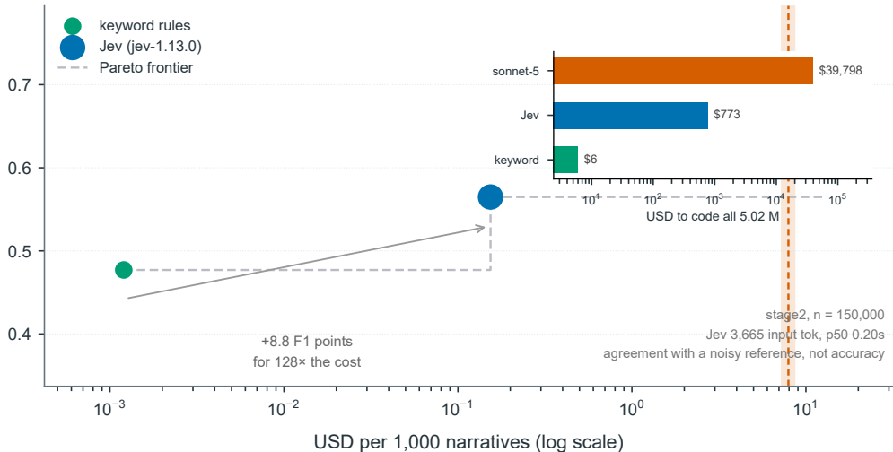
Cost-accuracy frontier; marker area \propto median latency
