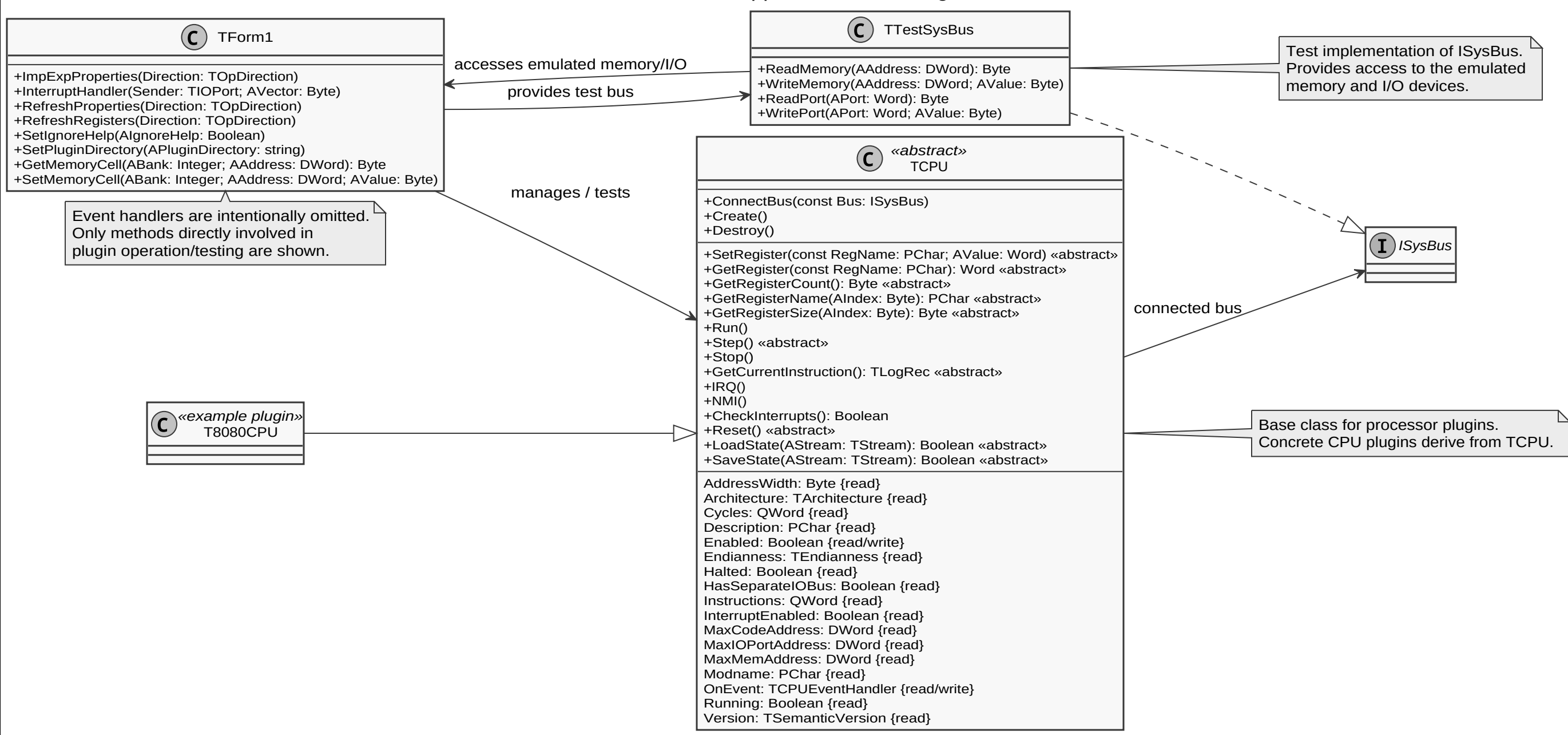
CLProcessor application class diagram
