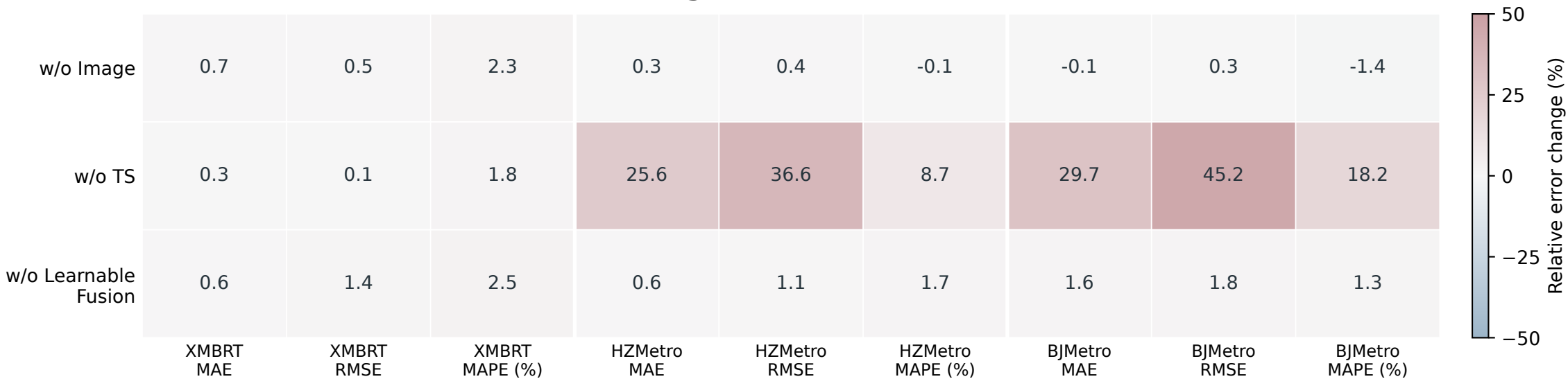
Relative error change of ablation variants vs. CWT-TSI
