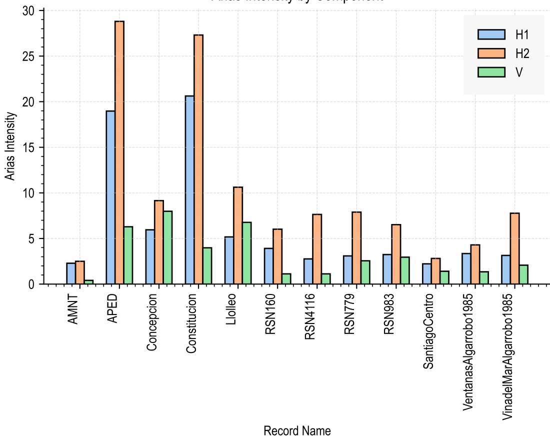
Arias Intensity by Component
