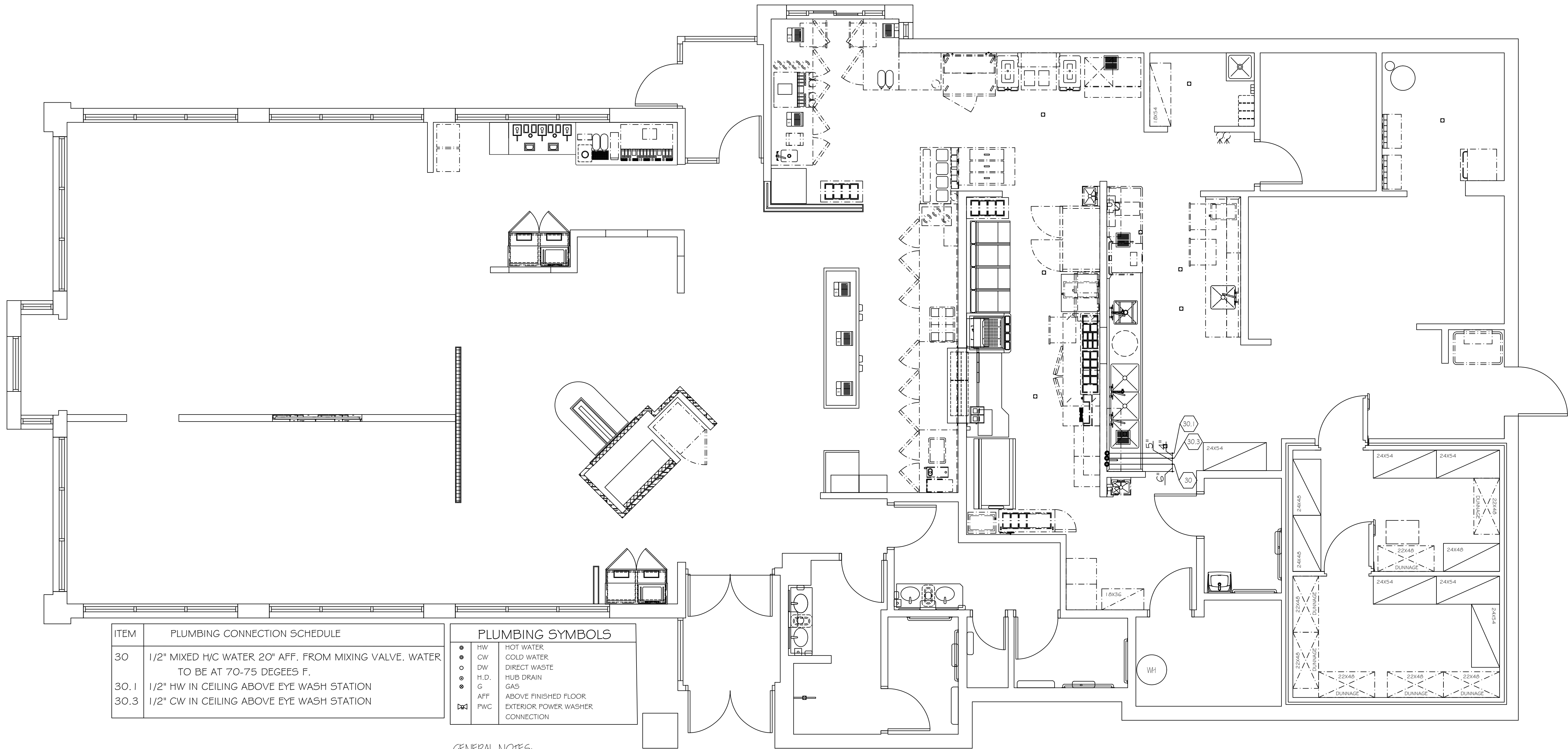
FOODSERVICE PLUMBING PLAN - CULVER'S OF SHAKOPEE, MN #0131 SCALE: 1/4" = 1'-0"
