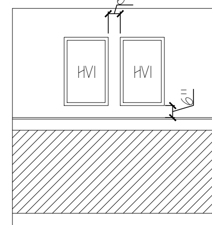
3 ELEV. - HEART OF FRESHNESS TYP. SCALE: 1/4" = 1'-0"
