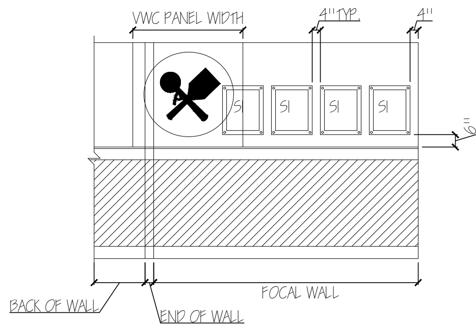
1 ELEV. - STANDARD STORY WALL & DINING MURAL VWC SCALE: 1/4" = 1'-0"
