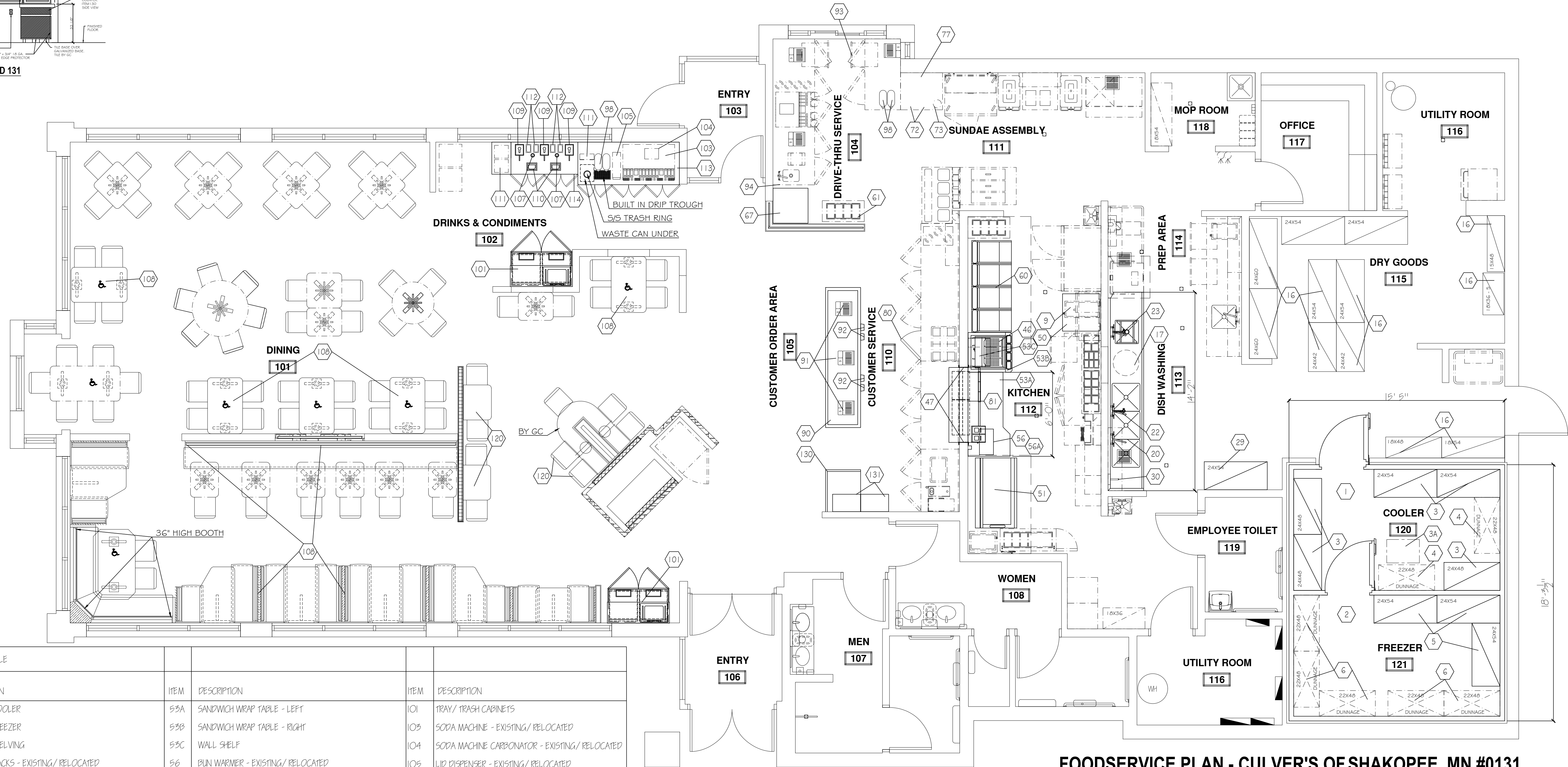
FOODSERVICE PLAN - CULVER'S OF SHAKOPEE, MN #0131 SCALE: 1/8" = 1'-0"
