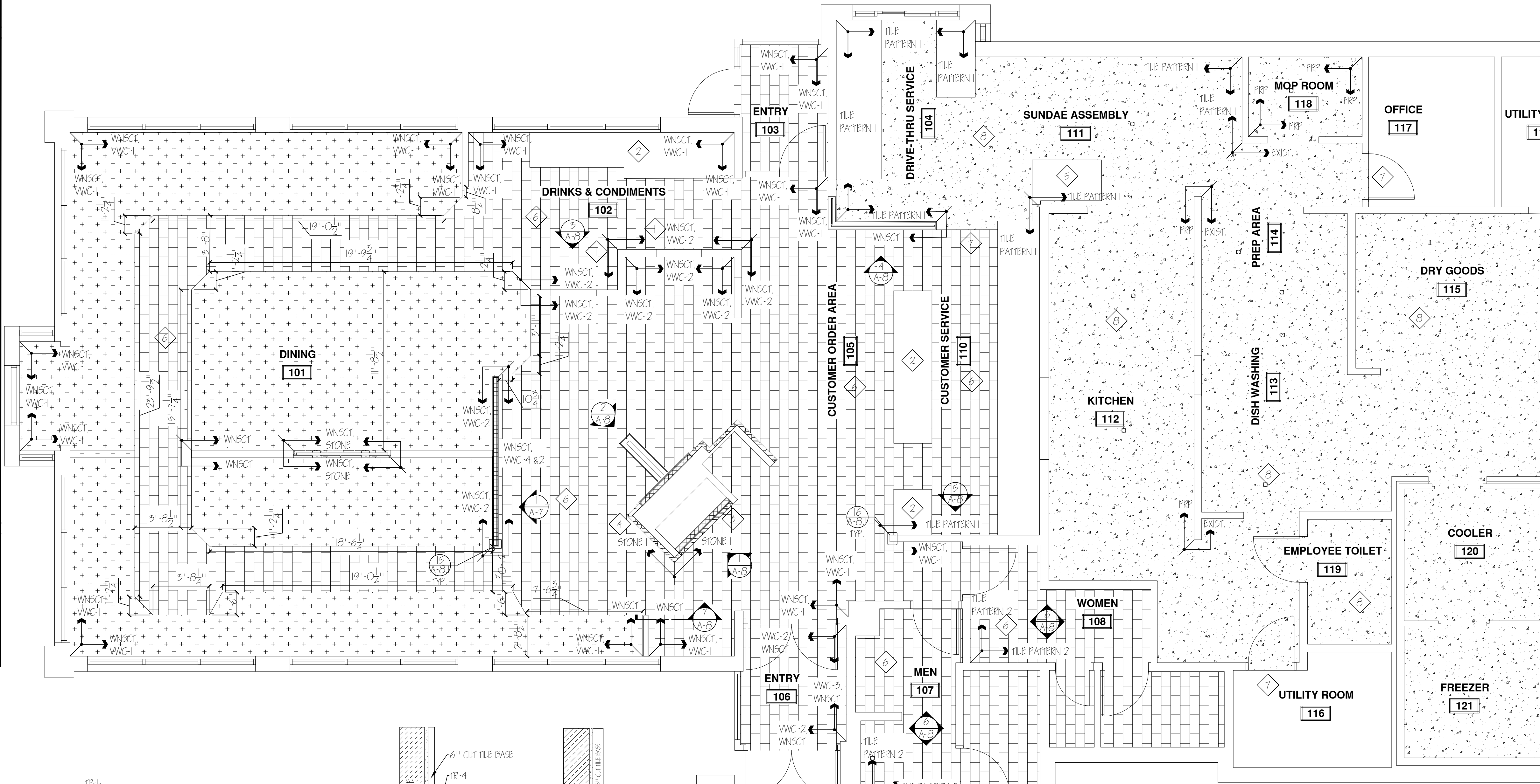
FINISH PLAN - CULVER'S OF SHAKOPEE, MN #0131 SCALE: 1/4" = 1'-0"
