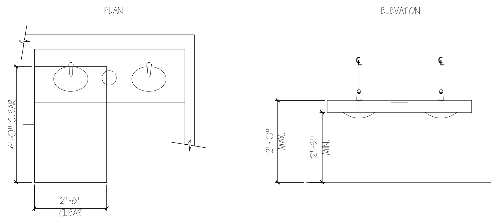
2 ADA LAVATORY CLEARANCES TYP. A-9 SCALE: 1/2" = 1'-0"
