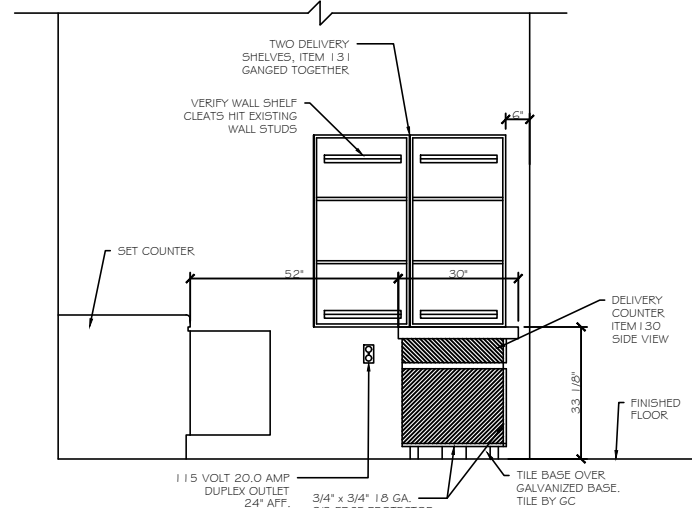
1 ELEV. - ITEM 130 AND 131 FS-1 SCALE: 1/4" = 1'-0"
