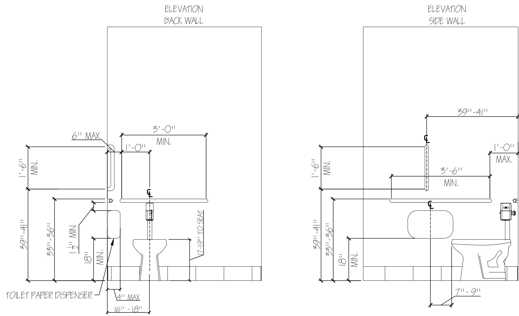
1 ADA TOILET STALL CLEARANCES TYP. A-9 SCALE: 1/2" = 1'-0"
