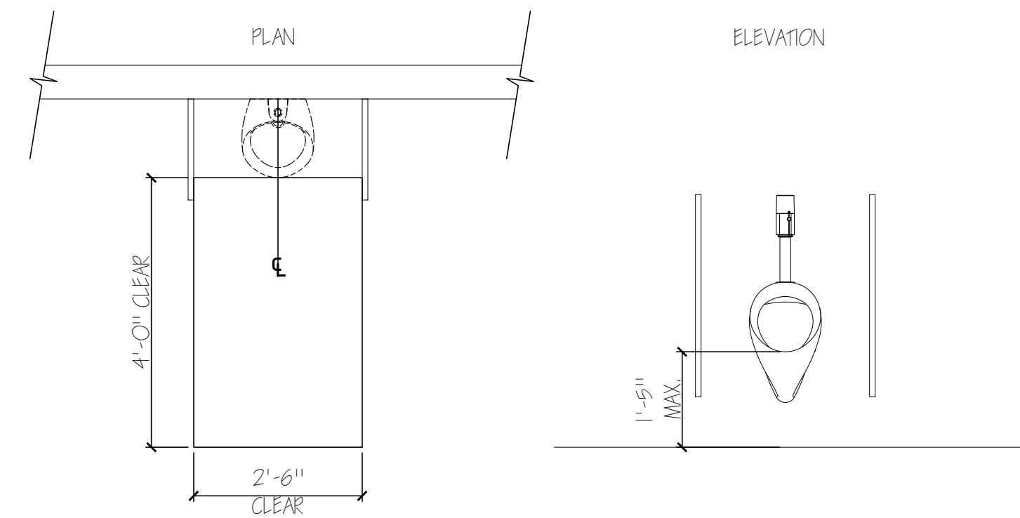
3 ADA URINAL CLEARANCES TYP. A-9 SCALE: 1/2" = 1'-0"
