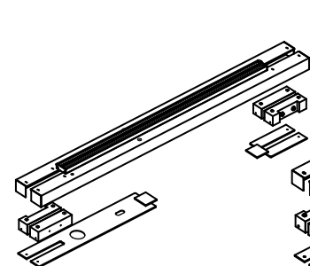
Floating Header (HDF-1750x4500-OHC) Sidelite Both
