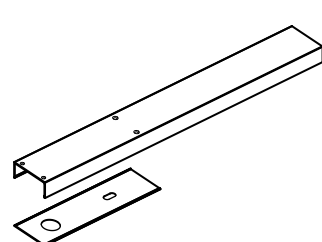
Overhead Closer Header (HDR-1750x4000-OHC)
