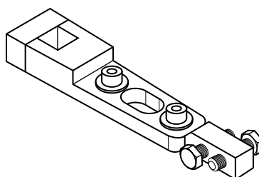
Overhead Closer Insert and Bottom Pivot (DOHC-275)
