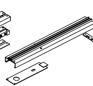
Floating Header (HDF-1750x4500-OHC) Sidelite None
