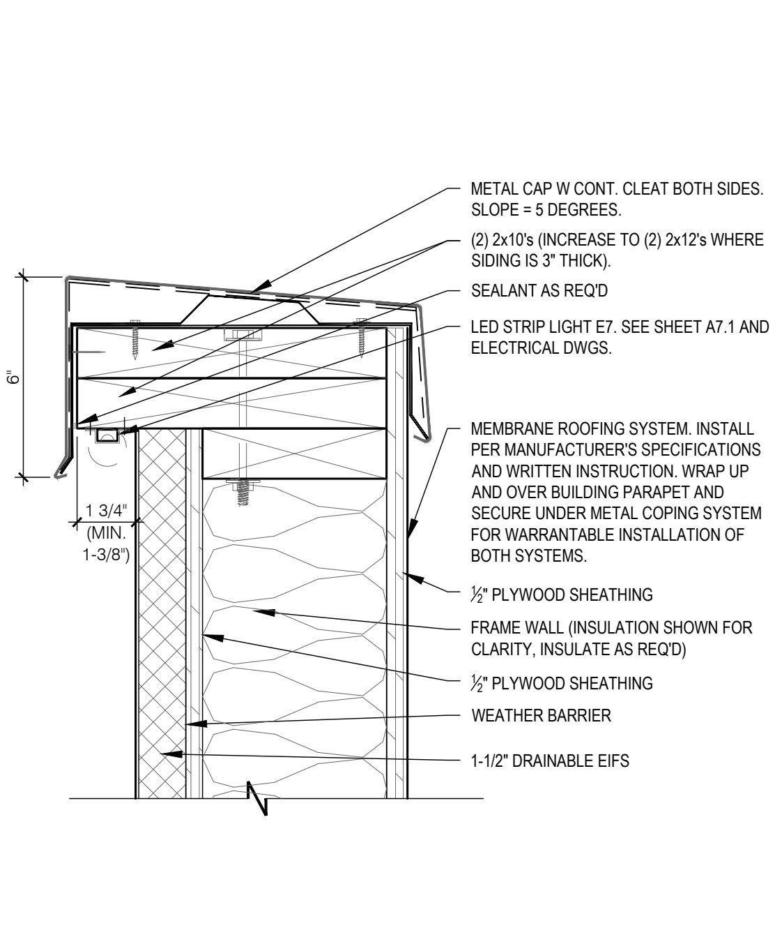
PARAPET CAP 3' = 1'-0" 17
