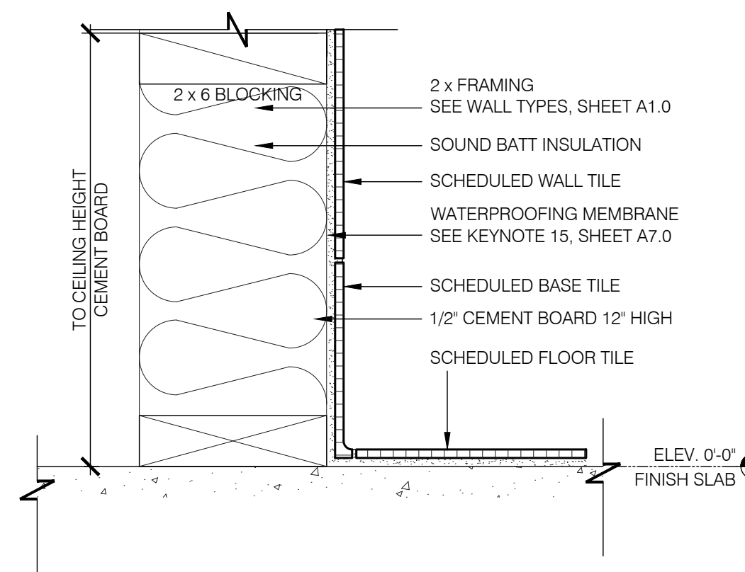
BASE at INT. PARTITION (RR's) 3"=1'-0" 10
