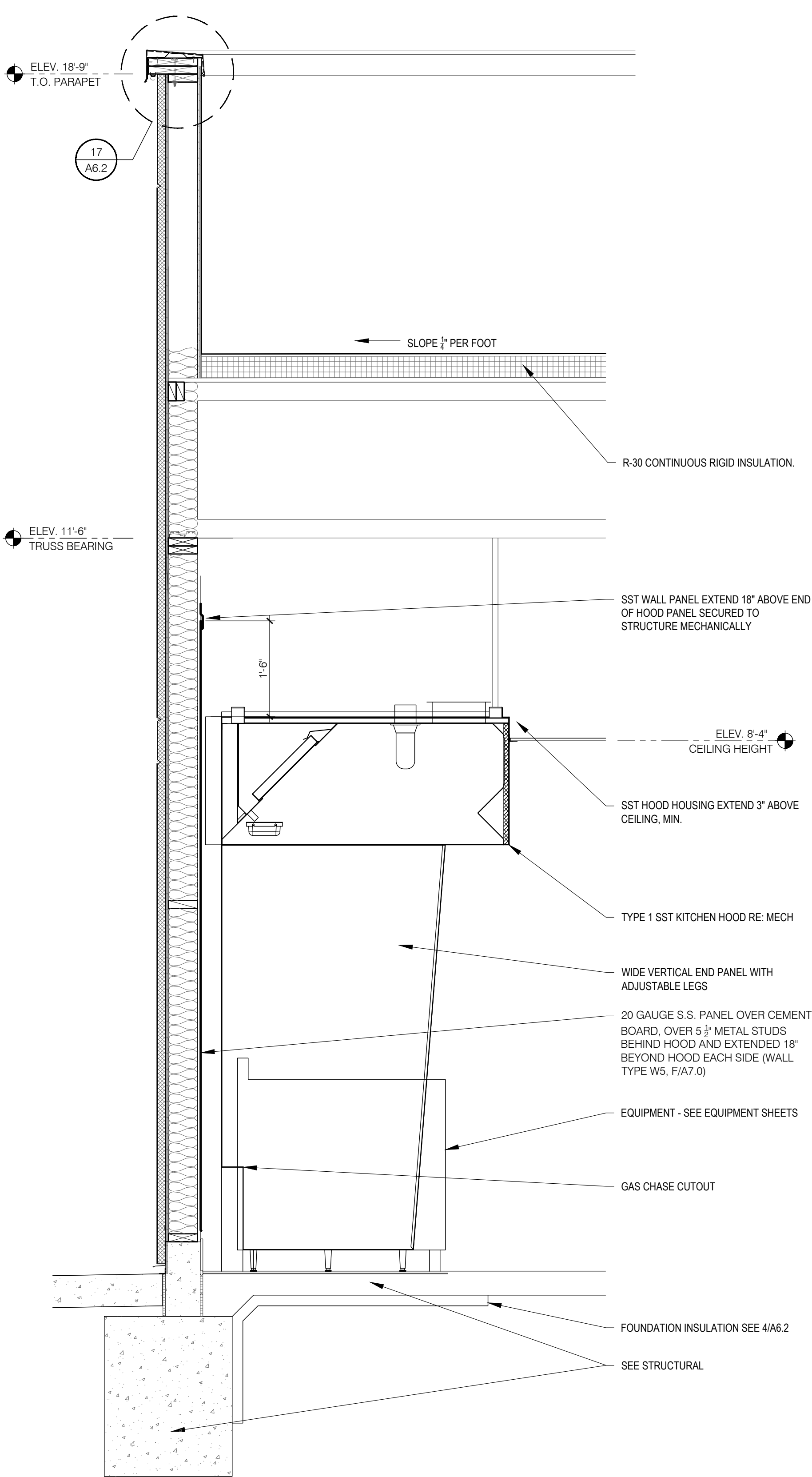
WALL SECTION at COOK LINE (SIDE WALL) 3/4" = 1'-0" A
