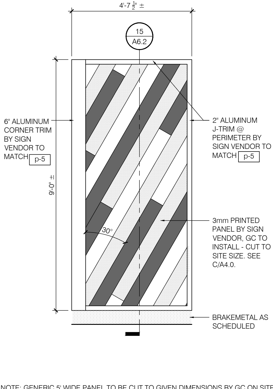
ELEVATION @ S44c WALL PANEL - EXT 1/2' = 1'-0" 14
