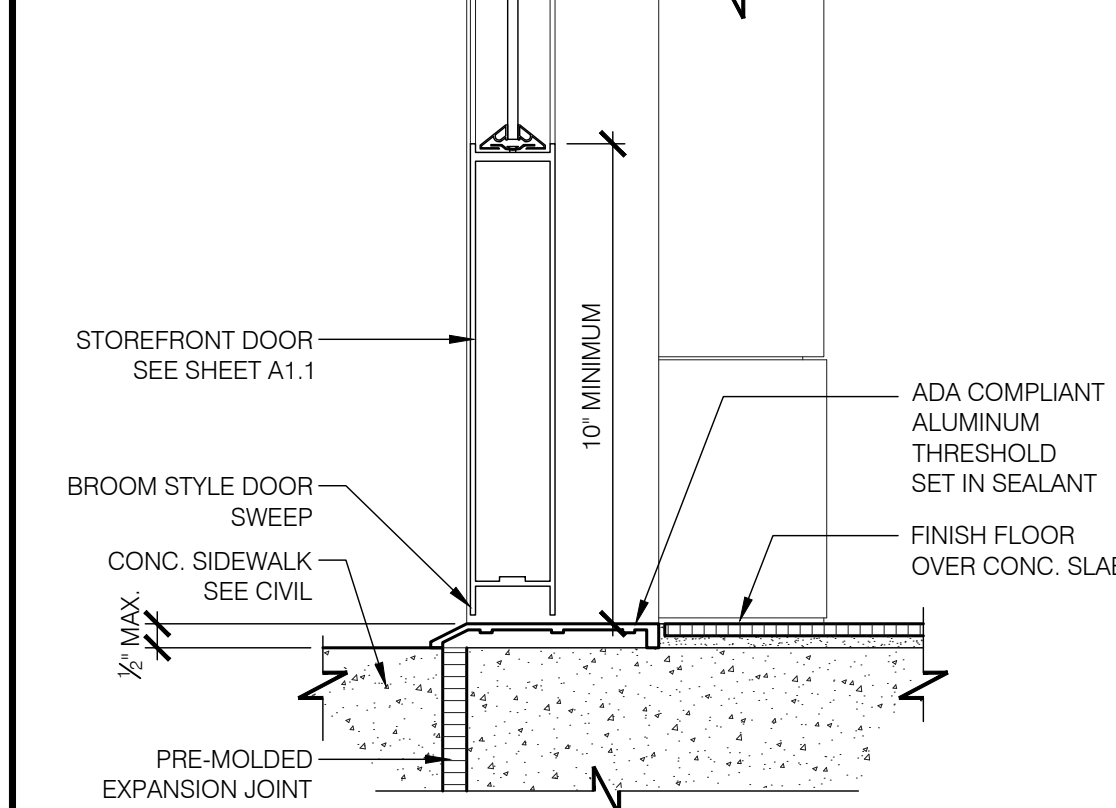
THRESHOLD at STOREFRONT DOOR 3"=1'-0" 1
