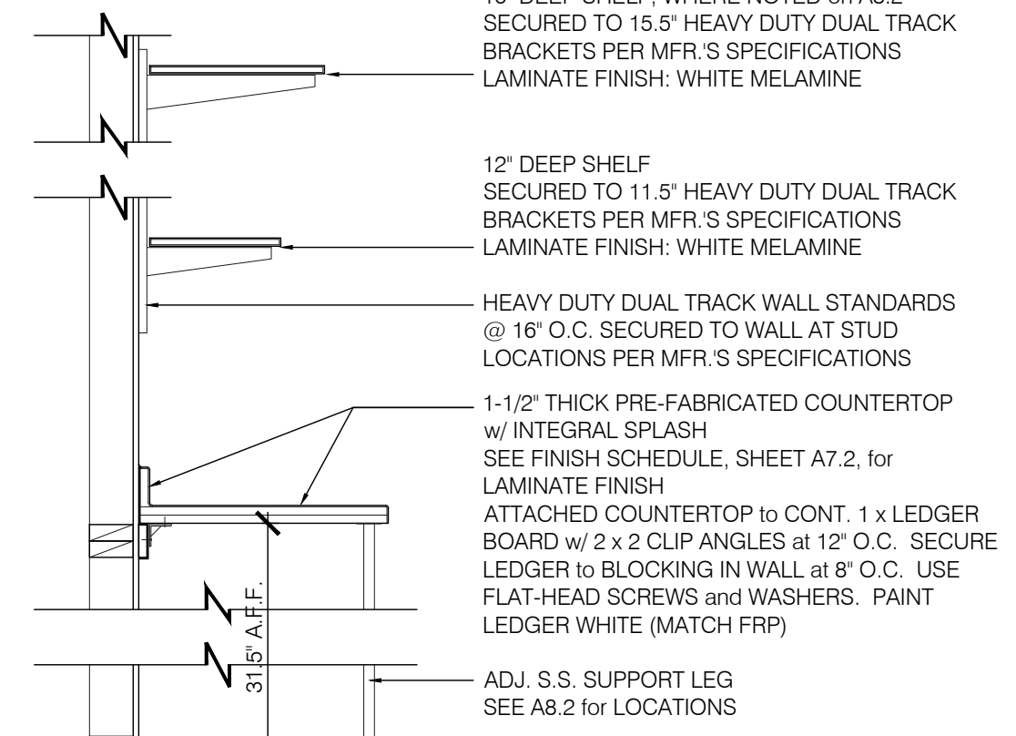
OFFICE COUNTER and SHELVING 3/4"=1'-0" 9
