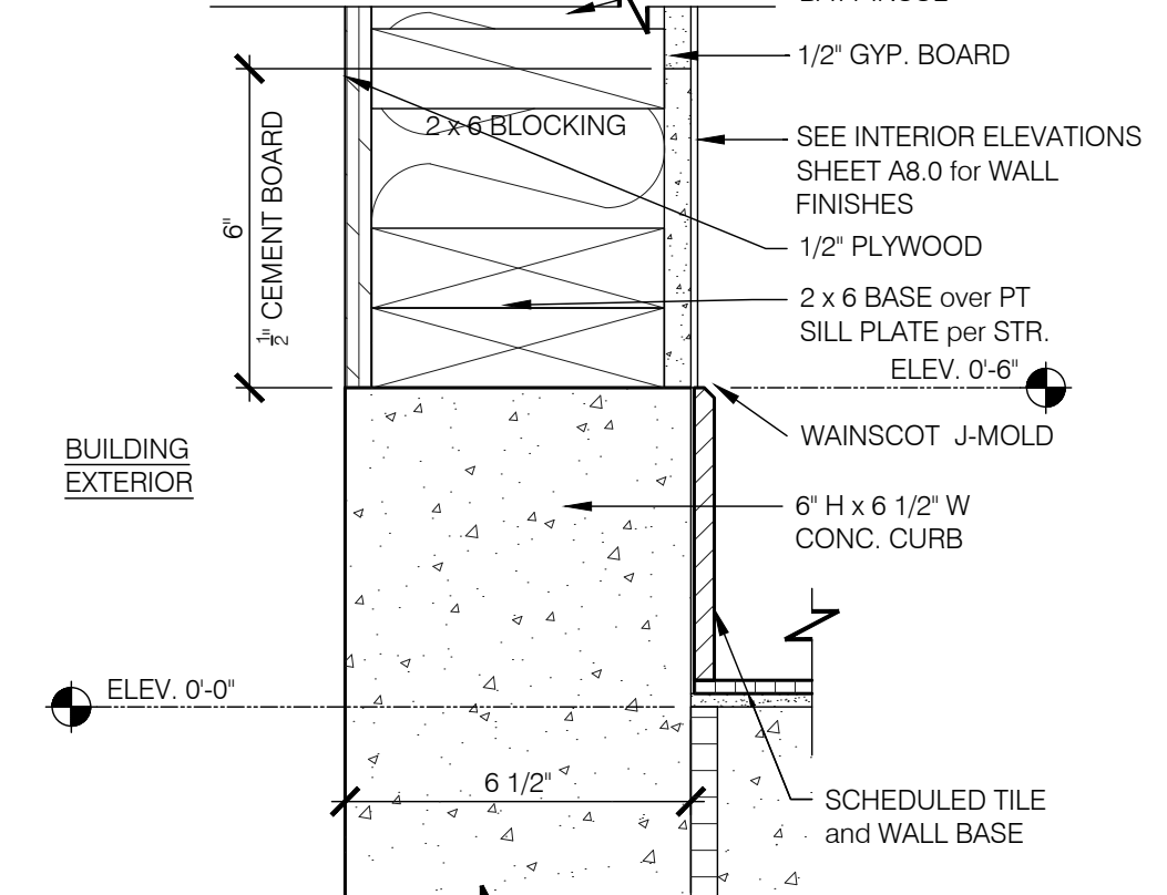
BASE at DINING (SIDE) 3"=1'-0" 3
