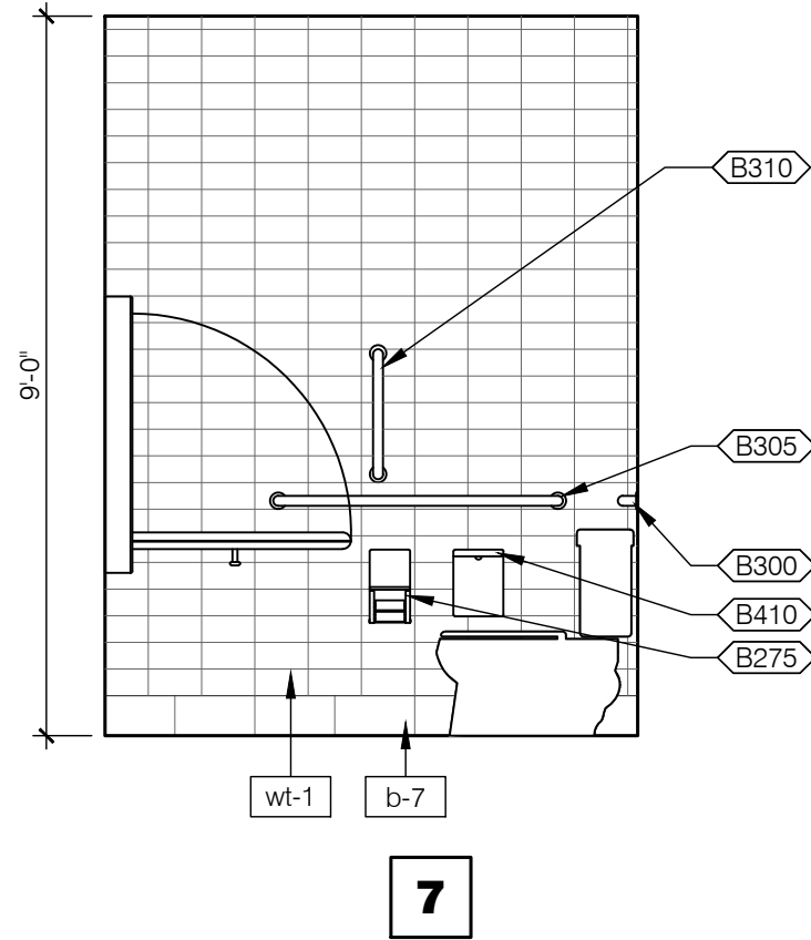
WOMEN'S RESTROOM 3/8" = 1'-0"
