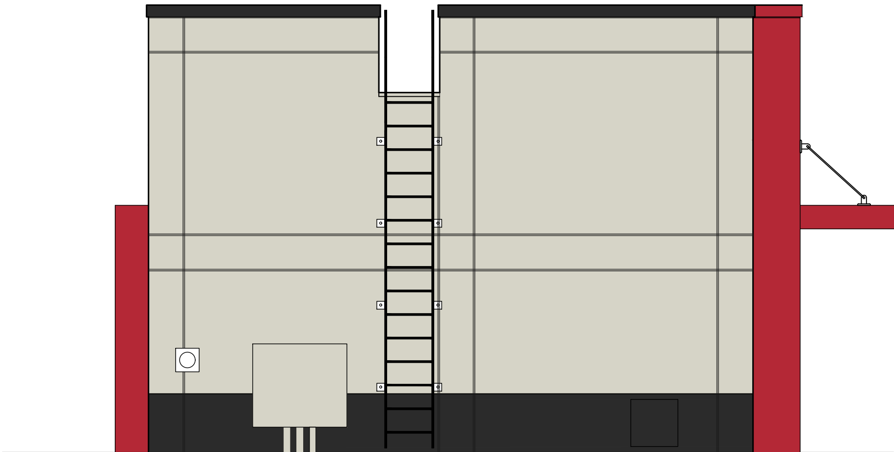
REAR ELEVATION
