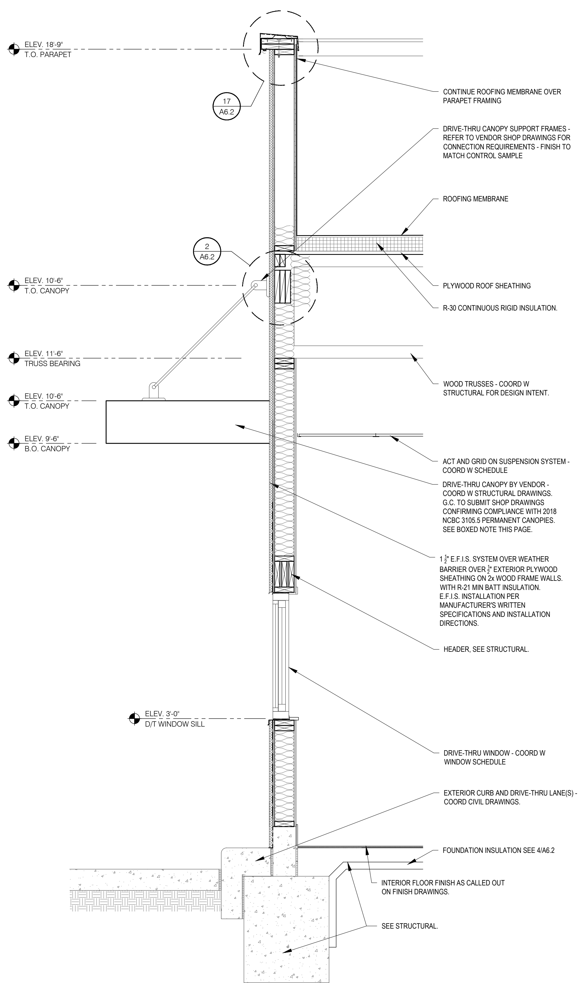
WALL SECTION at DRIVE THRU (SIDE WALL) 3/4" = 1'-0" B
