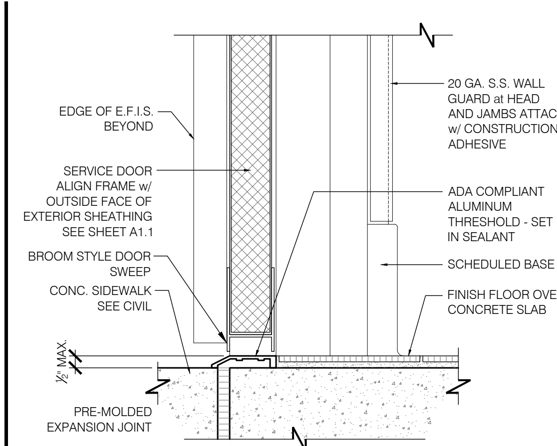
THRESHOLD at SERVICE DOOR 3"=1'-0" 16
