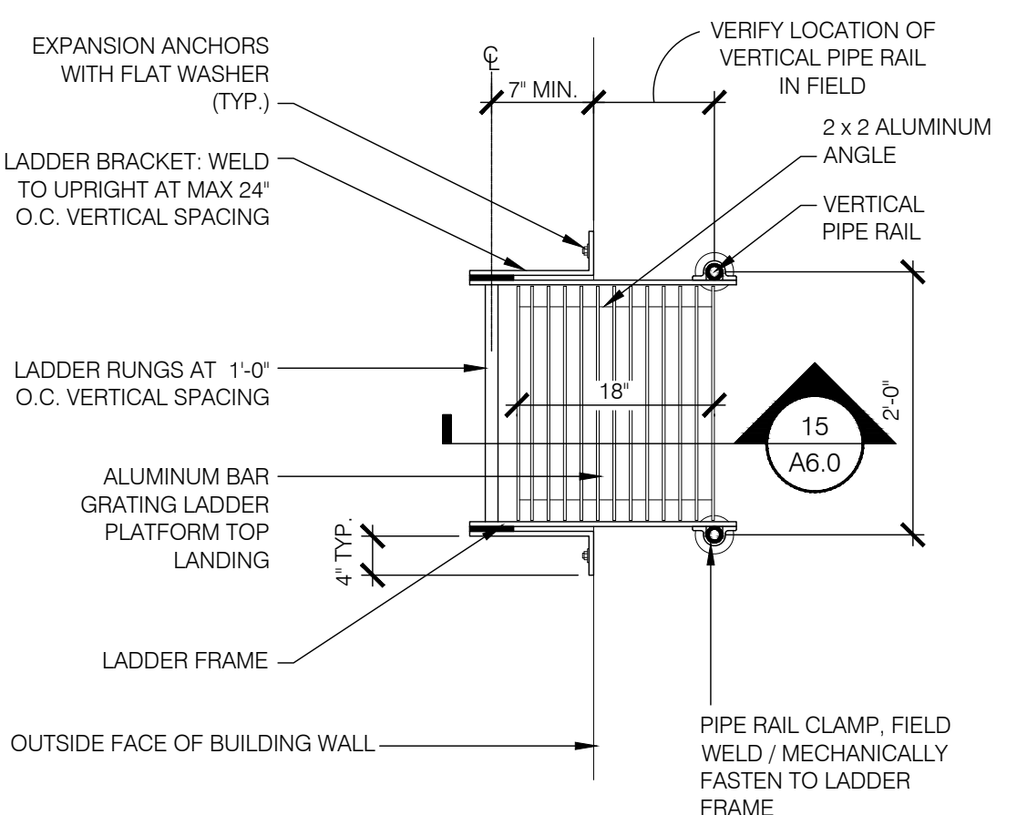
ROOF LADDER 1"=1'-0" 19
