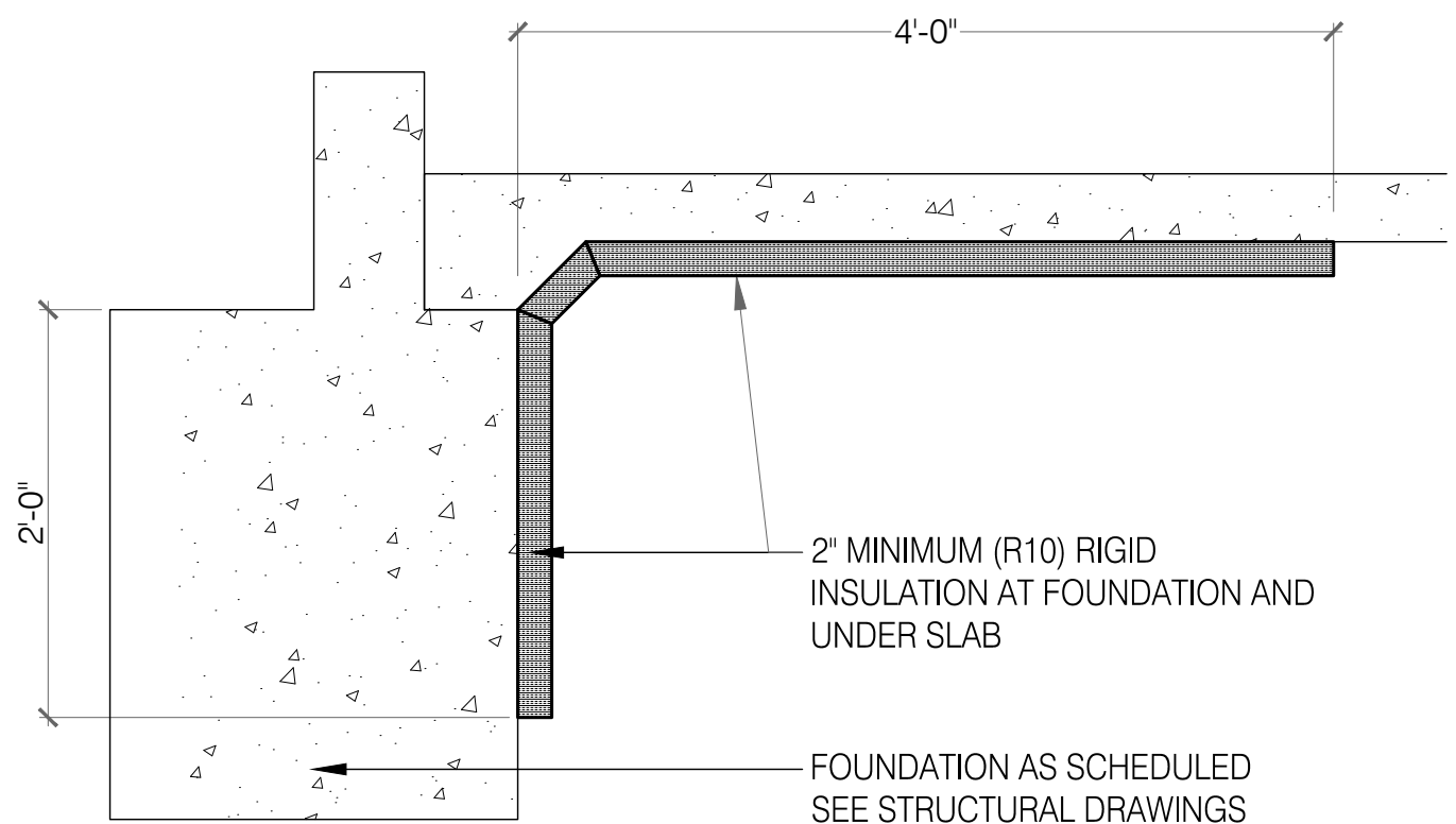
UNDER SLAB INSULATION DETAIL 1" = 1'-0" 4
