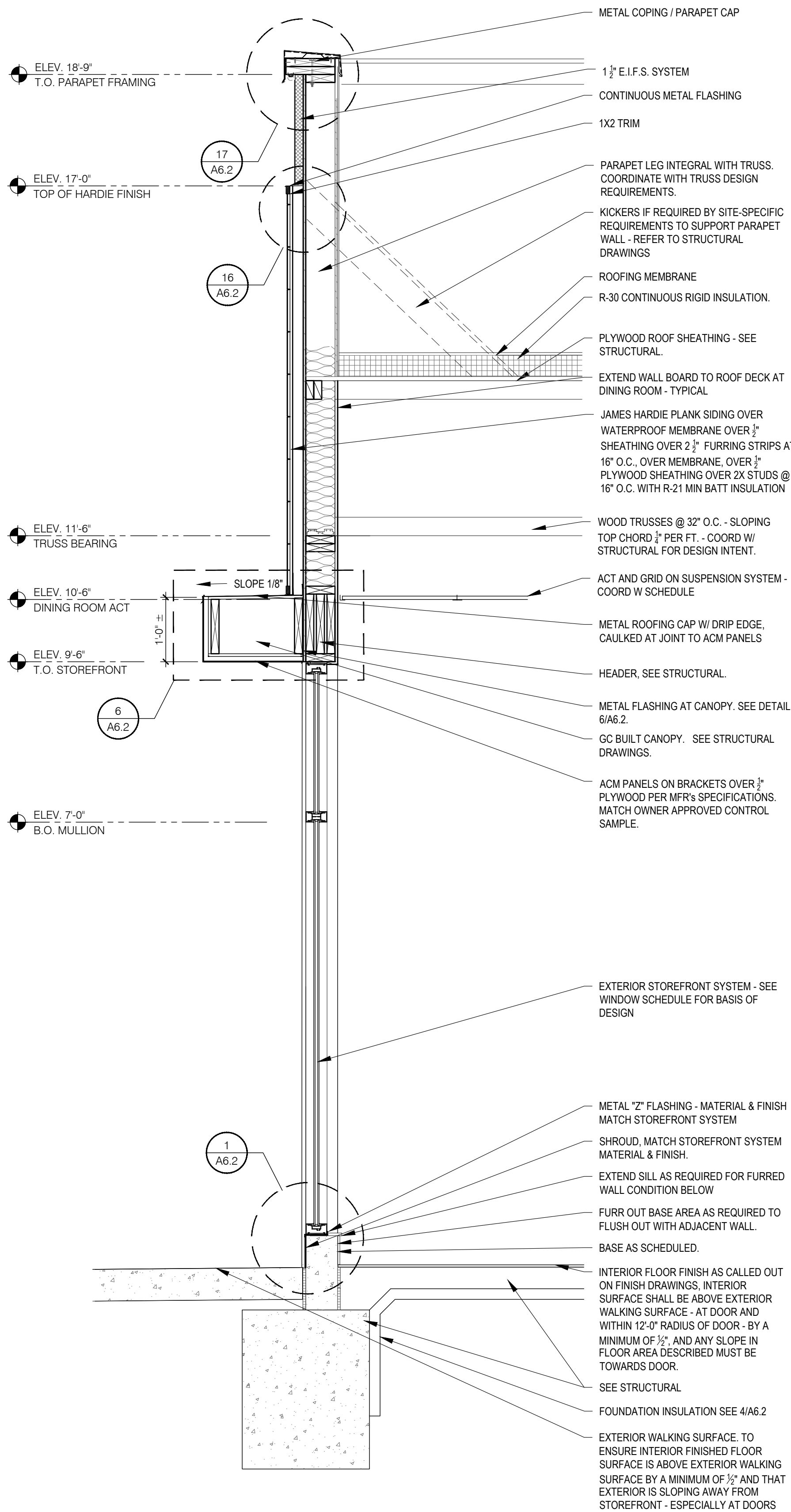
WALL SECTION at DINING SIDE WALL (FRONT WALL SIM.) 3/4" = 1'-0" B
