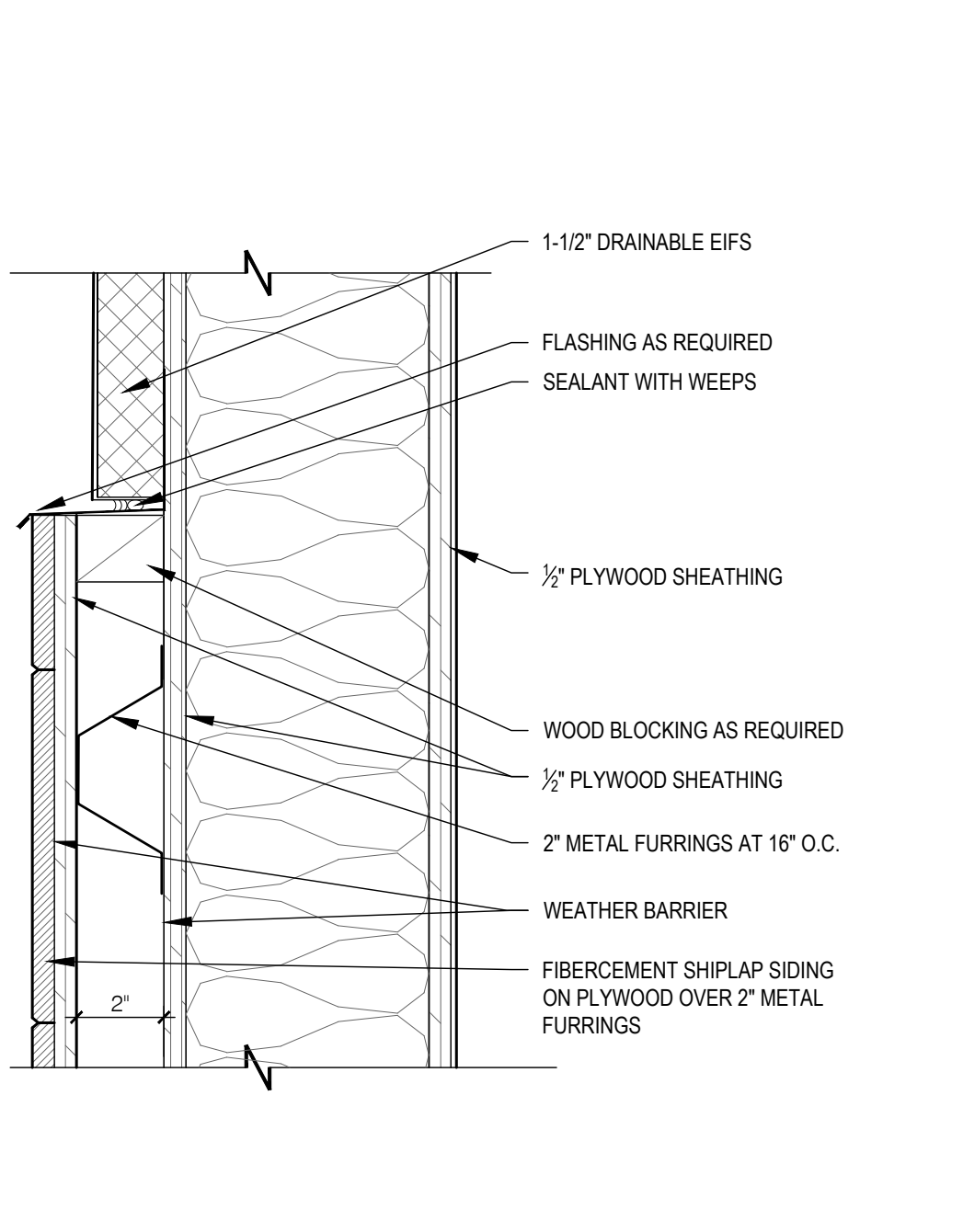
TOP OF PLANK SIDING TRANSITION 3' = 1'-0" 16
