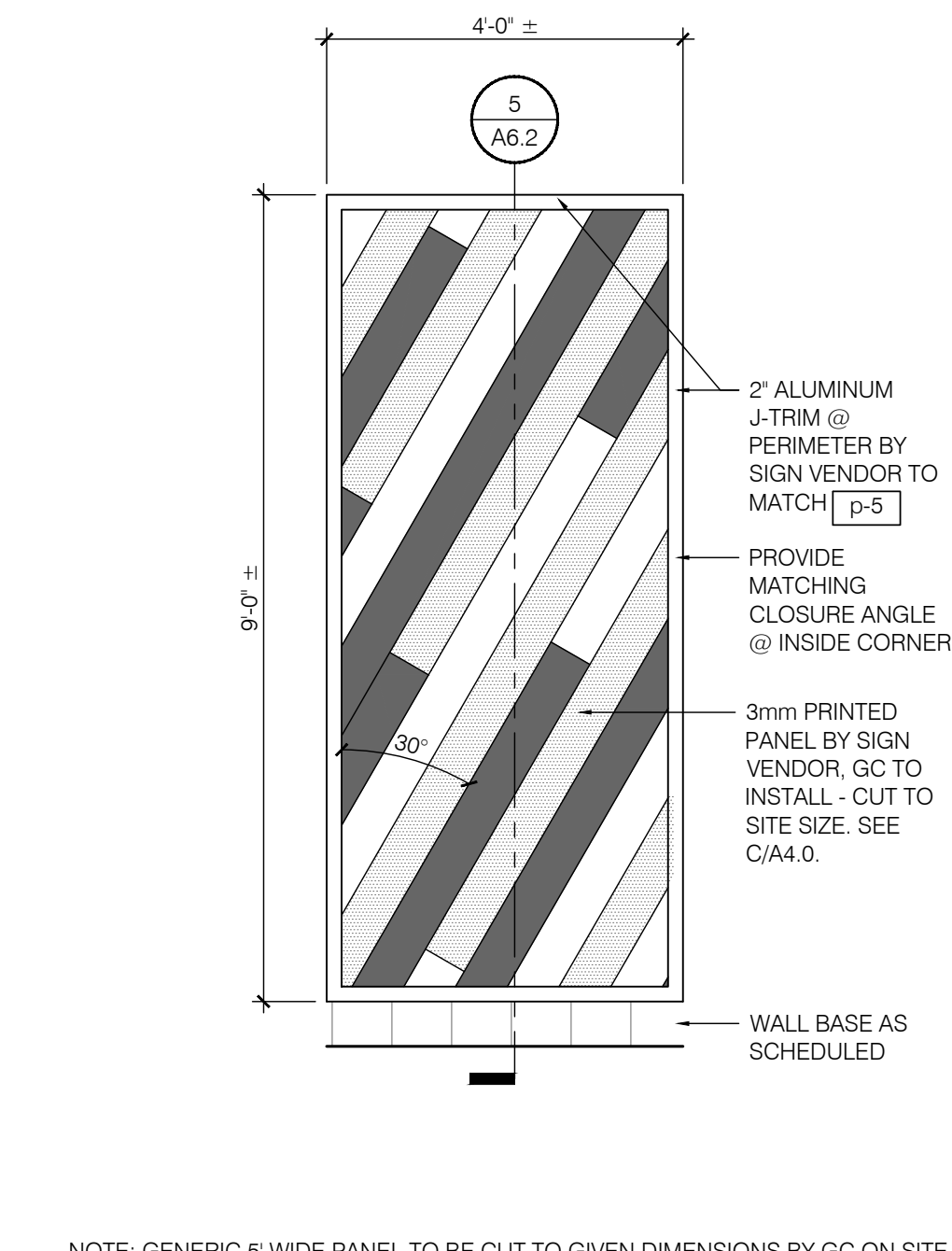
ELEVATION @ S44c WALL PANEL - INT 1/2' = 1'-0" 13
