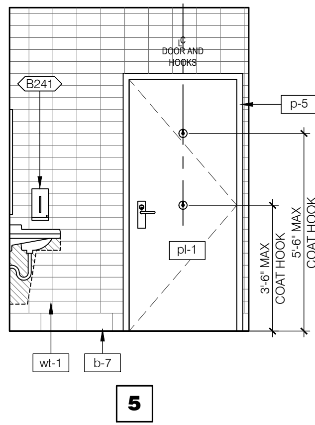
MEN'S RESTROOM 3/8" = 1'-0"
