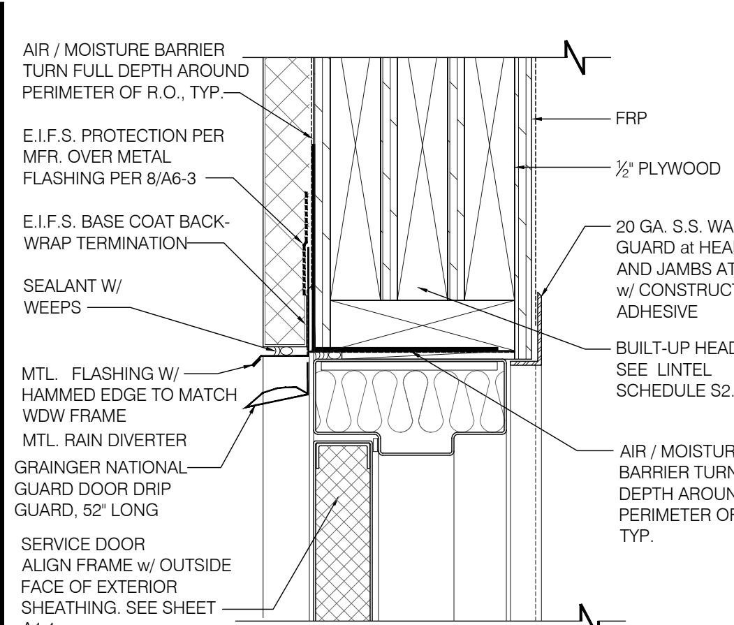
HEAD at SERVICE DOOR 3"=1'-0" 17
