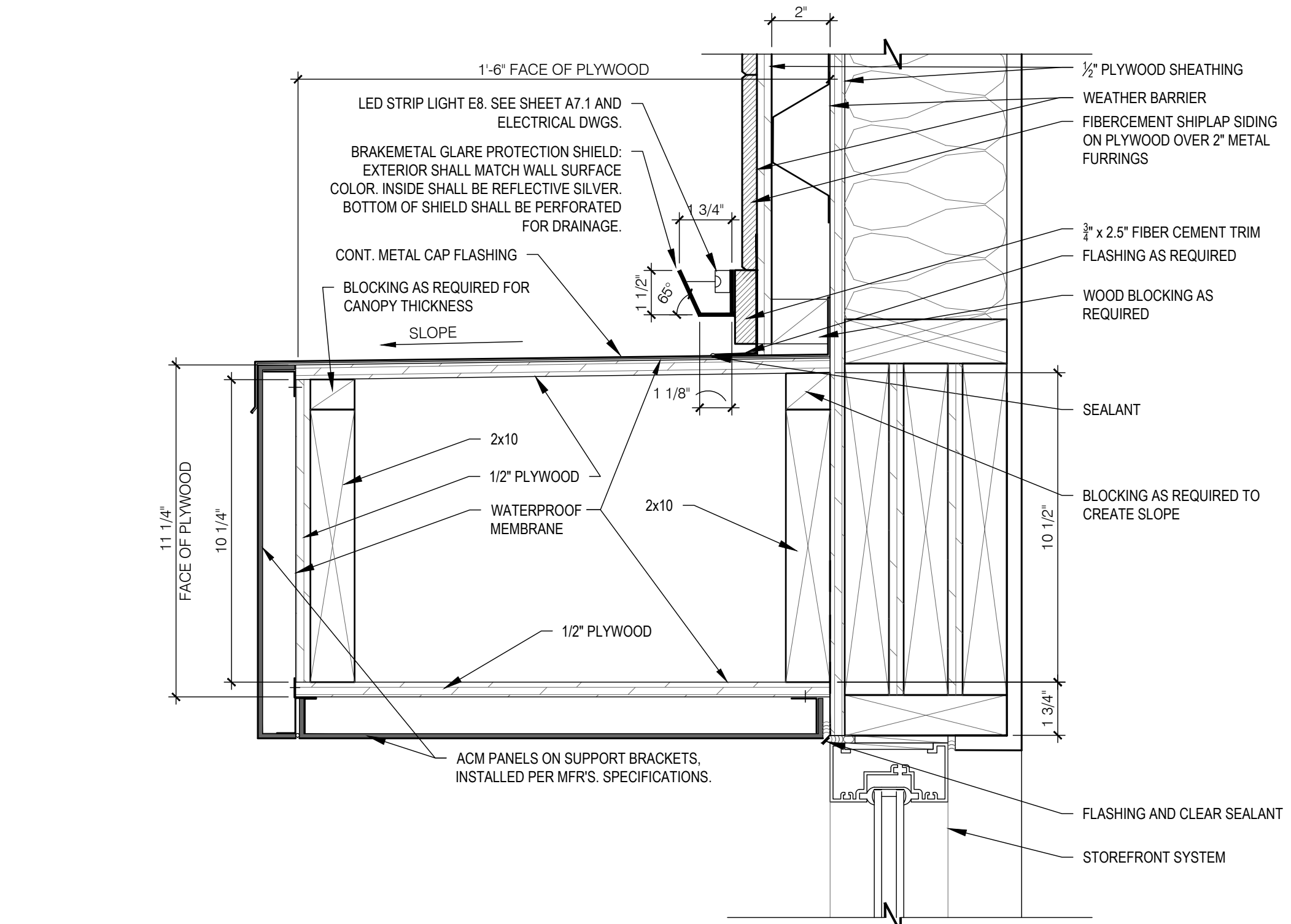
STOREFRONT AND EYEBROW CANOPY 3' = 1'-0" 6
