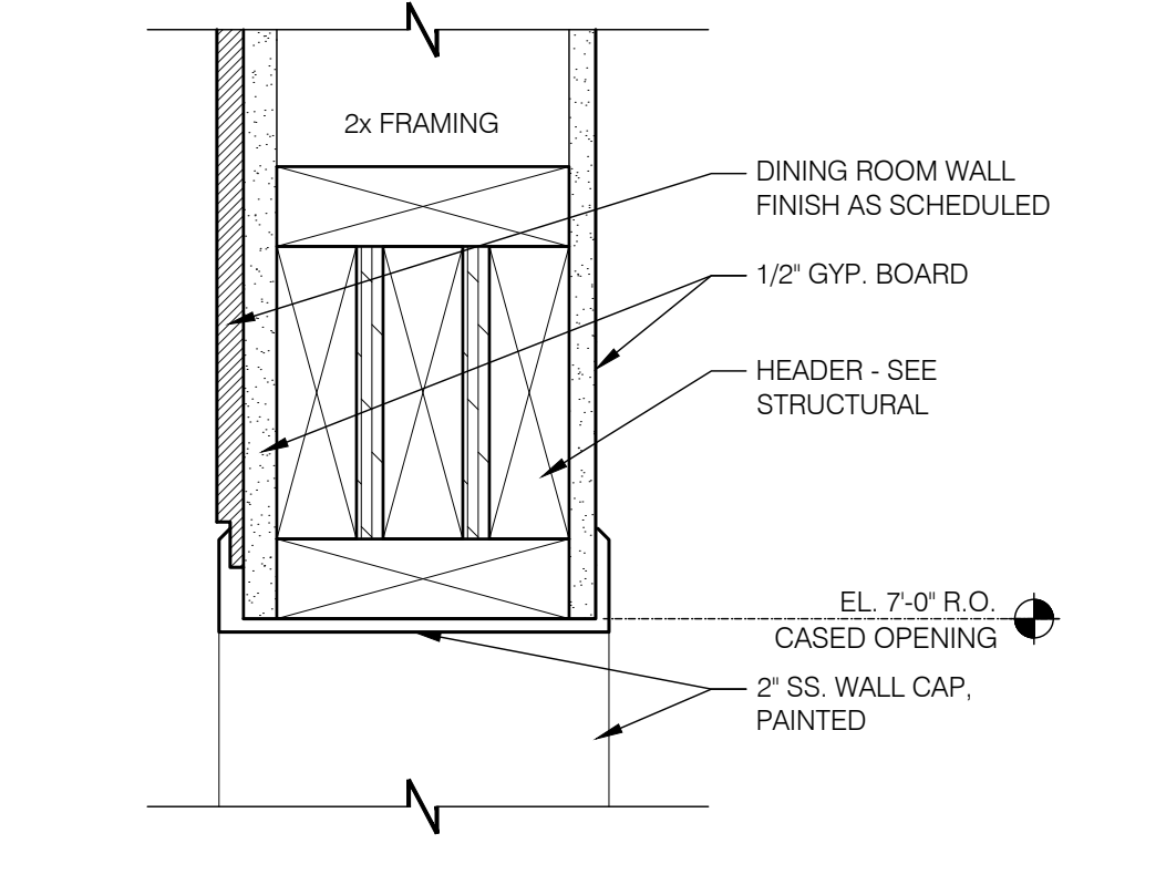
CASED OPENING DETAIL 3"=1'-0" 8
