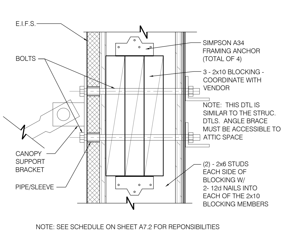
BLOCKING AT CANOPY 3' = 1'-0" 2
