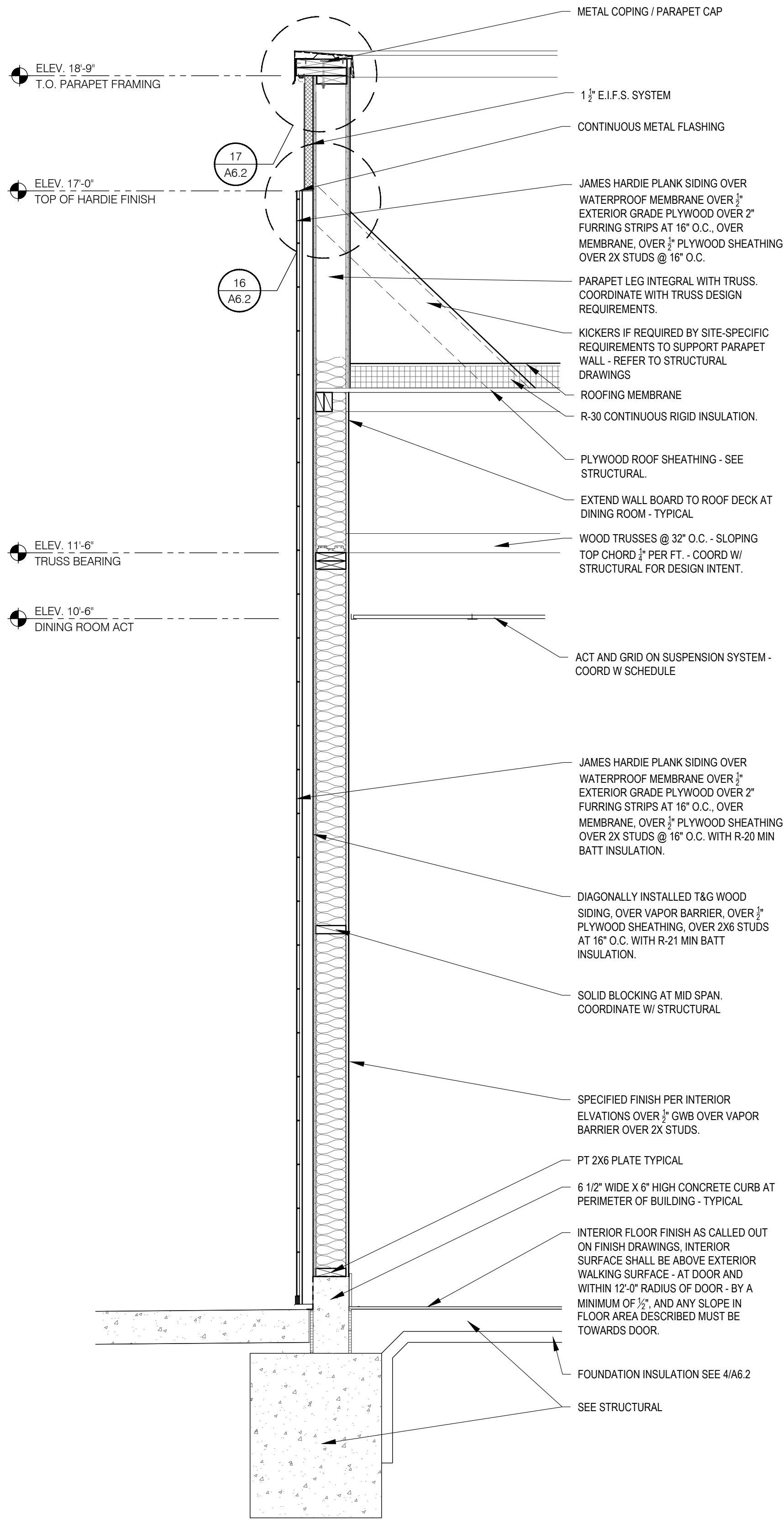
WALL SECTION at DINING (SIDE WALL) 3/4" = 1'-0" C
