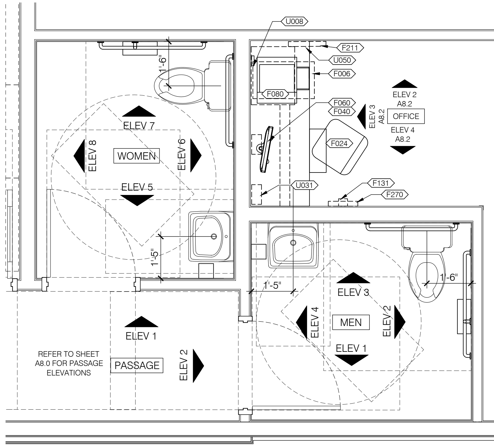
ENLARGED RESTROOM / OFFICE PLAN 1/2" = 1'-0" A
