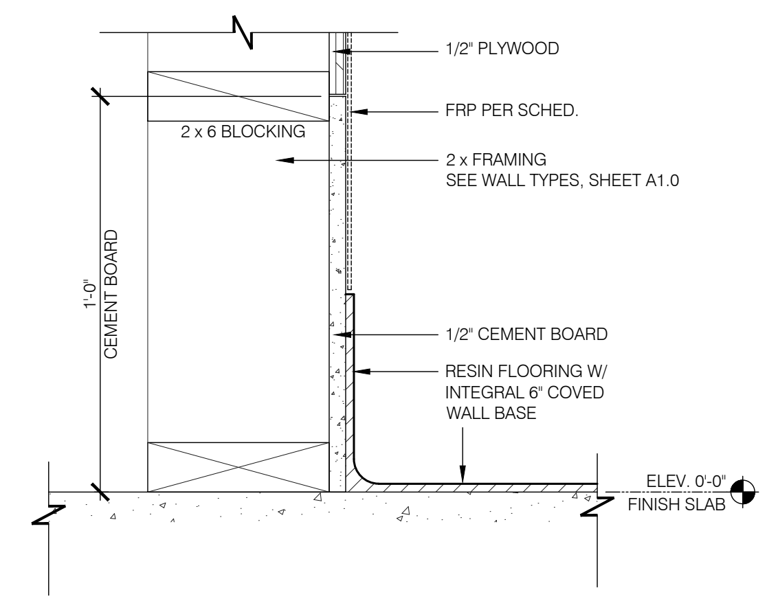
BASE at INT. PARTITION (KITCHEN) 3"=1'-0" 14
