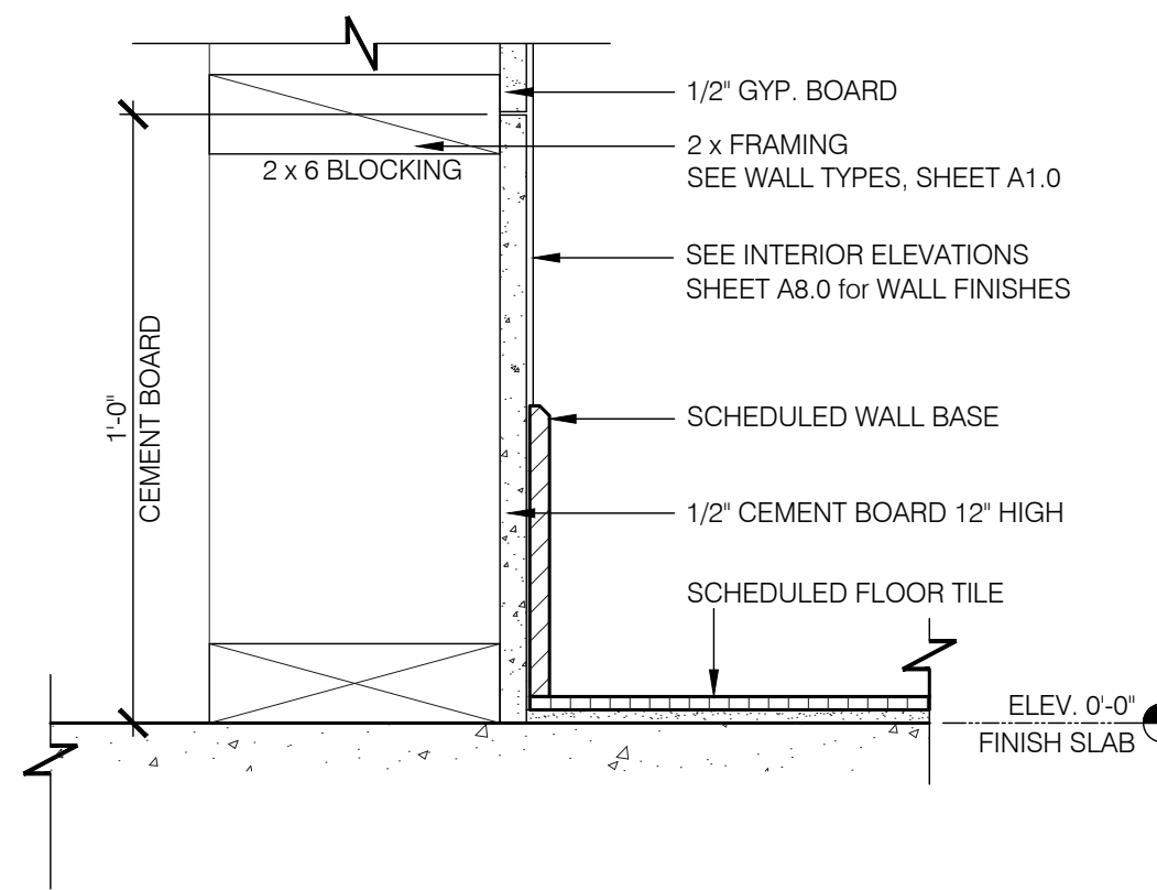
BASE at INT. PARTITION (DINING) 3"=1'-0" 5
