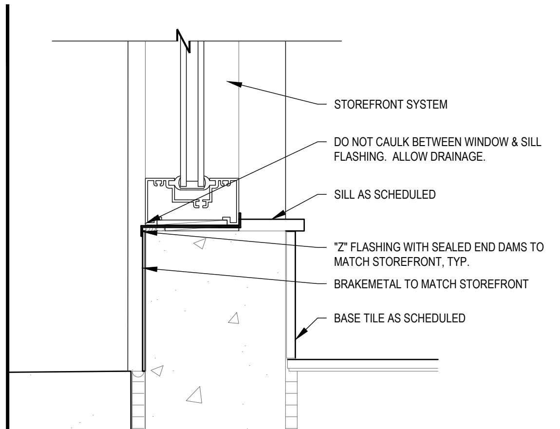
SILL AT STOREFRONT 3' = 1'-0" 1
