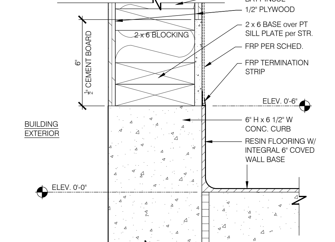
BASE at KITCHEN (SIDE and REAR) 3"=1'-0" 4
