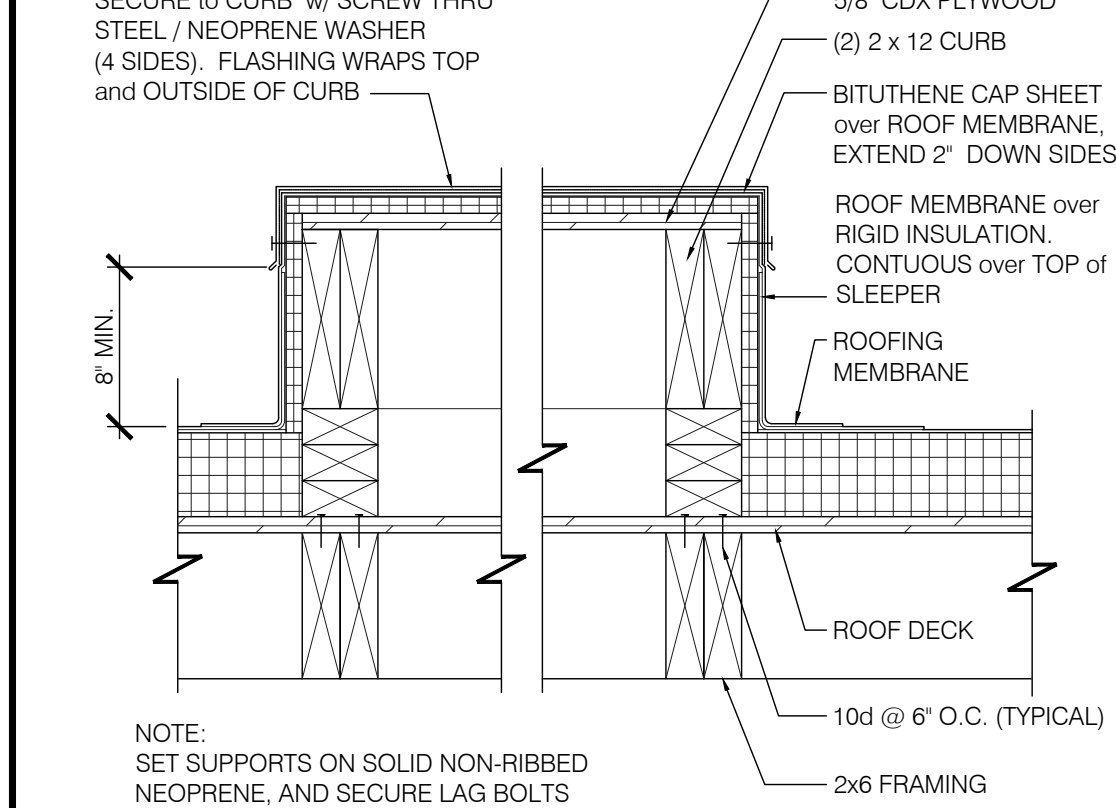
EQUIPMENT PLATFORM (OPTIONAL) 1 1/2"=1'-0" 6
