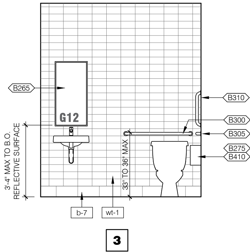
MEN'S RESTROOM 3/8" = 1'-0"
