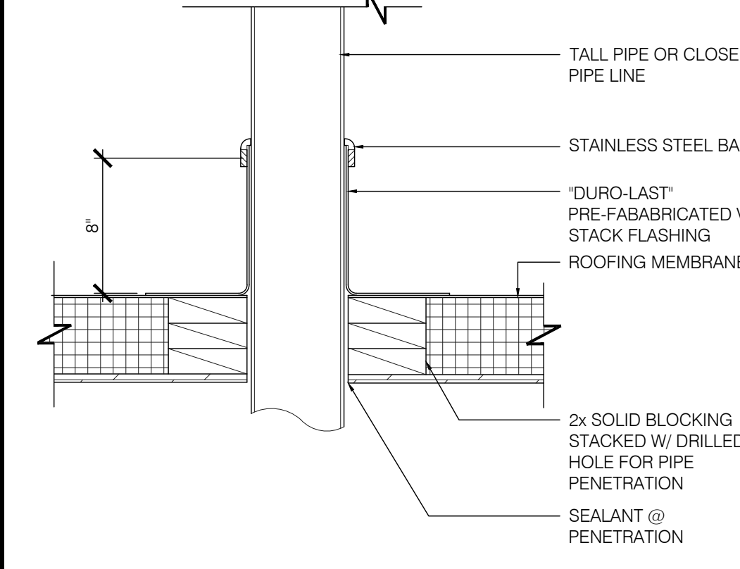
SEALED PIPE FLASHING 1 1/2"=1'-0" 2
