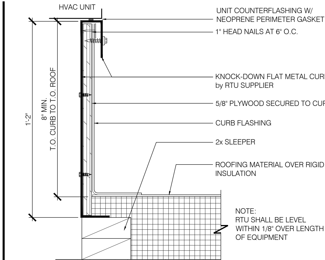
HVAC CURB 3"=1'-0" 11
