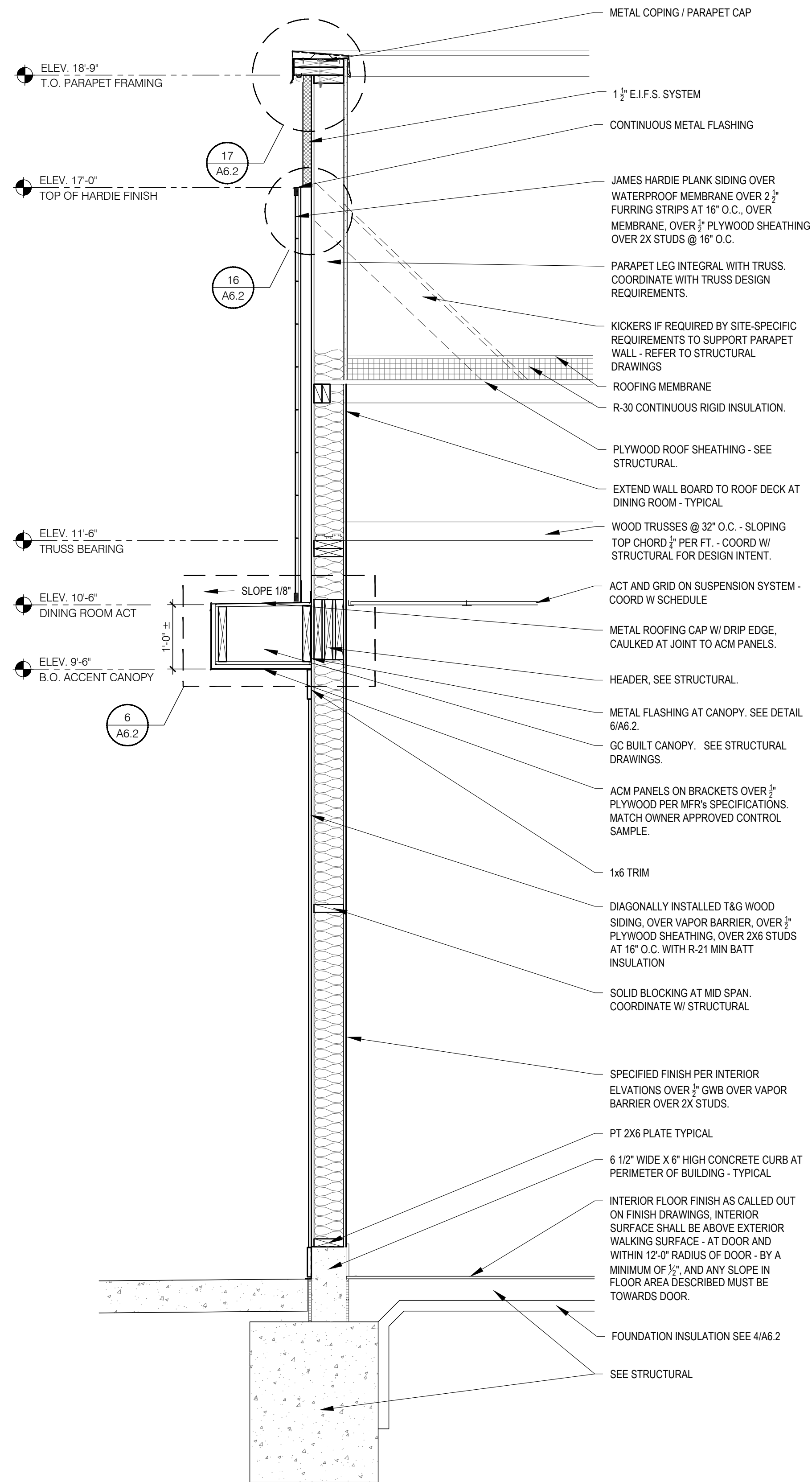
WALL SECTION at DINING (SIDE WALL) 3/4" = 1'-0" A
