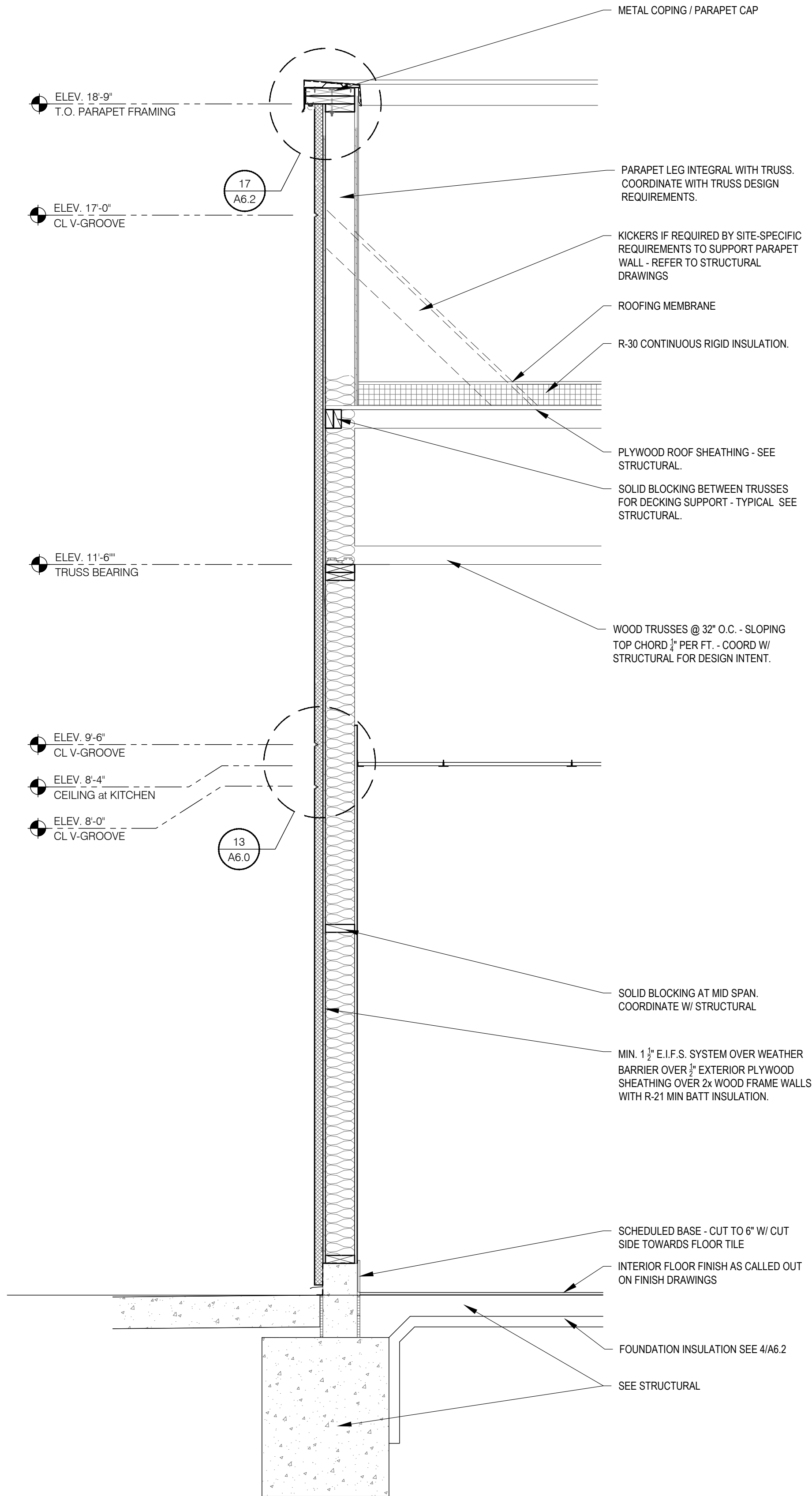
WALL SECTION at SIDE WALL 3/4" = 1'-0" C
