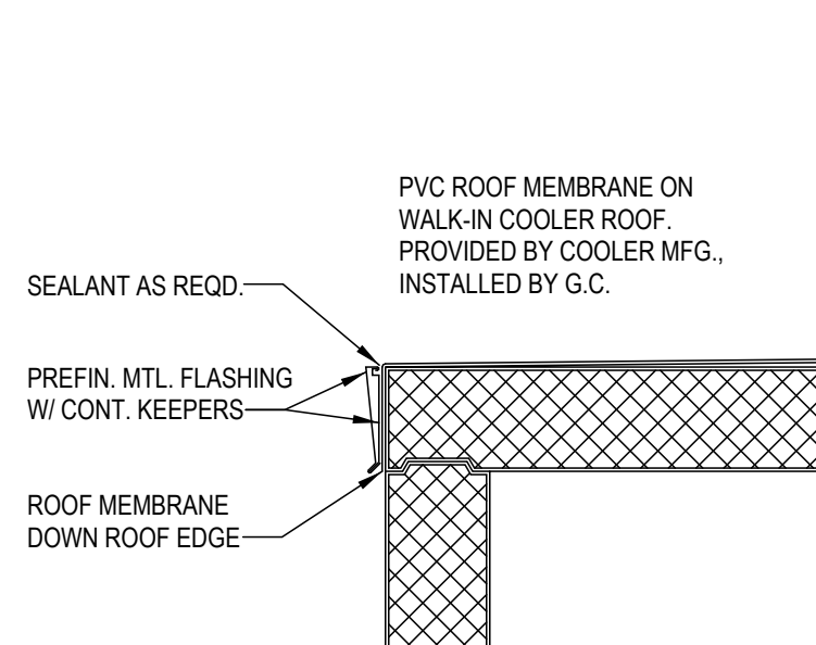
14 WALK-IN ROOF DETAIL A-303 SCALE: 1 1/2" = 1'-0"
