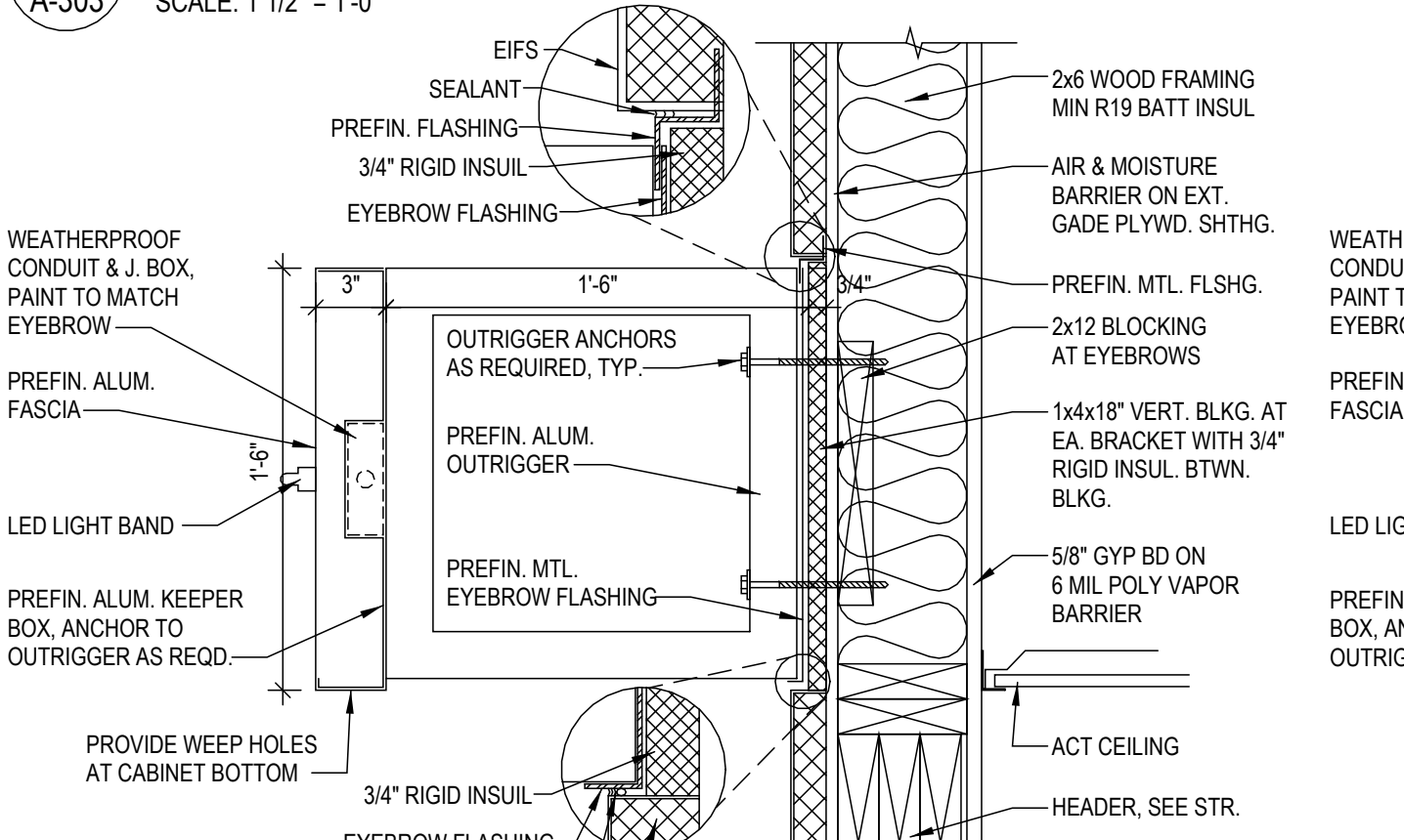
6 ENTRY CANOPY DETAIL A-303 SCALE: 1 1/2" = 1'-0"
