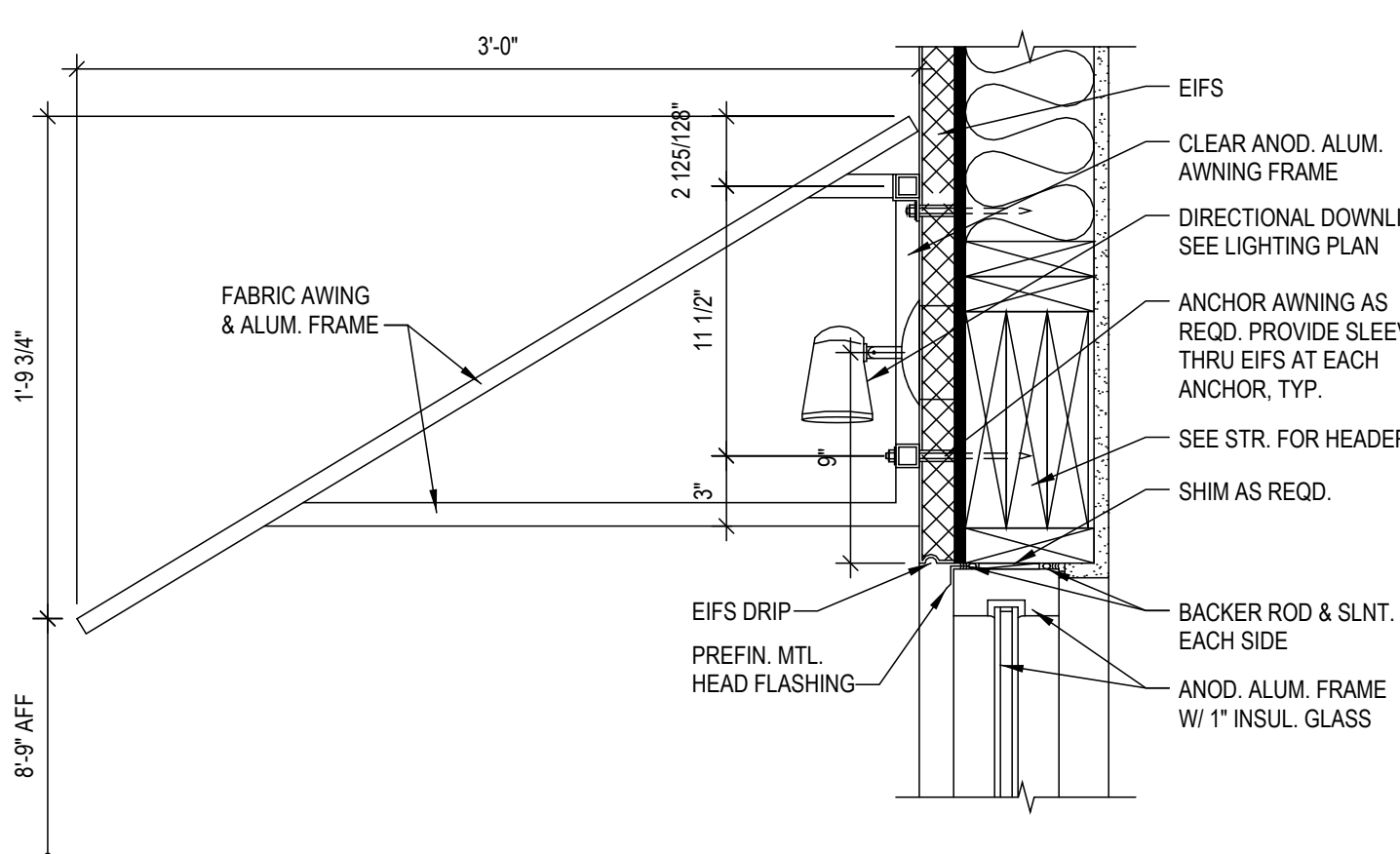
6 ENTRY CANOPY DETAIL A-303 SCALE: 1 1/2" = 1'-0"
