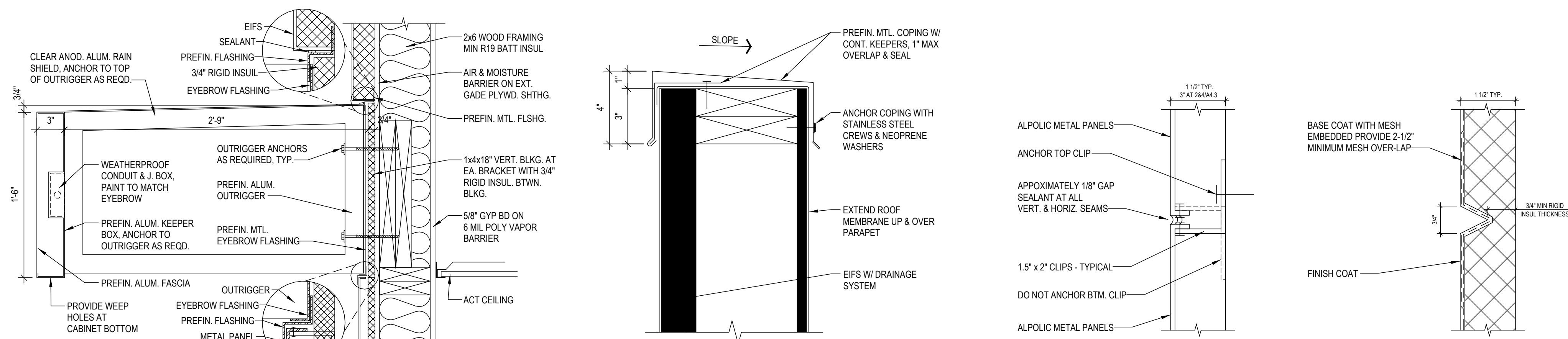
3/4" RIGID INSUL- DT CANOPY DETAIL 3 A-303 SCALE: 1 1/2" = 1'-0"
