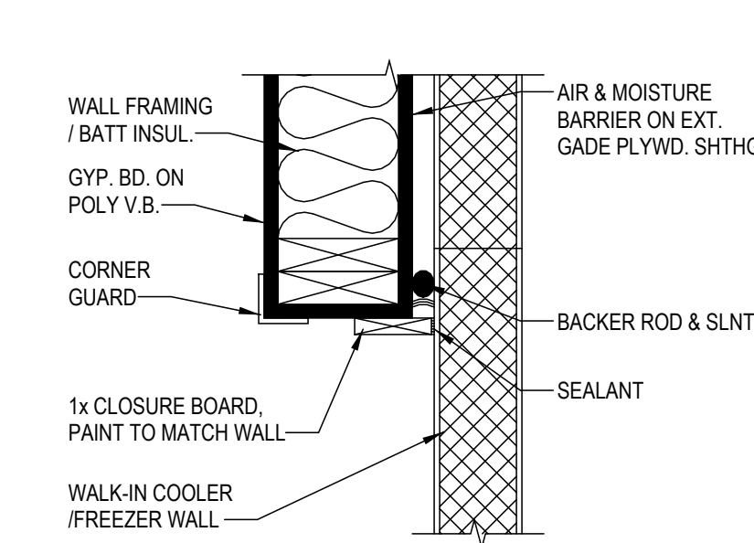
17 WALK-IN PLAN DETAIL A-303 SCALE: 1 1/2" = 1'-0"
