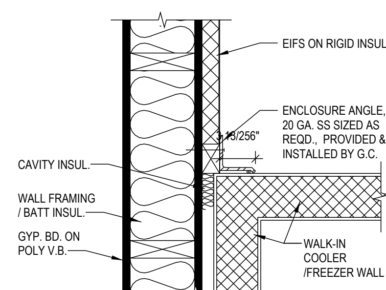
16 WALK-IN PLAN DETAIL A-303 SCALE: 1 1/2" = 1'-0"
