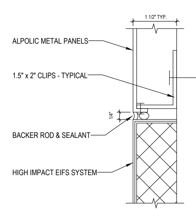
21 ALPOLIC/EIFS TRANSITION
