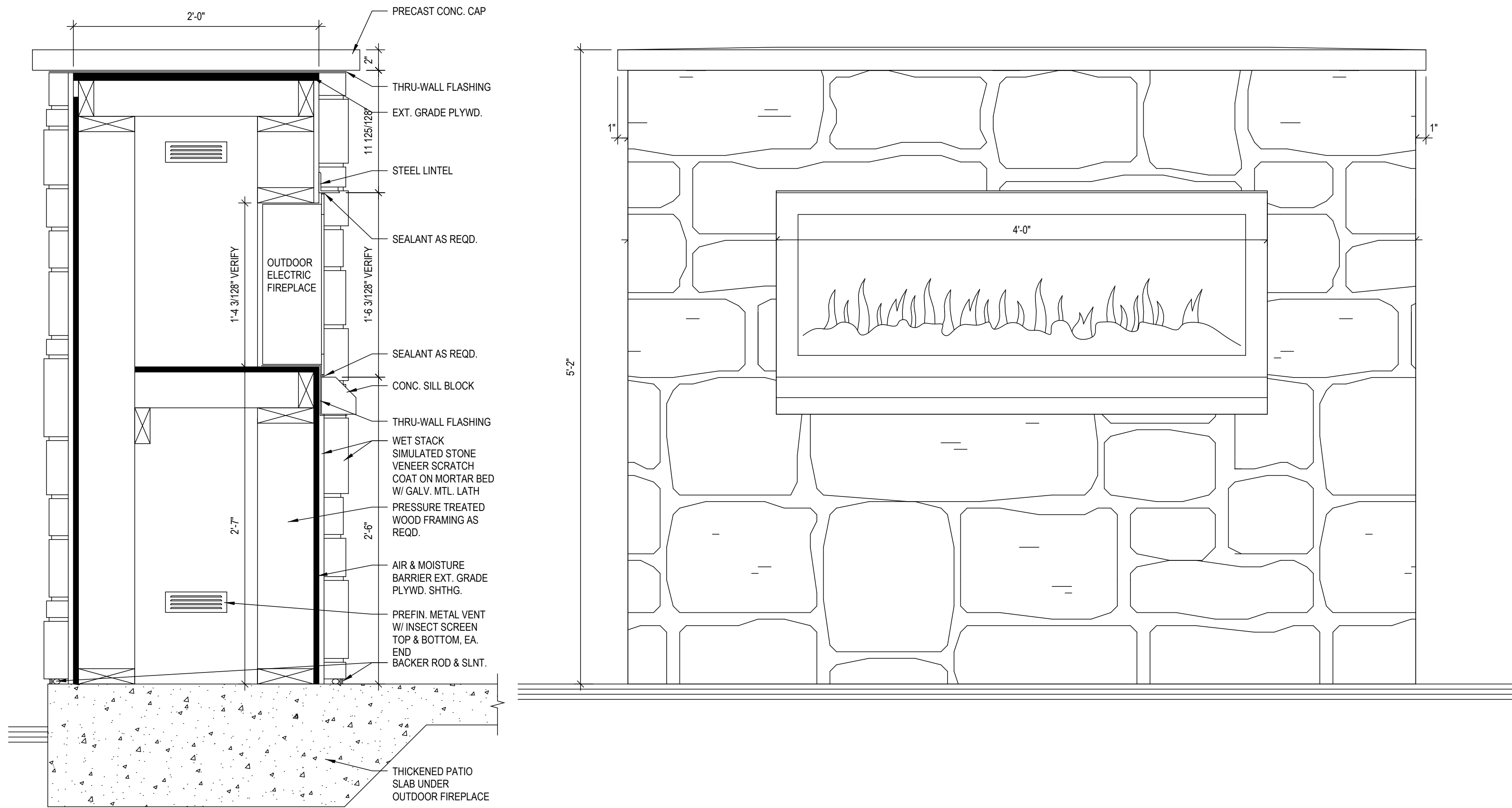
1 OPTIONAL OUTDOOR FIREPLACE DTL. A4.4 SCALE: 1 1/2" = 1'-0"
