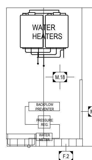
17 INTERIOR ELEVATION Scale is 1/4" = 1'-0" when printed full size.
