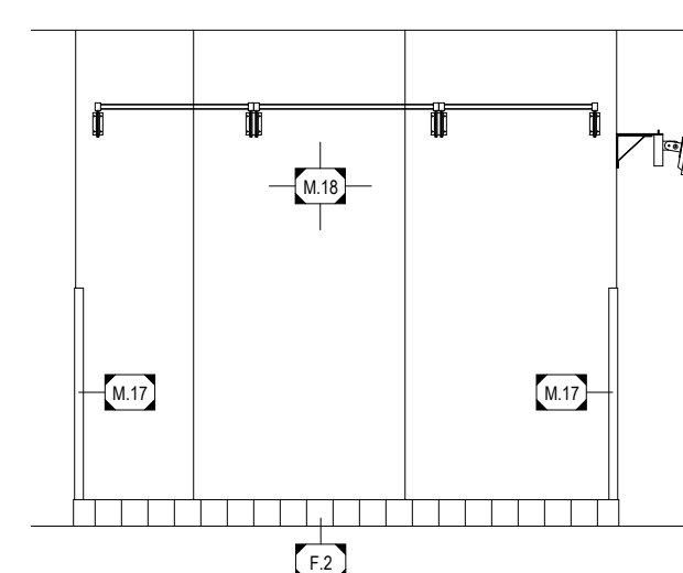
18 INTERIOR ELEVATION Scale is 1/4" = 1'-0" when printed full size.
