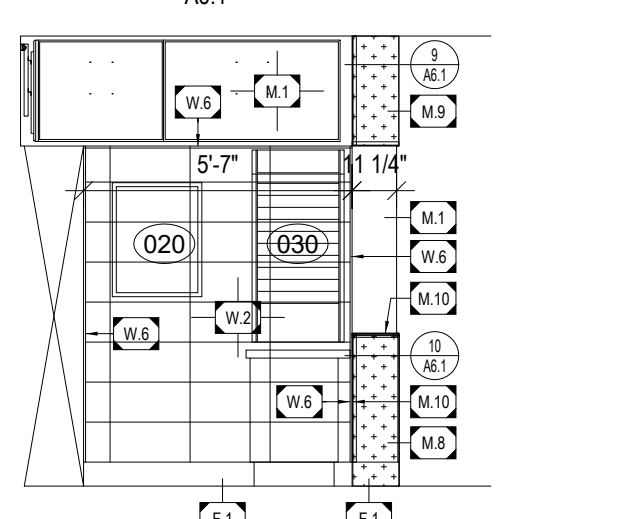
3 INTERIOR ELEVATION Scale is 1/4" = 1'-0" when printed full size.
