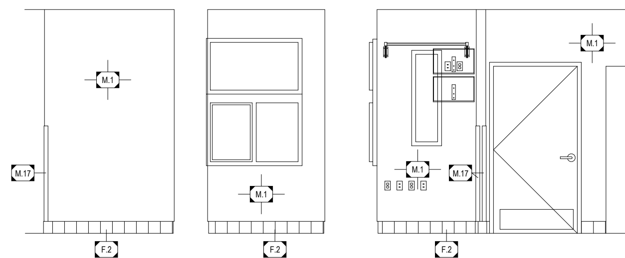
23 INTERIOR ELEVATION Scale is 1/4" = 1'-0" when printed full size.
