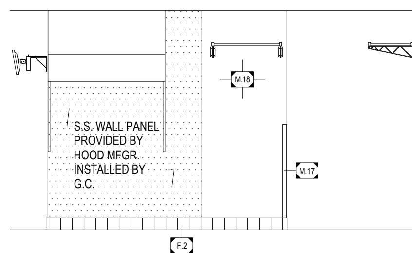
22 INTERIOR ELEVATION Scale is 1/4" = 1'-0" when printed full size.
