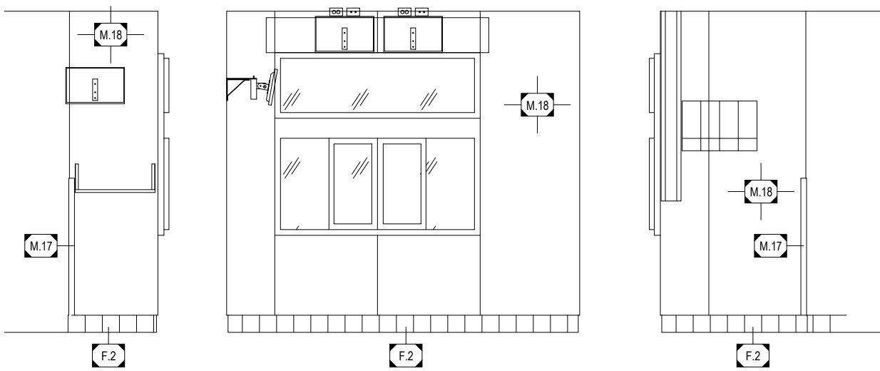
14 INTERIOR ELEVATION Scale is 1/4" = 1'-0" when printed full size.
