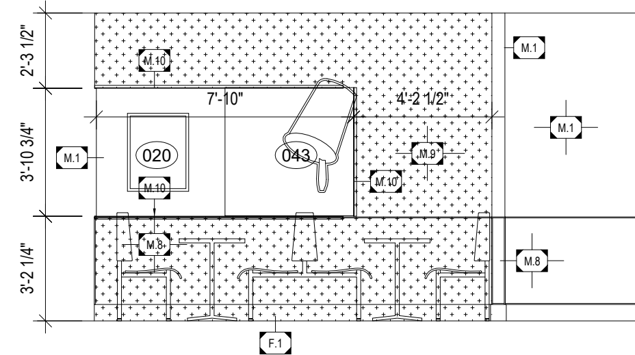
4 INTERIOR ELEVATION Scale is 1/4" = 1'-0" when printed full size.
