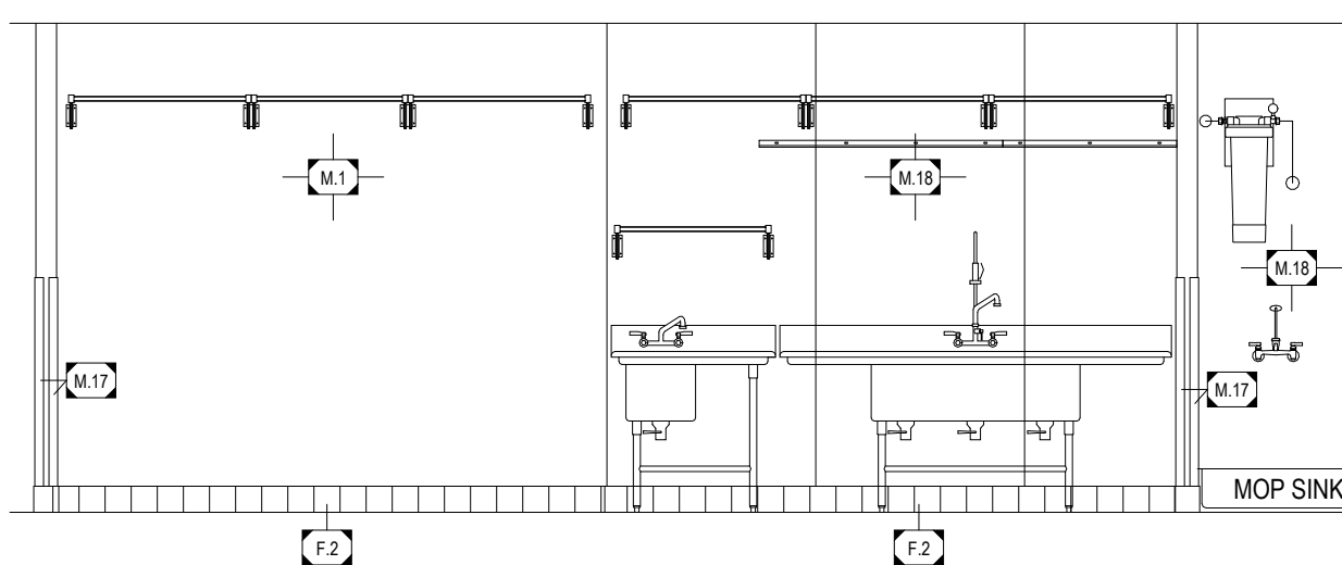
16 INTERIOR ELEVATION Scale is 1/4" = 1'-0" when printed full size.
