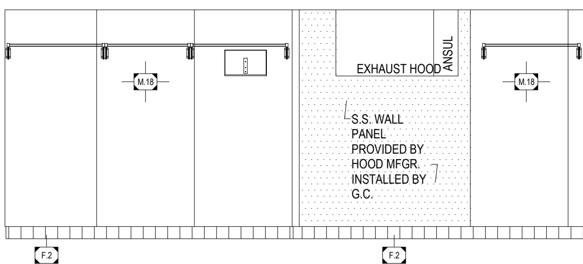
20 INTERIOR ELEVATION Scale is 1/4" = 1'-0" when printed full size.
