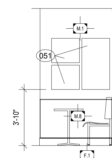
9 INTERIOR ELEVATION Scale is 1/4" = 1'-0" when printed full size.
