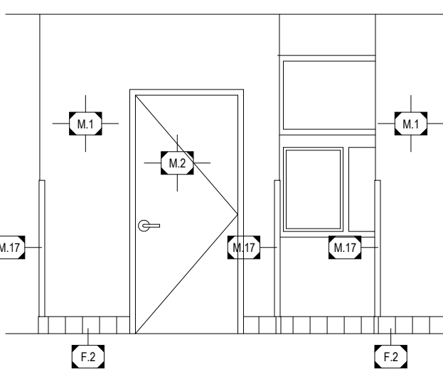
24 INTERIOR ELEVATION Scale is 1/4" = 1'-0" when printed full size.
