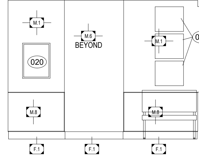
5 INTERIOR ELEVATION Scale is 1/4" = 1'-0" when printed full size.
