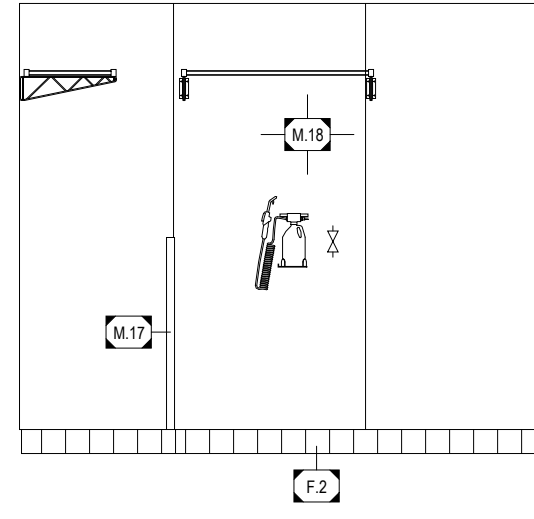
12 INTERIOR ELEVATION Scale is 1/4" = 1'-0" when printed full size.
