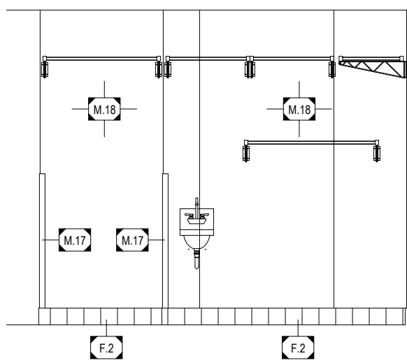
19 INTERIOR ELEVATION Scale is 1/4" = 1'-0" when printed full size.
