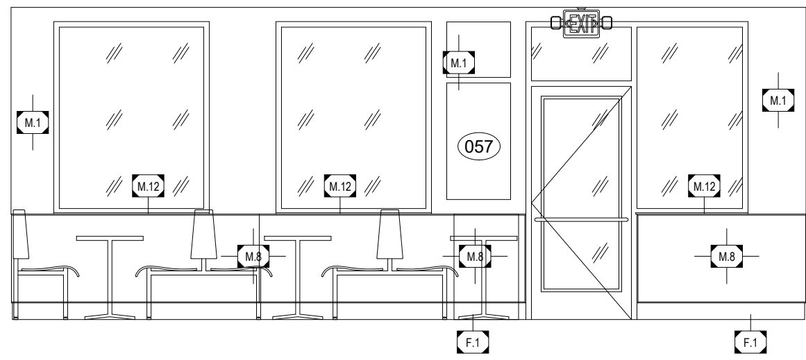
1 INTERIOR ELEVATION Scale is 1/4" = 1'-0" when printed full size.
