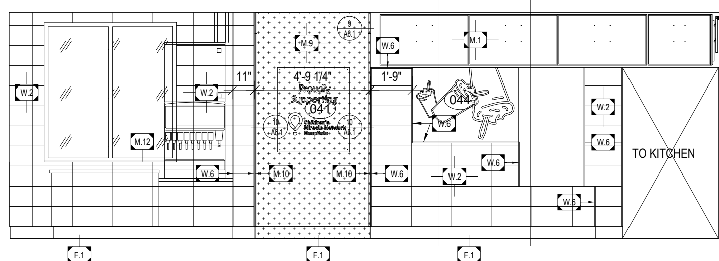
2 INTERIOR ELEVATION Scale is 1/4" = 1'-0" when printed full size.
