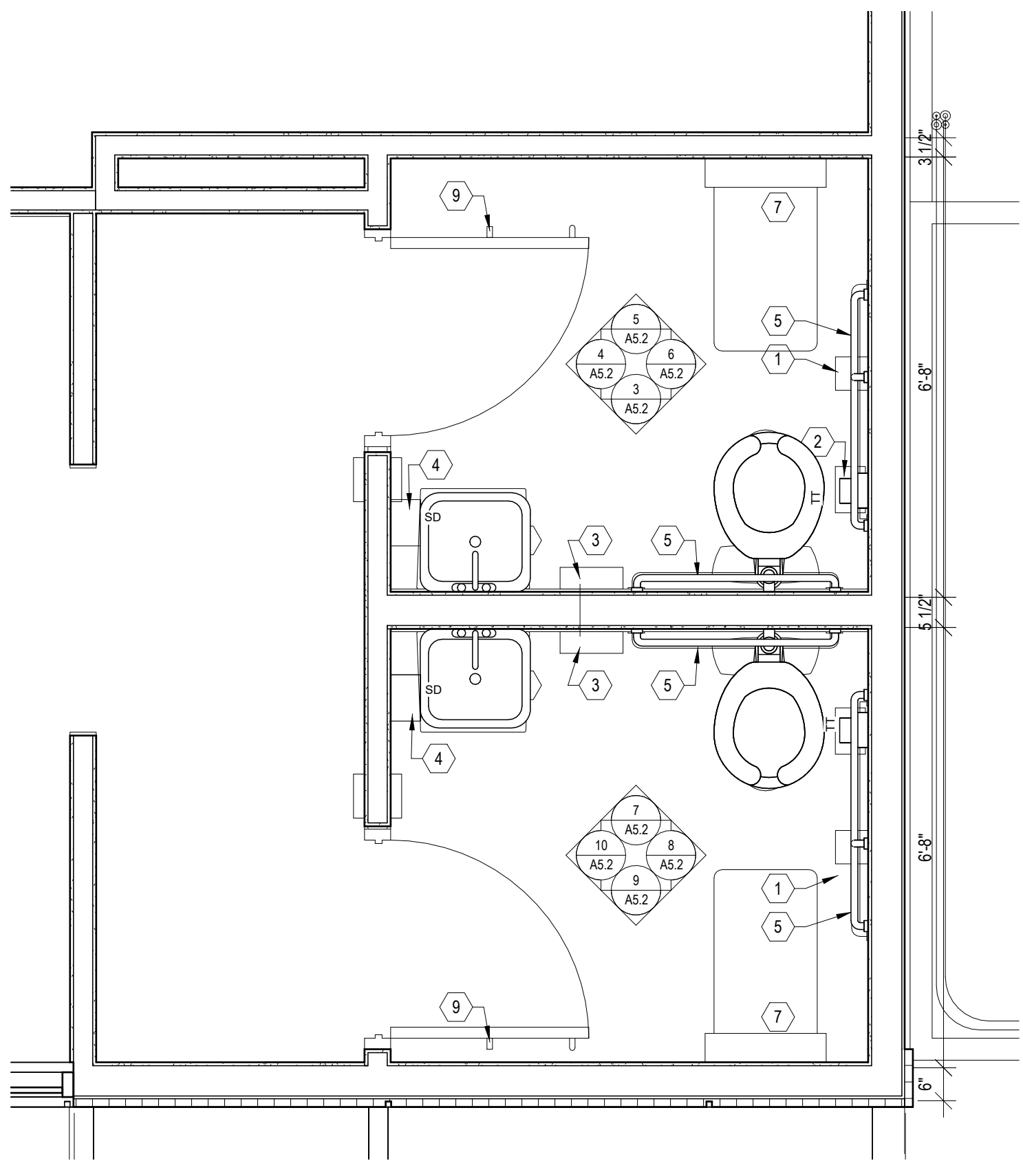
RESTROOM FLOOR PLAN
