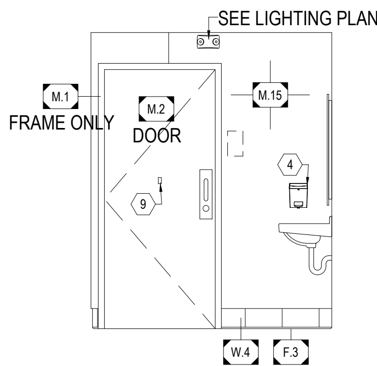
10 RESTROOM ELEVATION
