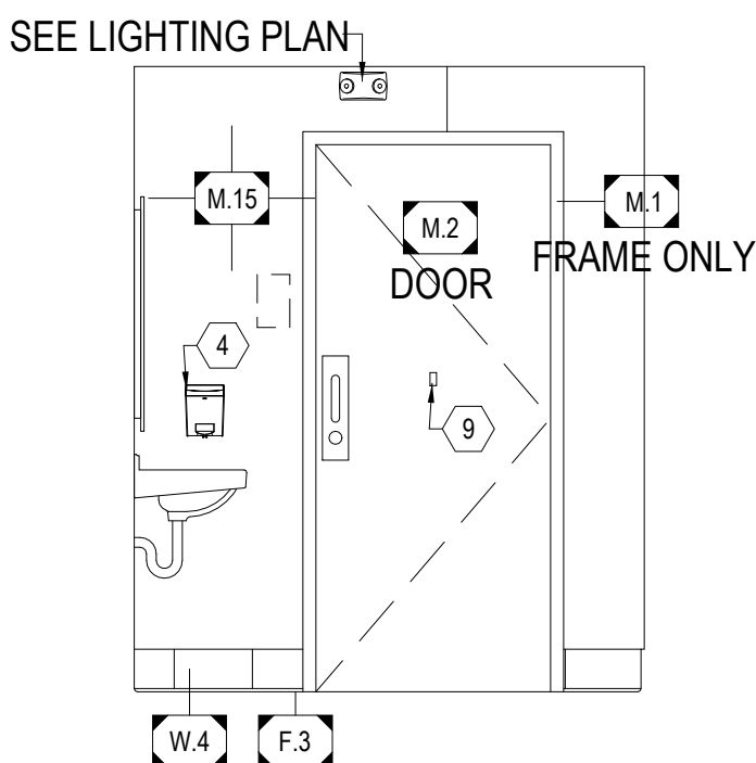
4 RESTROOM ELEVATION
