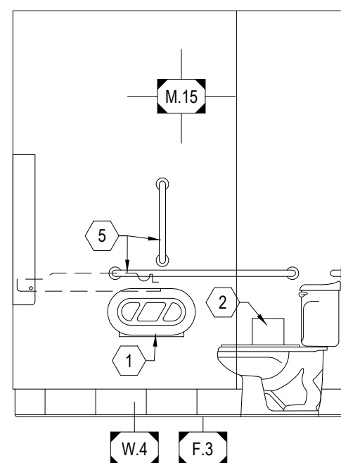
6 RESTROOM ELEVATION
