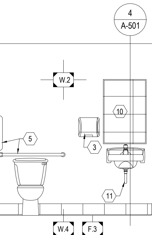
3 RESTROOM ELEVATION
