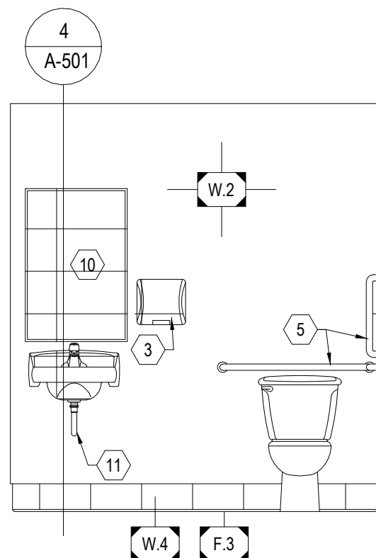
7 RESTROOM ELEVATION
