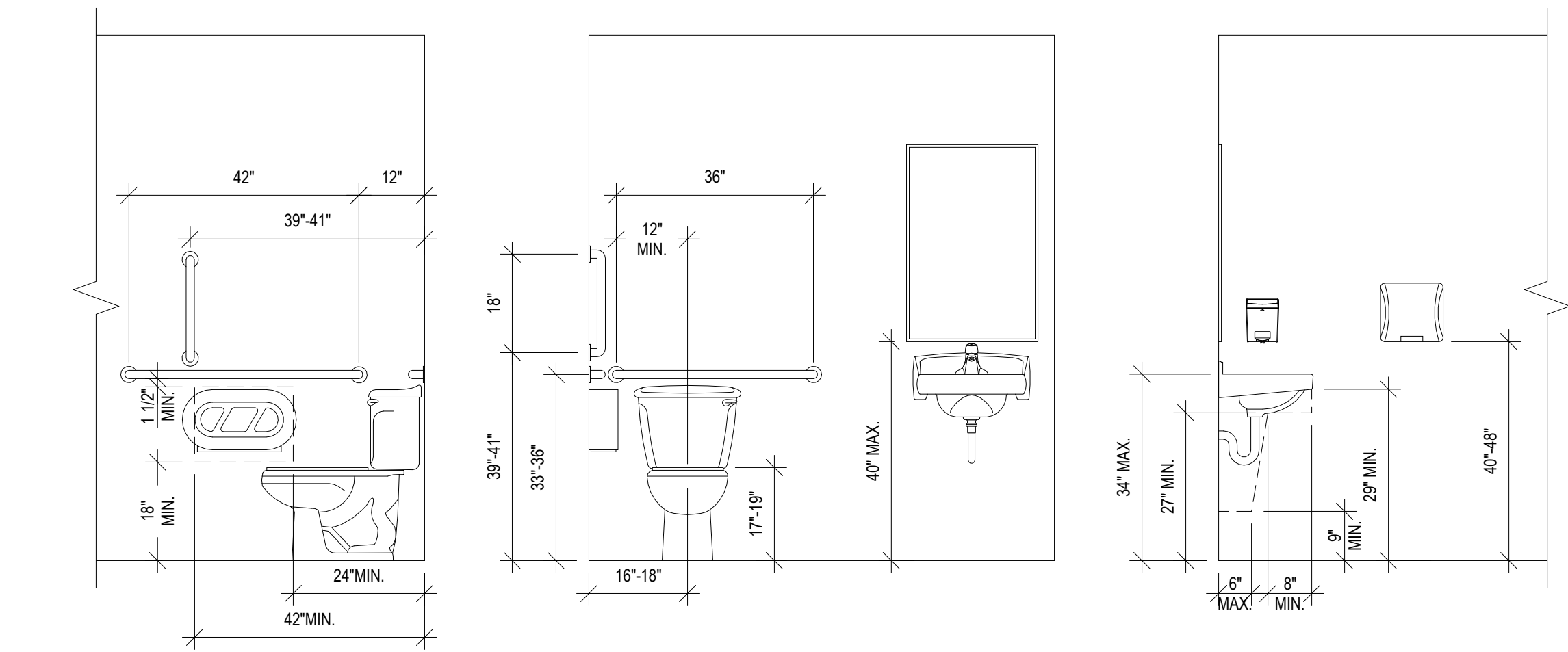
2 ADA Mounting Heights
