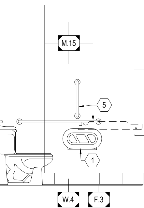
8 RESTROOM ELEVATION
