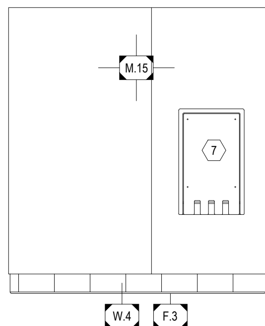
5 RESTROOM ELEVATION
