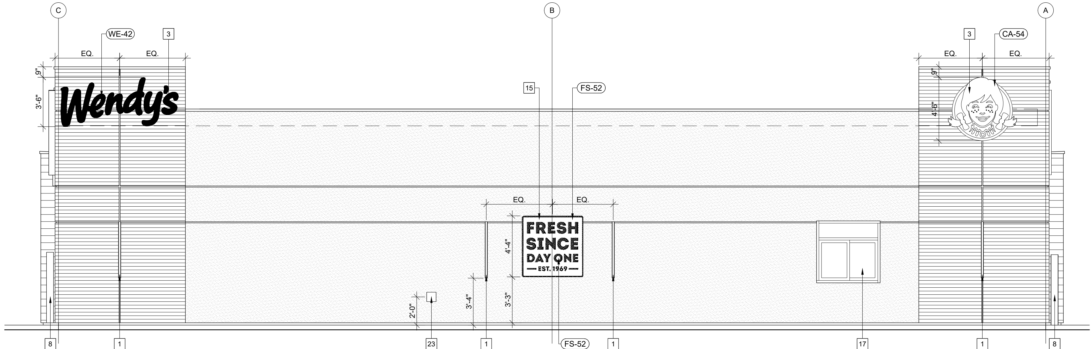
03 DRIVE-THRU SIDE ELEVATION
