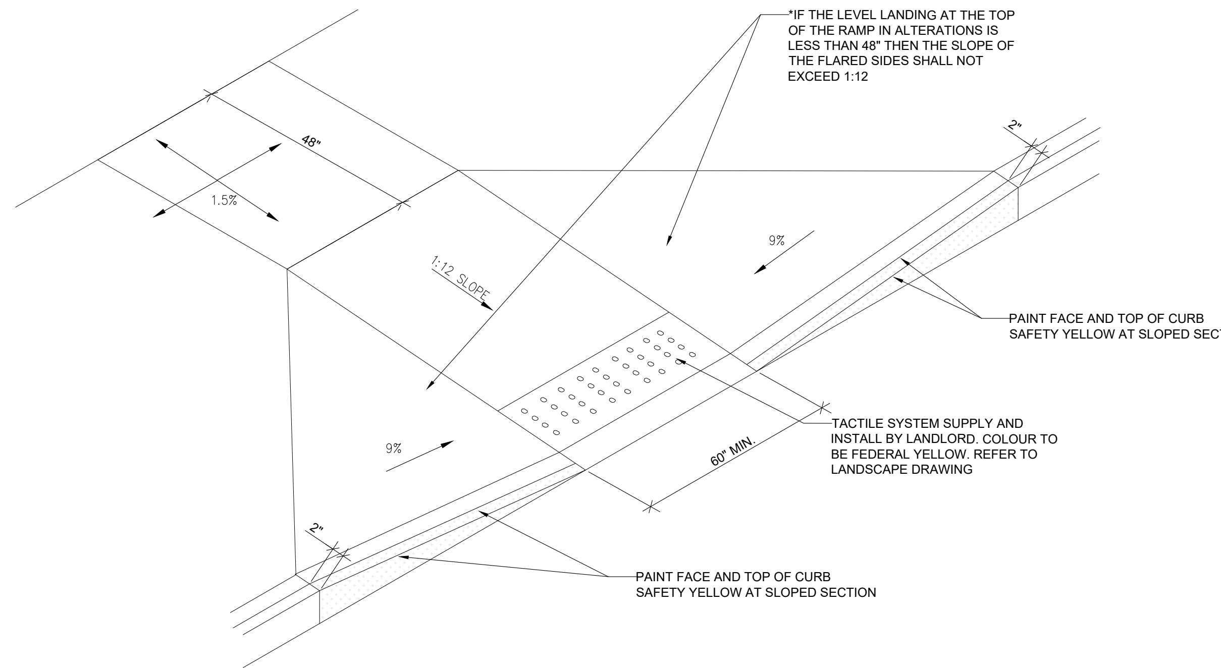
04 CURB RAMP DETAIL
