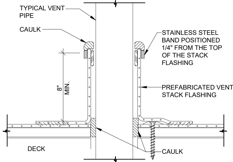
05 ROOF DETAIL - TYPICAL PIPE SCALE: 1 1/2" = 1'-0"
