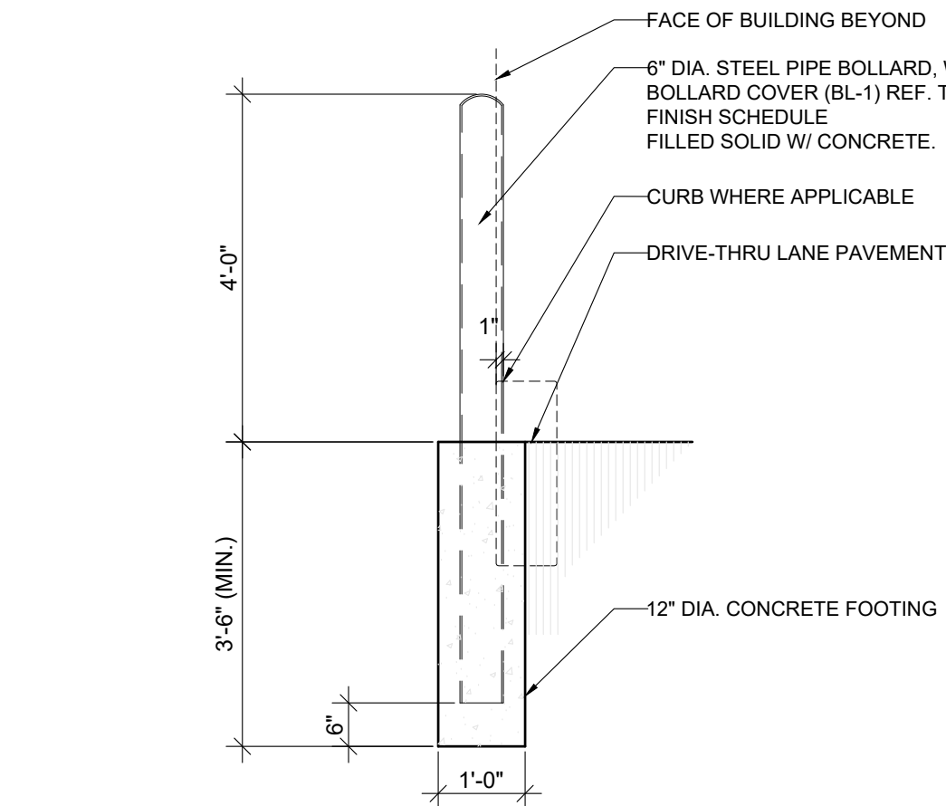
03 6" BOLLARD DETAIL
