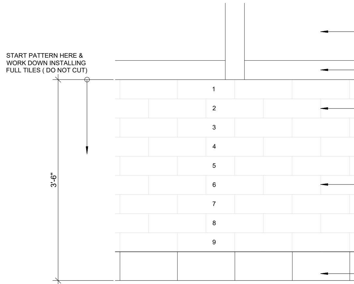
02 WT-13 WALL PATTERN DETAIL SCALE: 1" = 1'-0"
