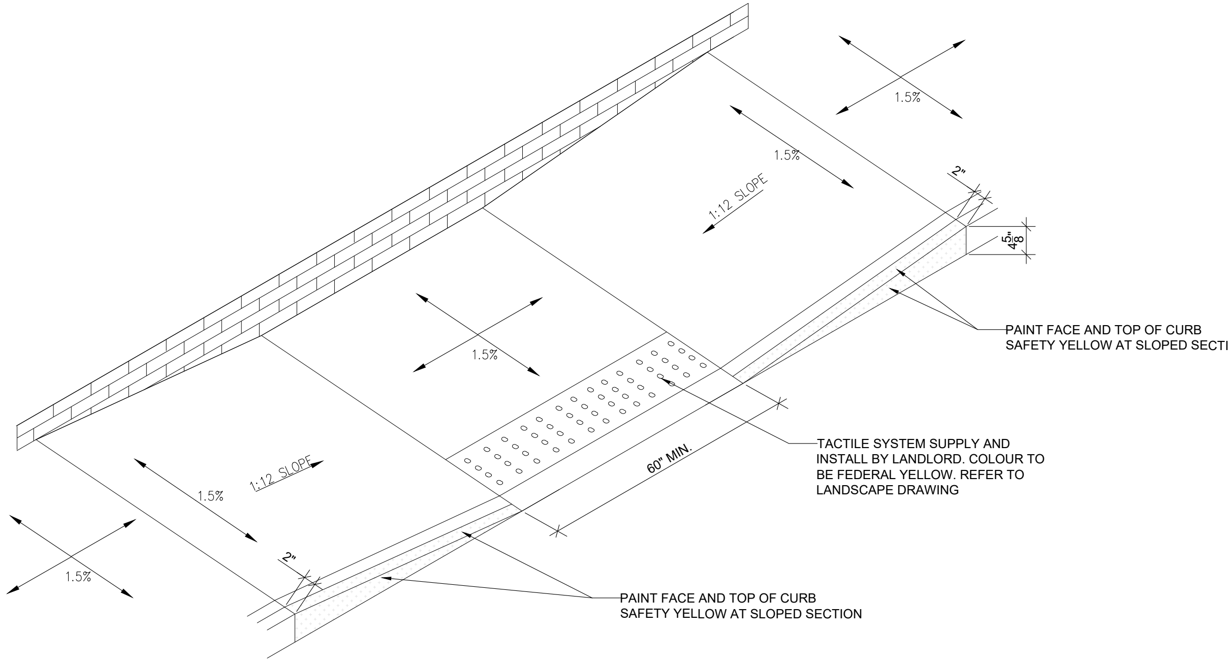
02 PAVEMENT MARKER DETAIL
