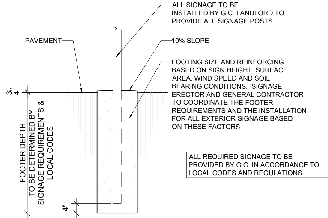
06 SIGN BASE DETAIL
