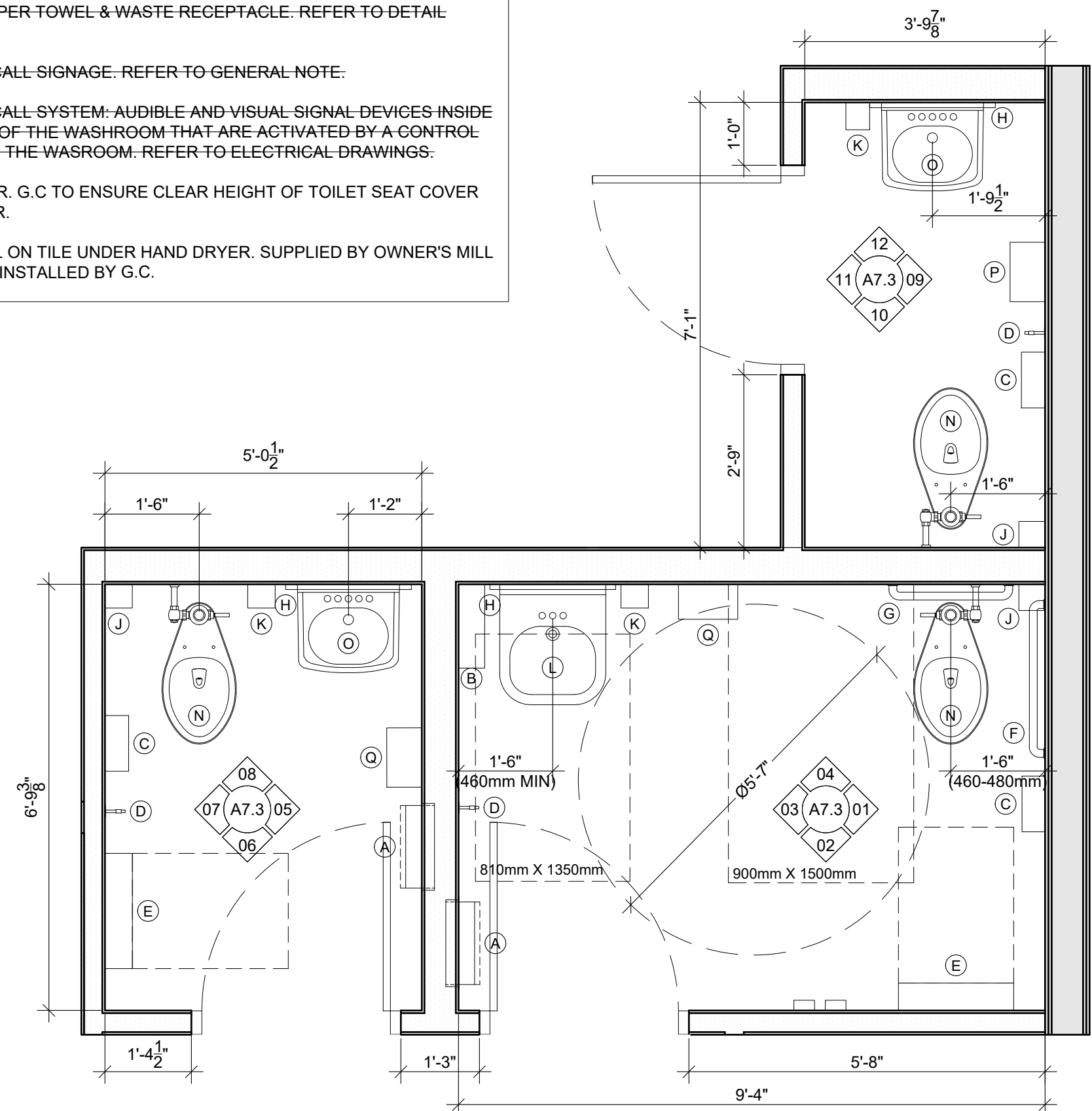
A ENLARGED WASHROOM PLAN SCALE: 1/2" = 1'-0"
