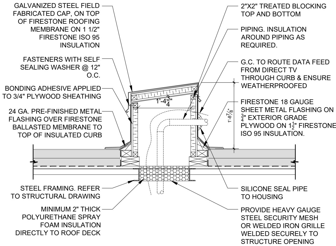
02 ROOF DETAIL - CONDENSER PIPE (A) SCALE: 3/4" = 1'-0"
