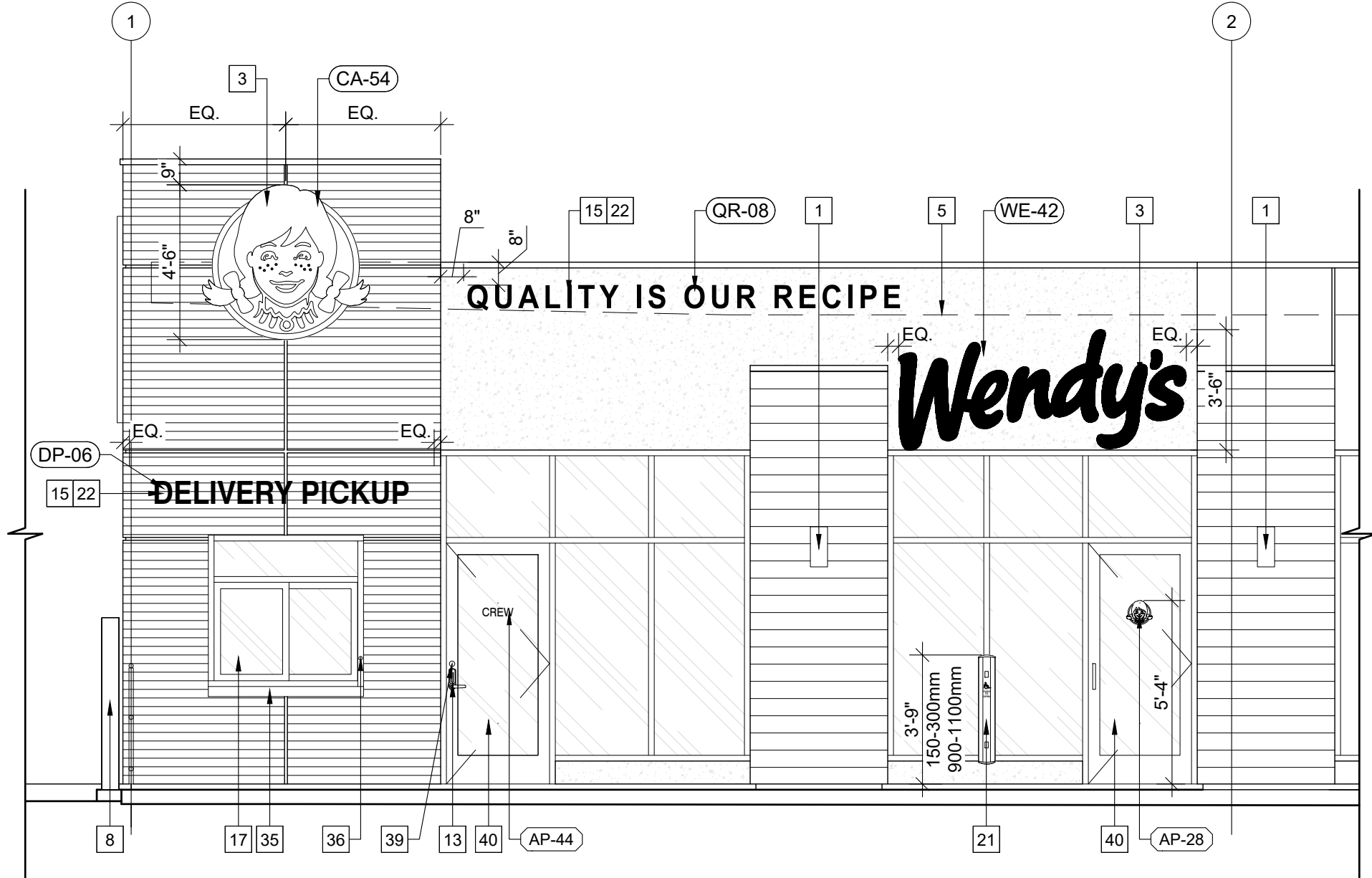
01 ENTRANCE SIDE ELEVATION
