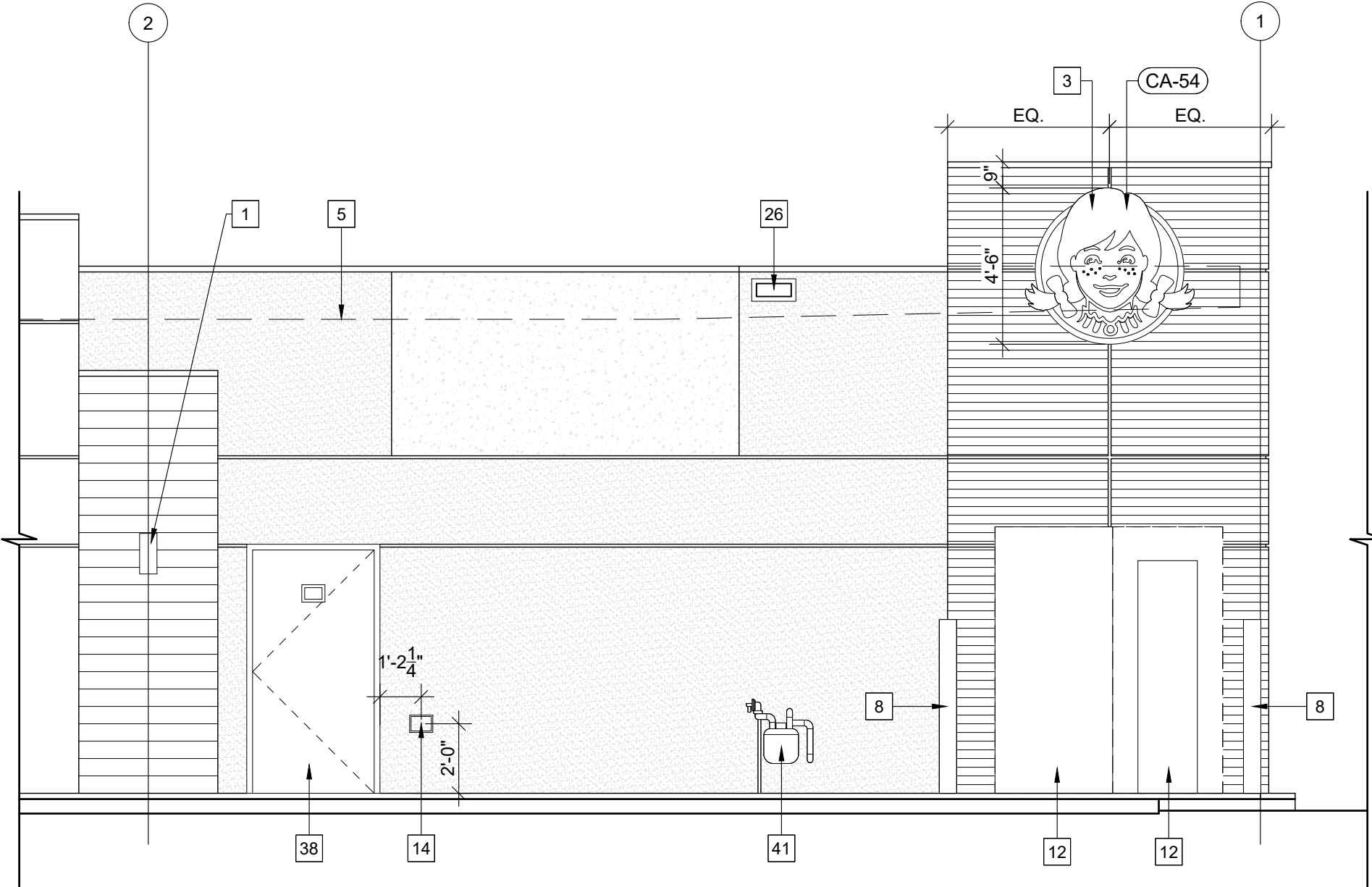
02 REAR ELEVATION
