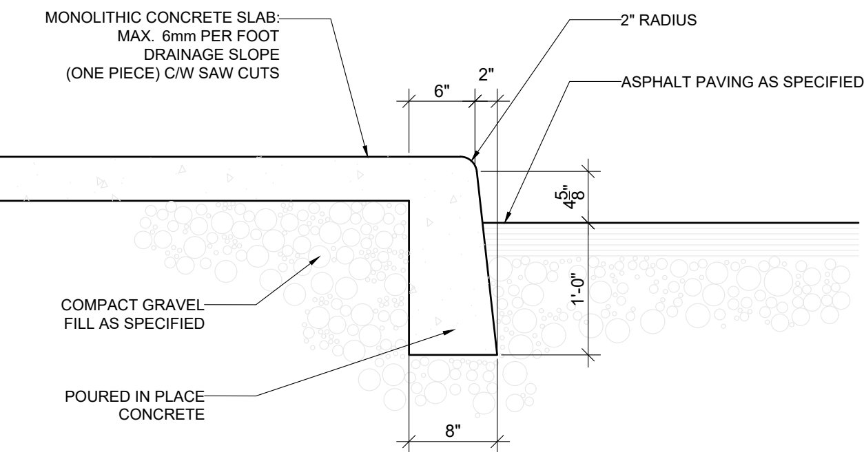
01 CONCRETE CURB DETAIL
