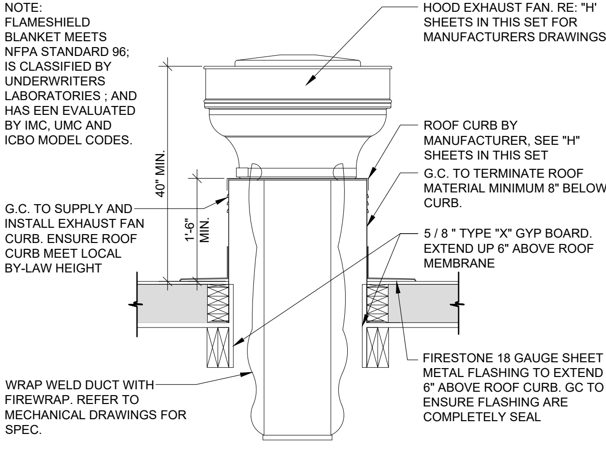
03 EXHAUST FAN DETAIL SCALE: 3/4" = 1'-0"
