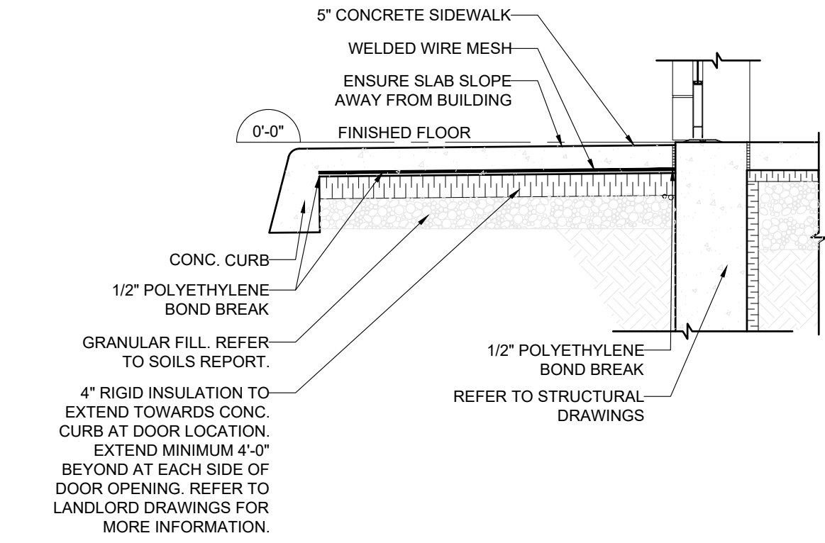
07 FROST SLAB DETAIL
