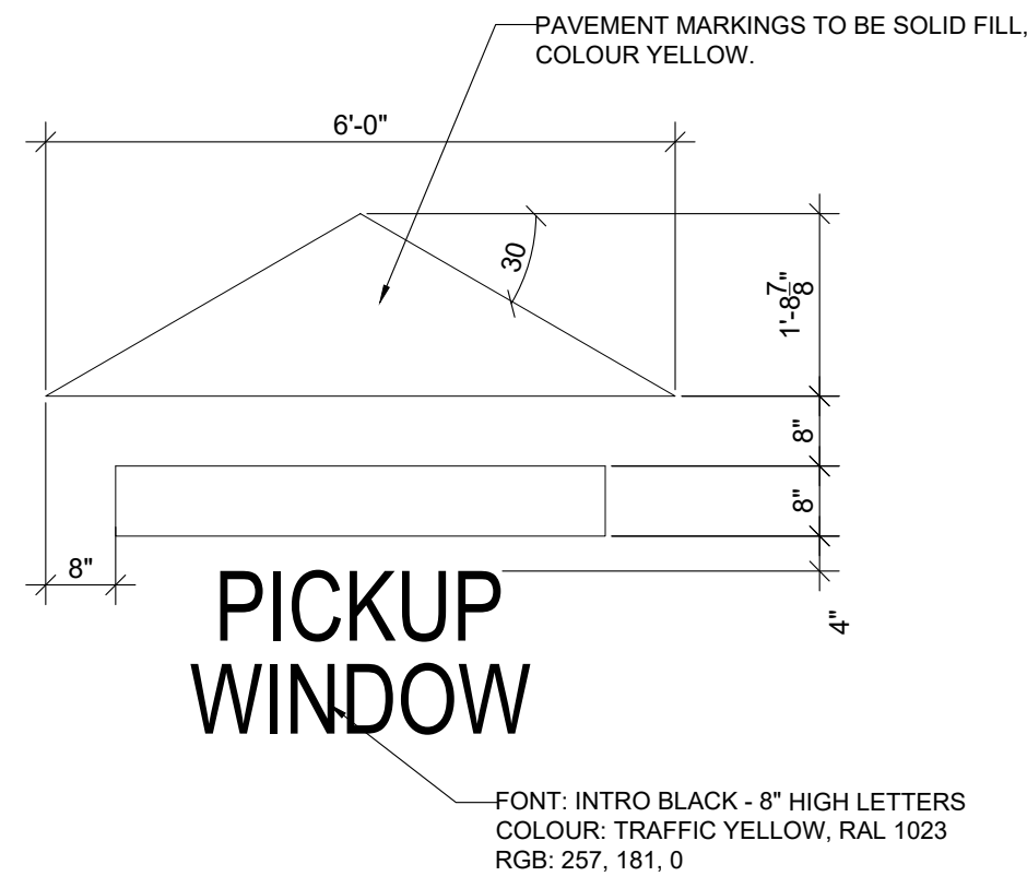
02 PAVEMENT MARKER DETAIL
