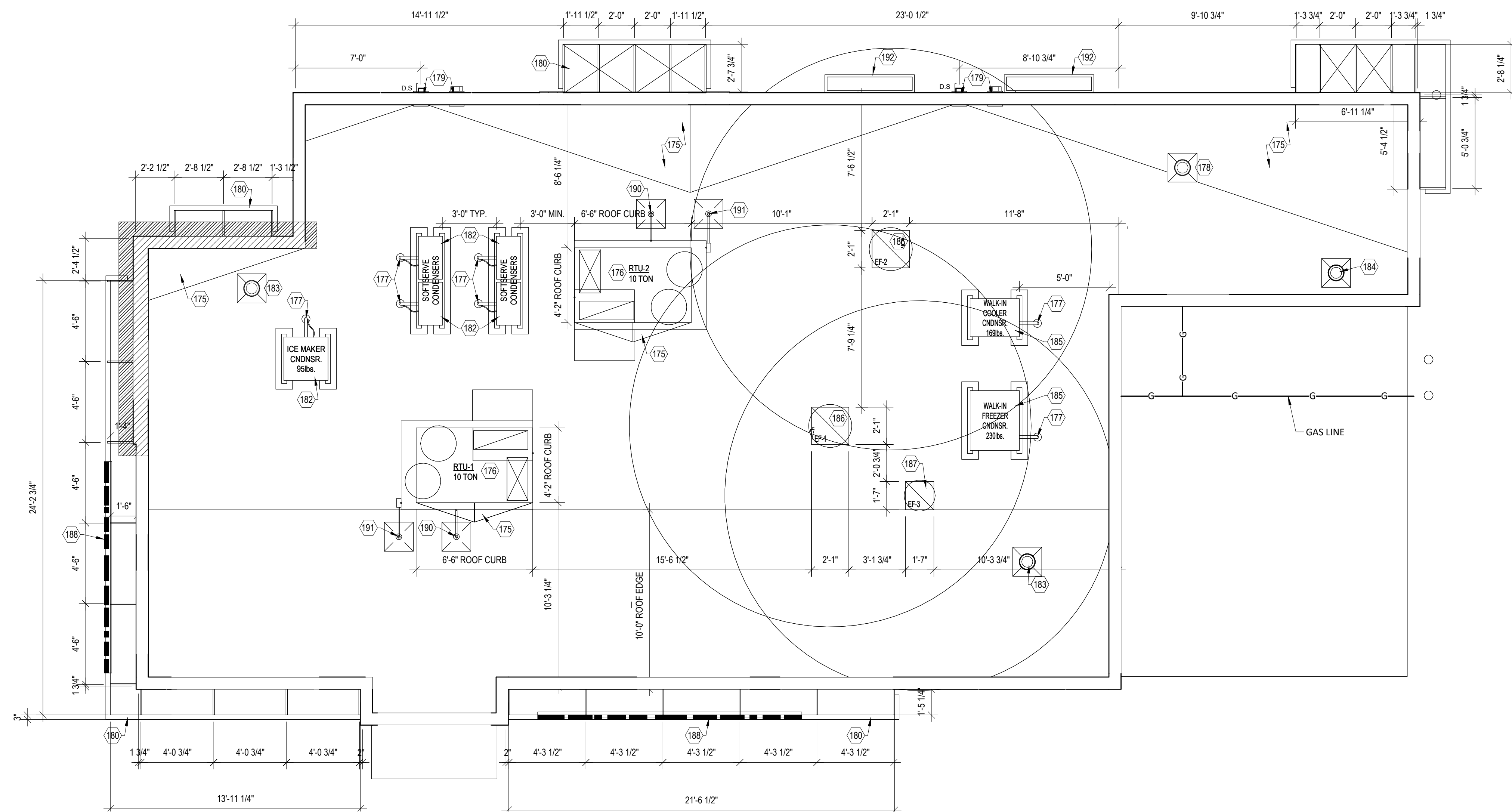
ROOF PLAN
