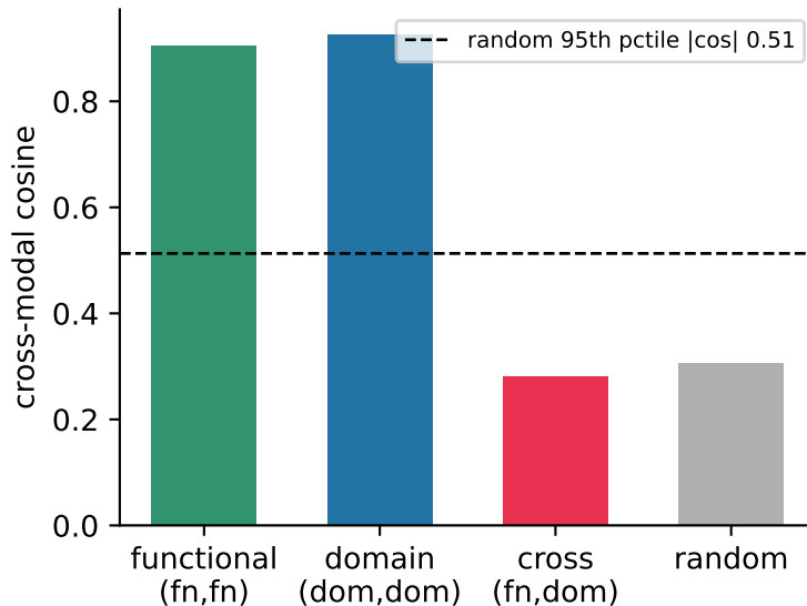
(b) Shared functional axis
