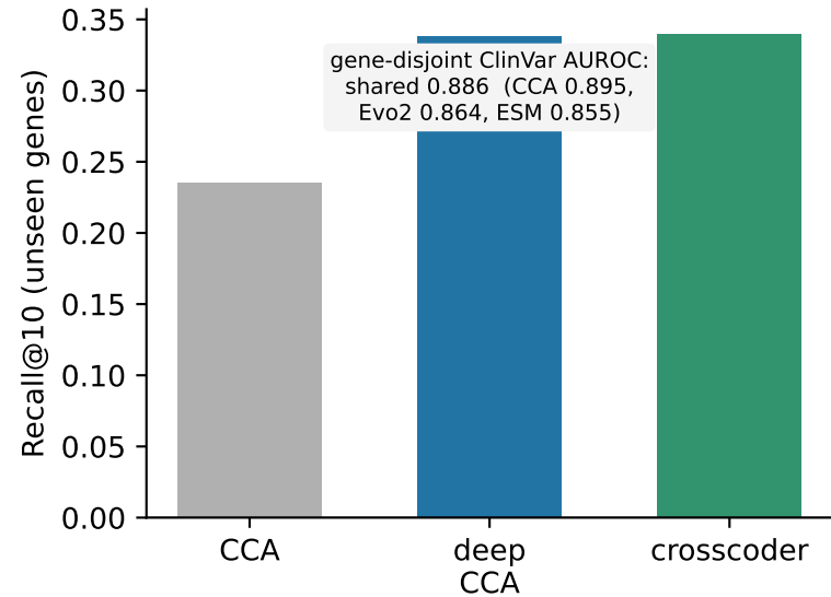
(a) Cross-gene retrieval (15 genes)
