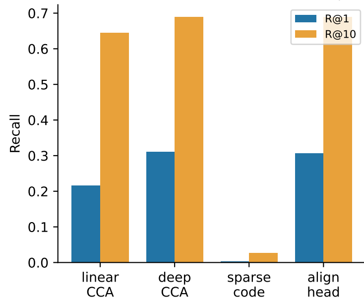
(a) Cross-modal retrieval (residue-disjoint)
