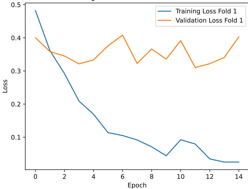
Training and Validation Loss for Fold 1
