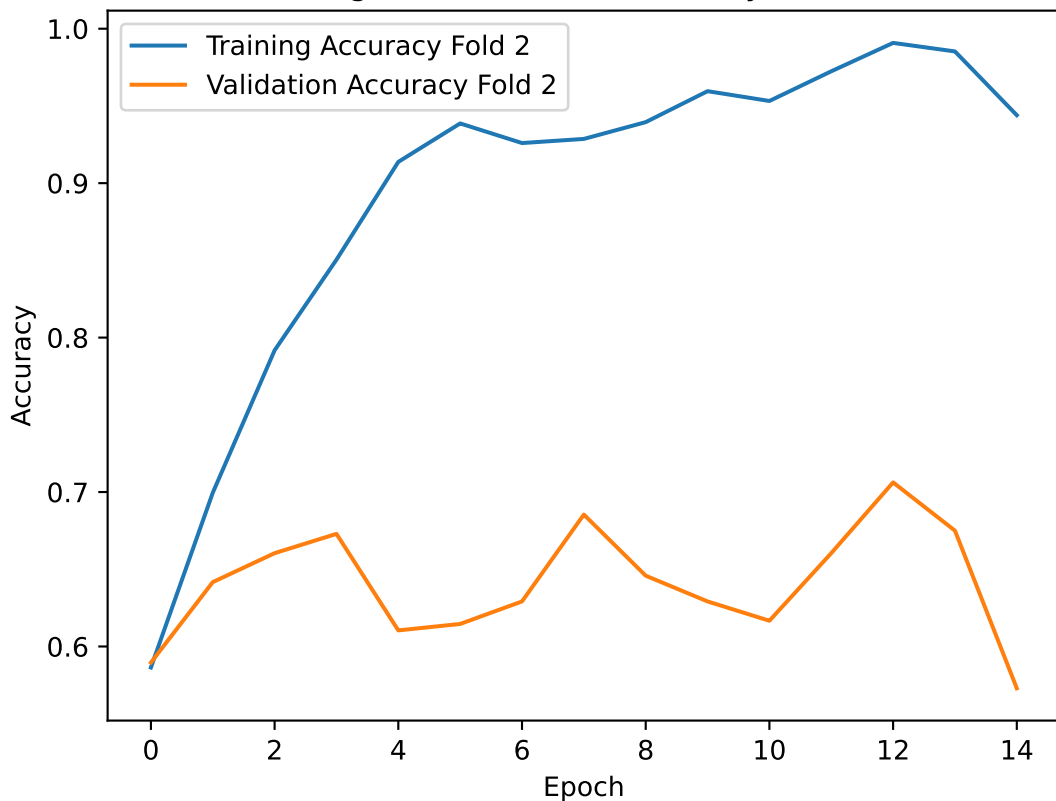
Training and Validation Accuracy for Fold 2
