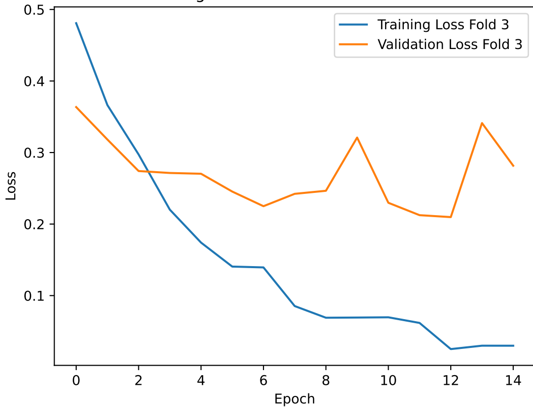
Training and Validation Loss for Fold 3
