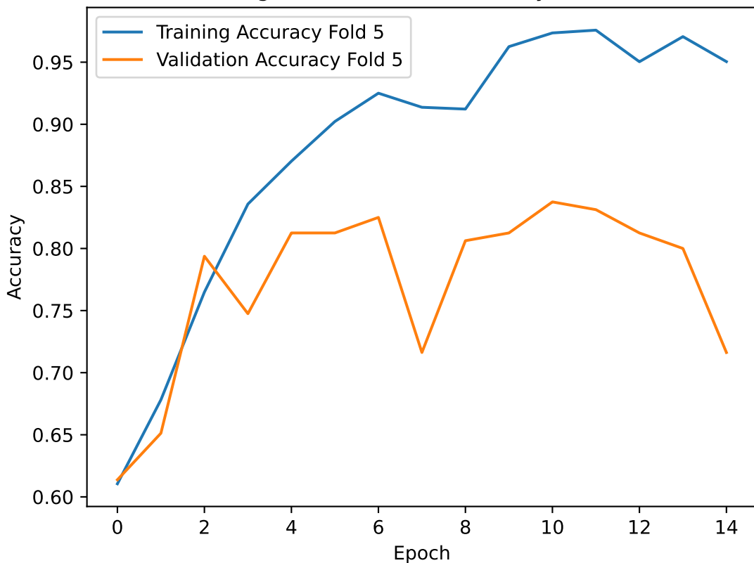
Training and Validation Accuracy for Fold 5
