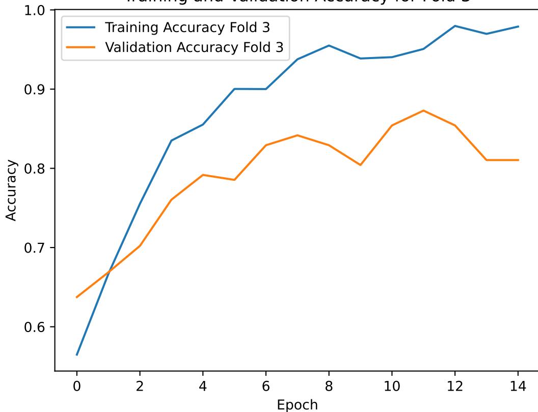
Training and Validation Accuracy for Fold 3
