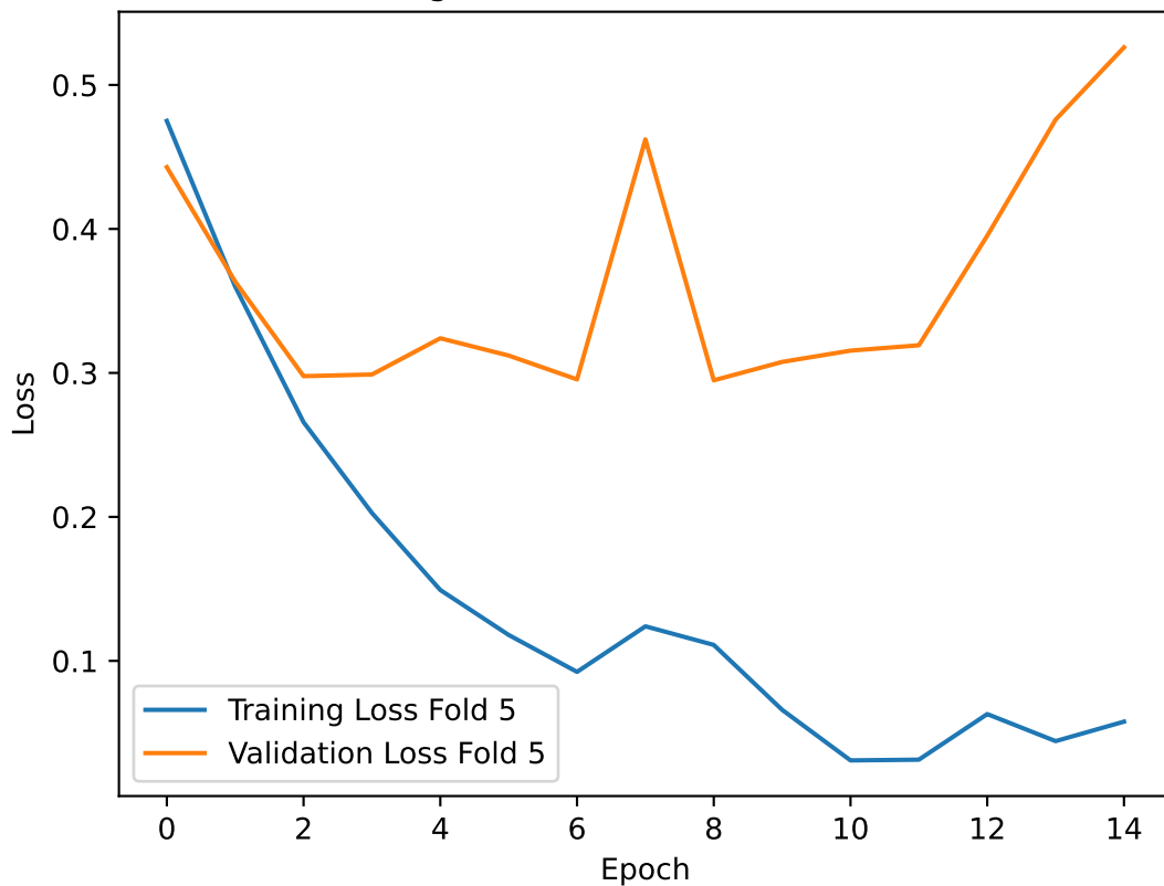
Training and Validation Loss for Fold 5
