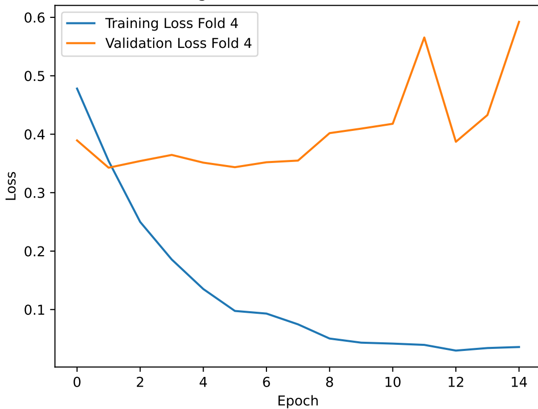
Training and Validation Loss for Fold 4
