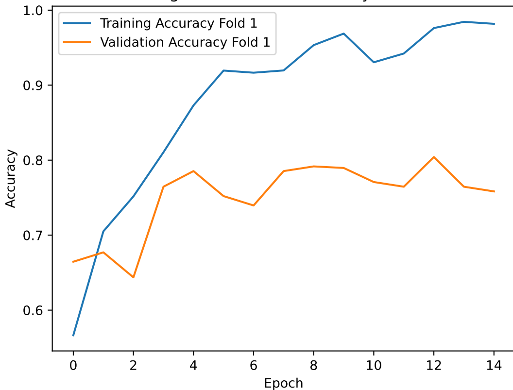
Training and Validation Accuracy for Fold 1
