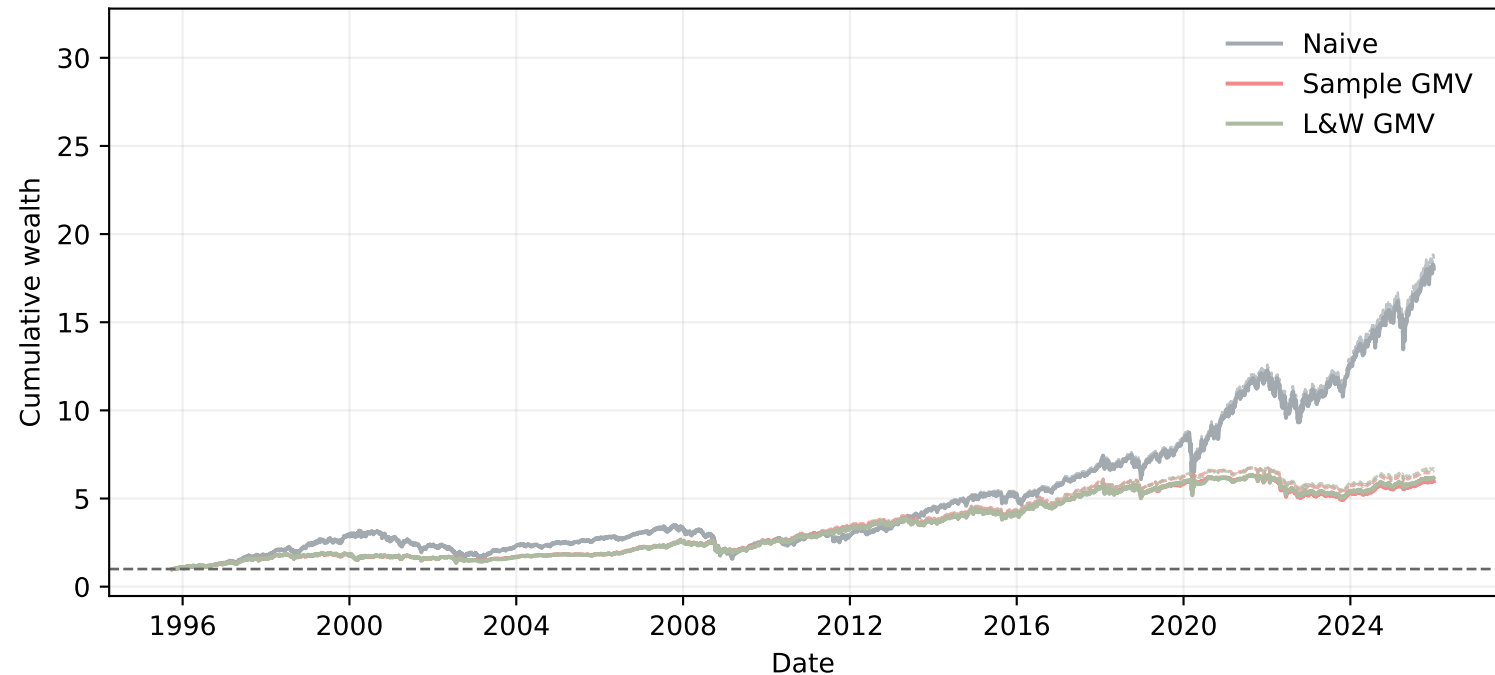
Cumulative Wealth - N = 100
