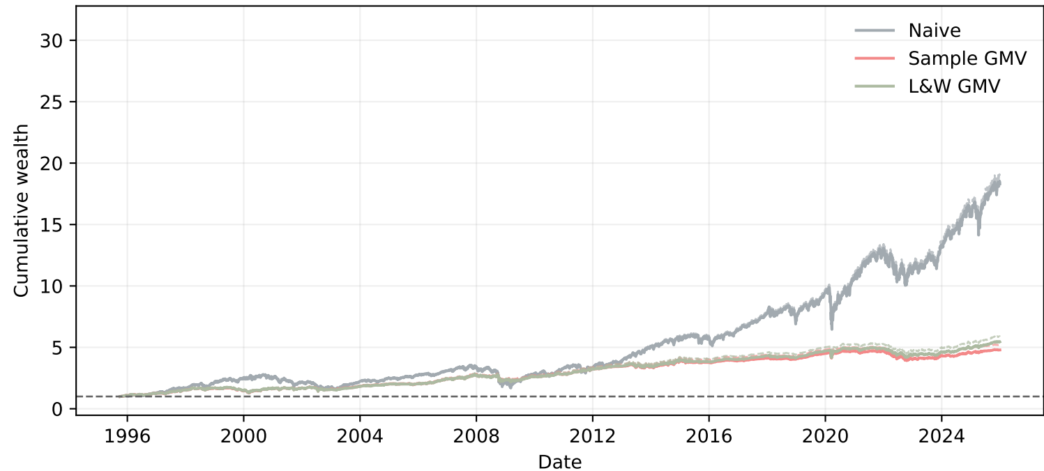
Cumulative Wealth - N = 200
