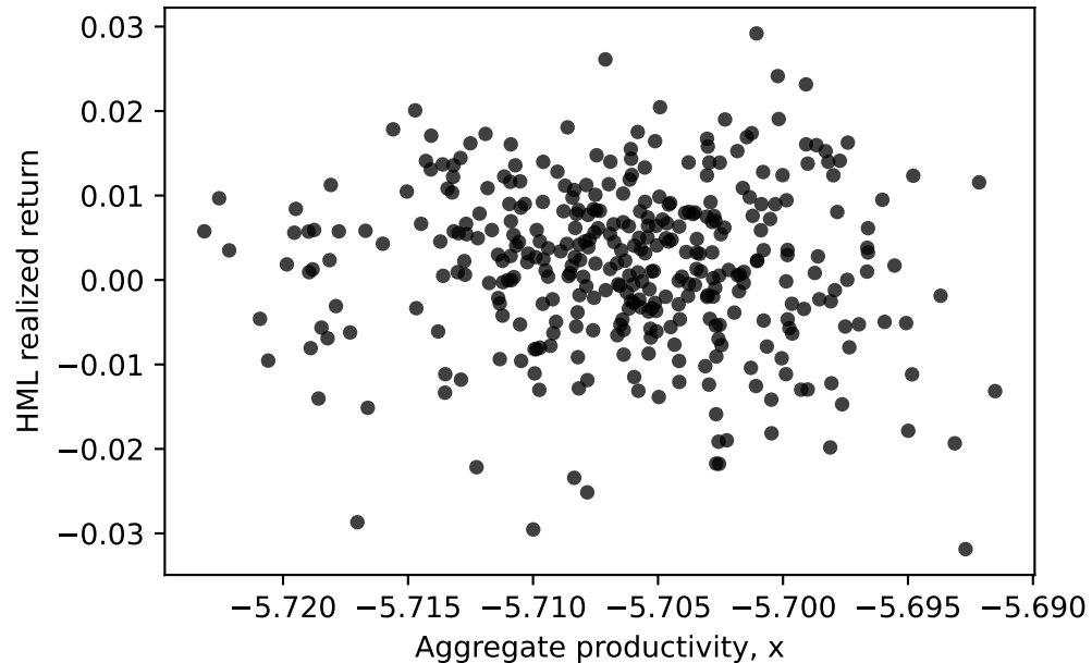
Panel A: Simulated HML
