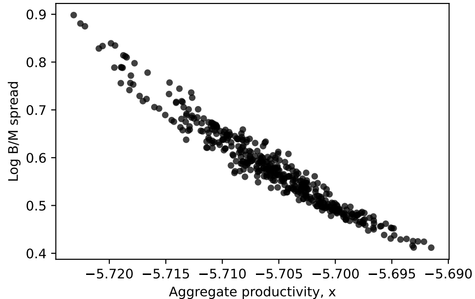
Panel B: Value Spread
