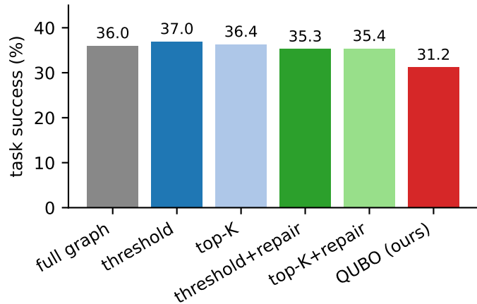
Binding budget (0.75 x full-graph cost, fully constrained)
